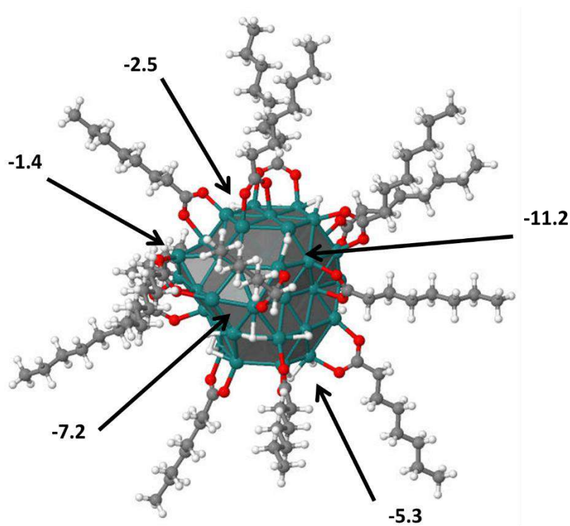
Figure 3.50 \Delta G_H (kcal.mol -1 ), arrows indicate the adsorption sites of \text{Ru}_{55}(\text{C}_7\text{H}_{15}\text{COO})_{14}(\text{H})_{14} NP.
