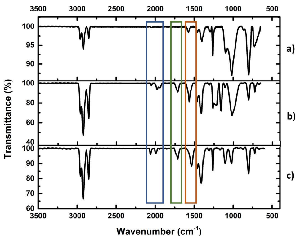
Figure 3.29 Experimental FTIR spectra: (a) (\text{Ru}_x(\text{C}_7\text{H}_{15}\text{COOH})_{0.15})_{\text{THF}} ; (b) (\text{Ru}_x(\text{C}_7\text{H}_{15}\text{COOH})_{0.30})_{\text{THF}} ; (c) (\text{Ru}_x(\text{C}_7\text{H}_{15}\text{COOH})_{0.40})_{\text{THF}} NPs. Three specific vibration regions are highlighted: (blue) \nu(\text{CO}) ; (green) \nu(\text{COOH}) ; (orange) \nu(\text{COO}) .
