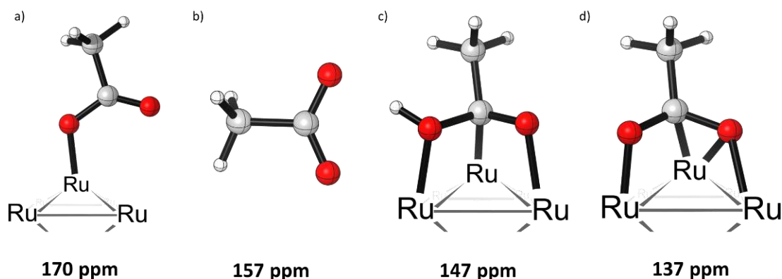
Figure 2.29 Carboxylic carbon DFT chemical shift of the carboxylic moieties free and interacting with [Ru 6 ] nanocluster. Different coordination modes (a) CH 3 COO; η, (c) CH 3 COOH; σ carbon, μ, (d) CH 3 COO; σ carbon, μ 3 & (b) free CH 3 COO.
