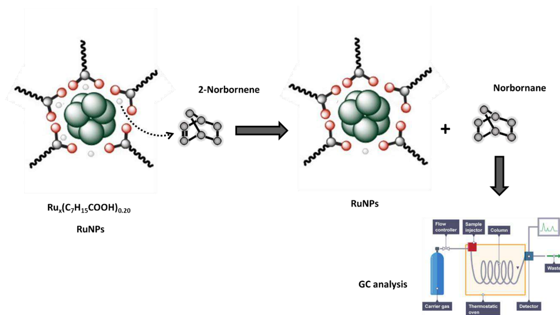
Scheme 3.9 Hydrides titration at the surface of \text{Ru}_x(\text{C}_7\text{H}_{15}\text{COOH})_{0.20} NPs by the norbornene test.
