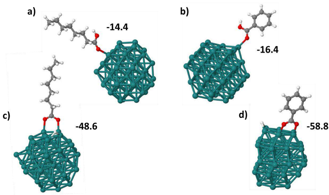
Figure 4.11 Theoretical models representing the interaction of carboxylic moieties with the \text{Ru}_{55} NP over the (001) plane. (a) octanoic acid; (b) benzoic acid; (c) octanoate; (d) benzoate. The E_{ads} ( \text{kcal}\cdot\text{mol}^{-1} ) are also presented.
