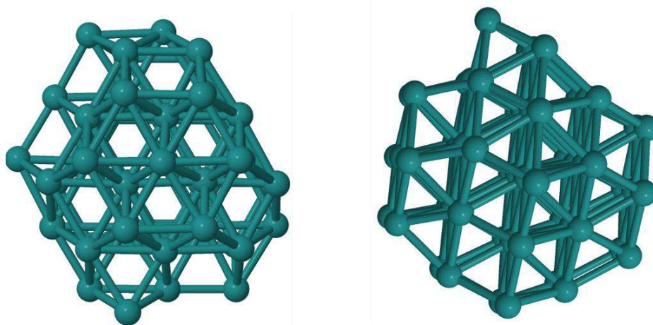
Figure 6.4 Ultra-small Ru 55 model.
