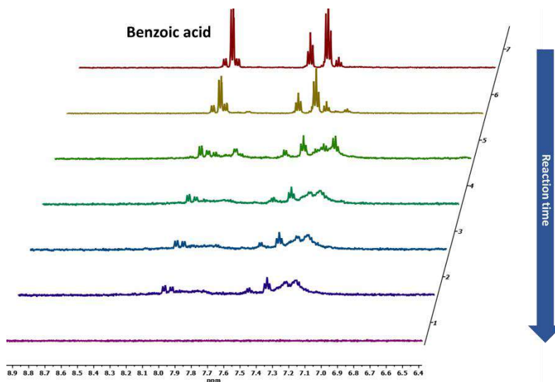
Figure 4.4 Zoom of the aromatic region of the ^1\text{H-NMR} ( \text{THF-}d^8 ) spectra provided in figure 4.3.
