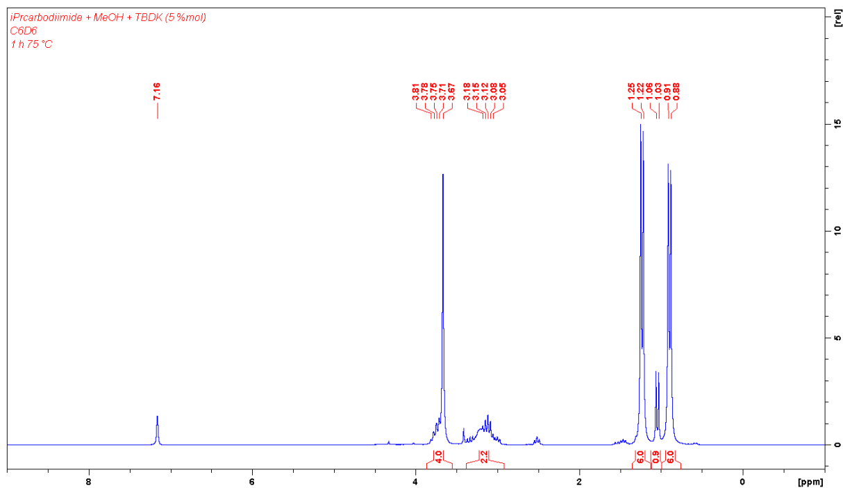
Figure VII-76 ^1\text{H} spectrum of crude mixture: formation of N,N' -diisopropyl- O -methylisourea ( 2a ) in \text{C}_6\text{D}_6
