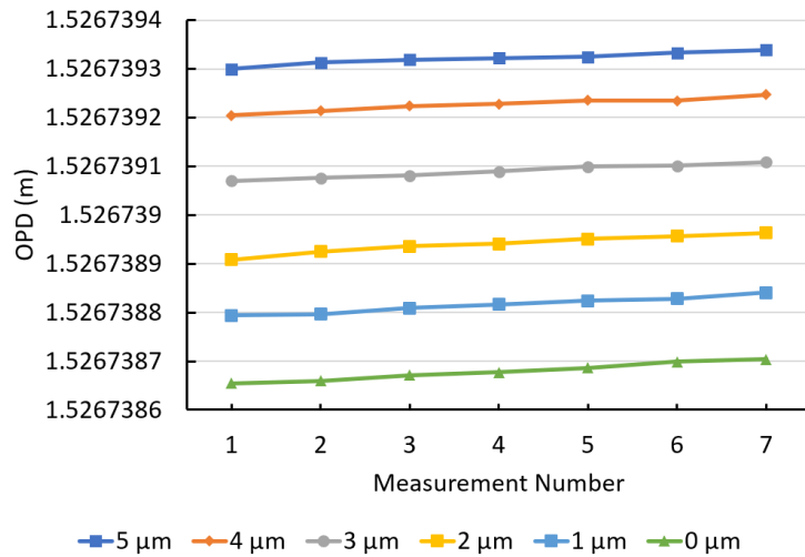
Fig. 5.11. Measurement result using zero-padding to the linearized fringe signal. Xx zeros were added so that the overall digital resolution was 1 μm.
