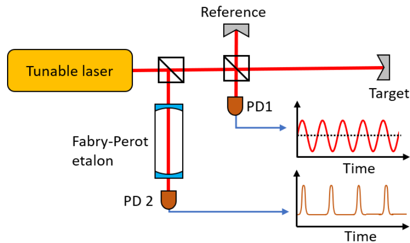
Fig. 1.18. The ADM system setup based on FSI. Adapted from Ref. [44].
