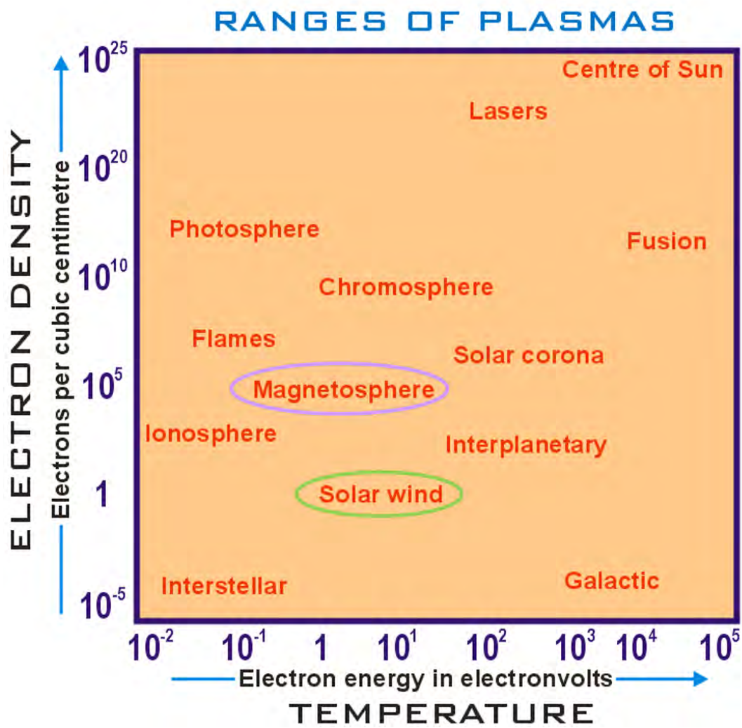
Figure 1.2 – The ranges of temperature and densities of plasmas (1eV ~ 11600K). Figure from Peratt (1996).
