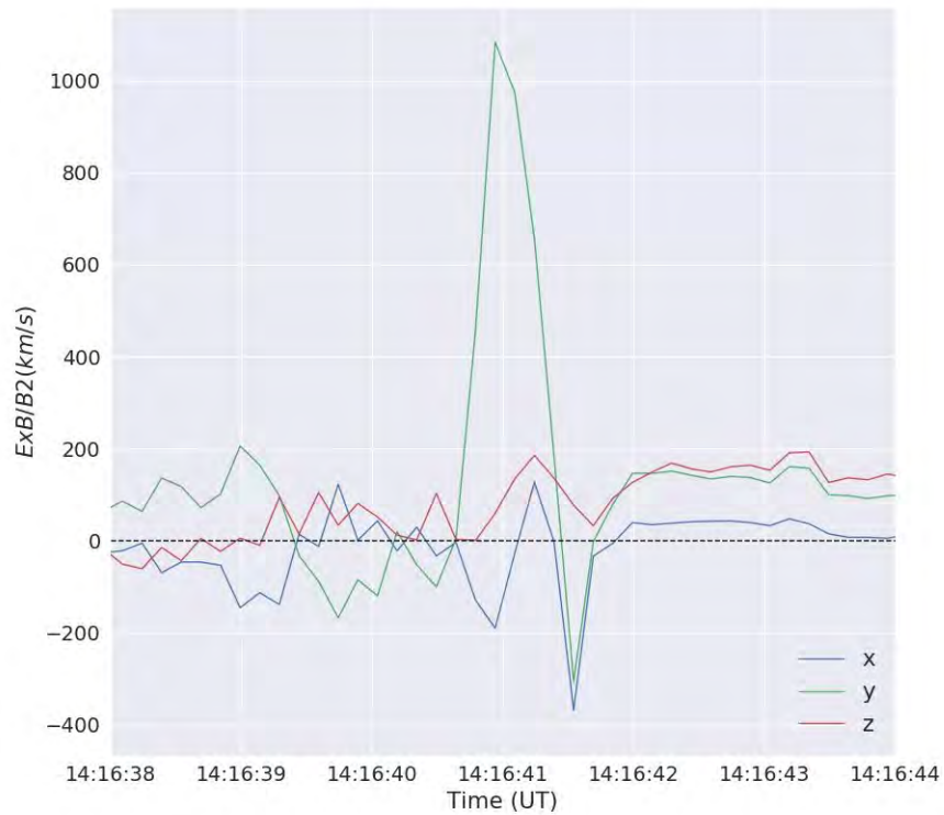
Figure 4.10 – Electric drift speed ( E \times B / B^2 ).
