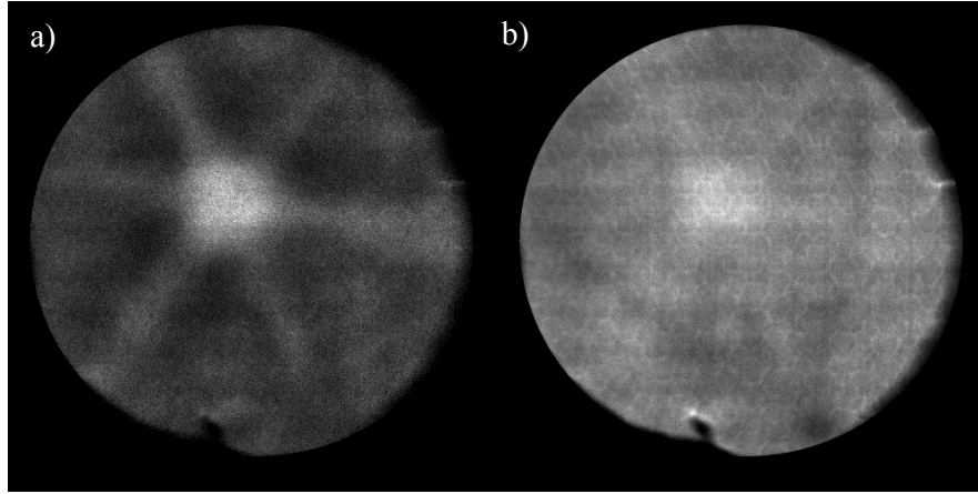
Figure 3-17. Desorption map from APT of the Fe-35Cr, 235MPa, \langle 111 \rangle -grain, a) from multiple event map, b) \langle 111 \rangle pole in the single event map.
