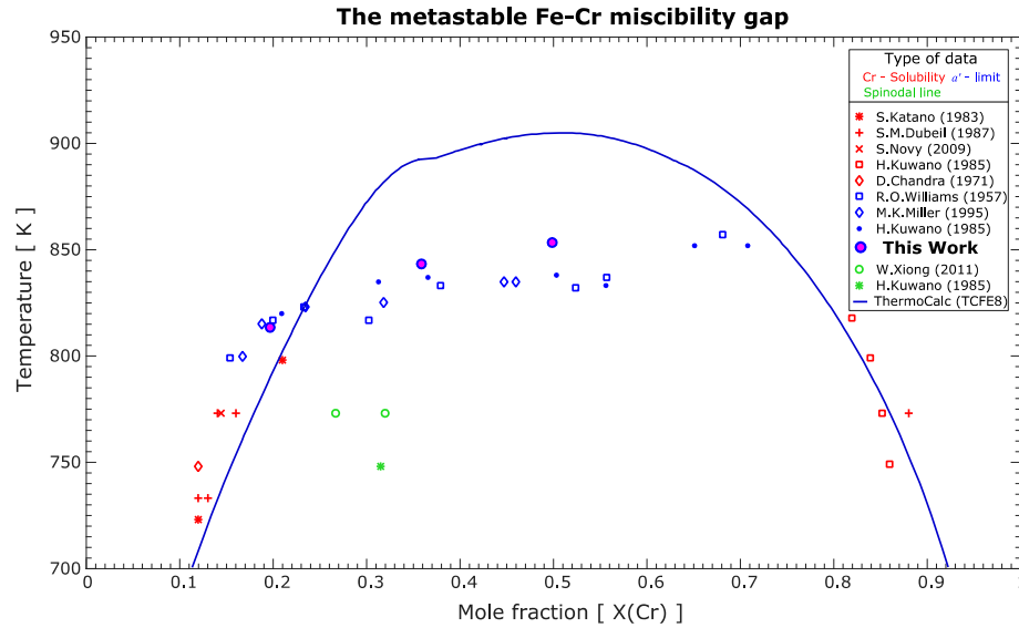
Figure 4-19. A comparison between the metastable MG according to CALPHAD, i.e. ThermoCalc TCFE8 database, this work and literature data. Note that the temperature is given in Kelvin as it is the standardized unit when working with CALPHAD.
