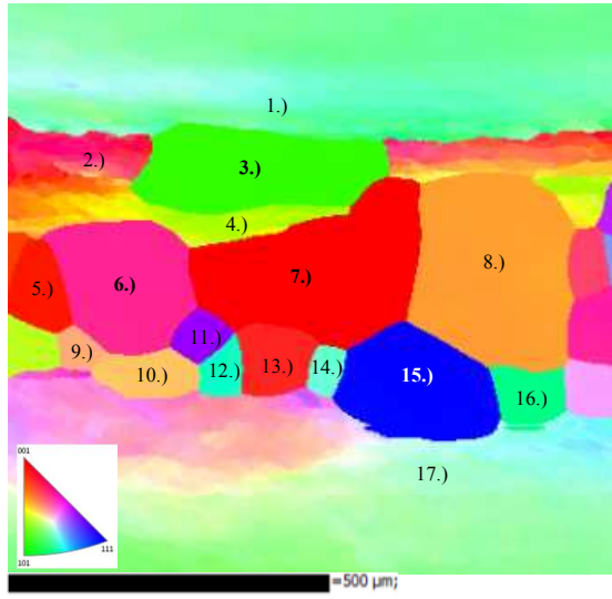
Figure 5-11. EBSD IPF Z Fe-35Cr 525°C 96h 235MPa step size 2.26μm.
