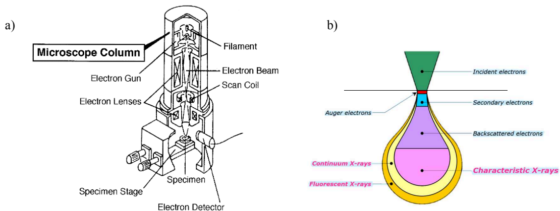
Figure 3-4. a) Schematics of a scanning electron microscope [97], and b) beam - matter interaction [98].
