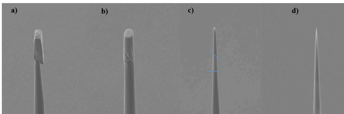
Figure 3-15. a) Chunk of <001> stress-aged sample, b) milled sample with some OP-S on the surface, c) milled sample diameter \sim 300\text{nm} , d) milled sample diameter \sim 80\text{nm} .
