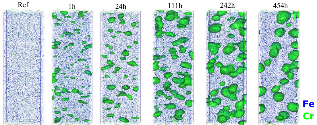
Figure 4-5. Kinetic evolution of the Nb-stabilized Fe-20Cr alloy at 500°C, the extracted volumes are 10x20x60nm and iso -surface threshold was set to 25at. %Cr.
