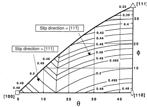
Figure 5-3. Schmid factor dependency of [111]-direction in the [001], [110] and [111] bcc planes by Euler angles [208].
