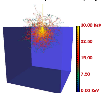
Figure 3-5. CASINO simulation of 30keV implantation depth in Fe-50Cr material, volume 5x5x5 \mu\text{m} .
