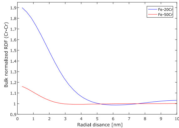
Figure 4-15. RDF of Fe-20Cr and Fe-50Cr at 525°C for 23 days. The strength of Cr-Cr affinity is associated to the width and height of the RDF. Thus (Cr - Cr)_{max}^{20Cr} = 1.90 , the distance to the 2 nd RDF maxima R_2^{20Cr} = 9.70nm , (Cr - Cr)_{max}^{50Cr} = 1.16 and R_2^{20Cr} = 6.47nm .
