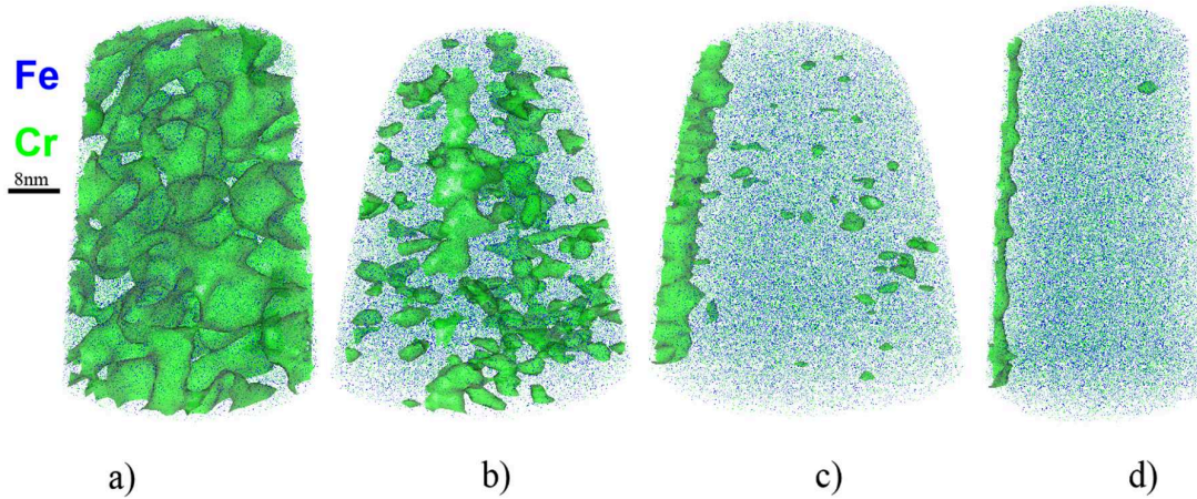
Figure 4-10. APT results of the Fe-50Cr alloys aged 120h, iso surface threshold is set at 60at.-%-Cr. Displaying: a) an interconnected structure (SD) at 565°C, b) high-density Cr fluctuations at 570°C, c) dispersed Cr fluctuations at 578°C and d) stochastic Cr fluctuations at 580°C.
