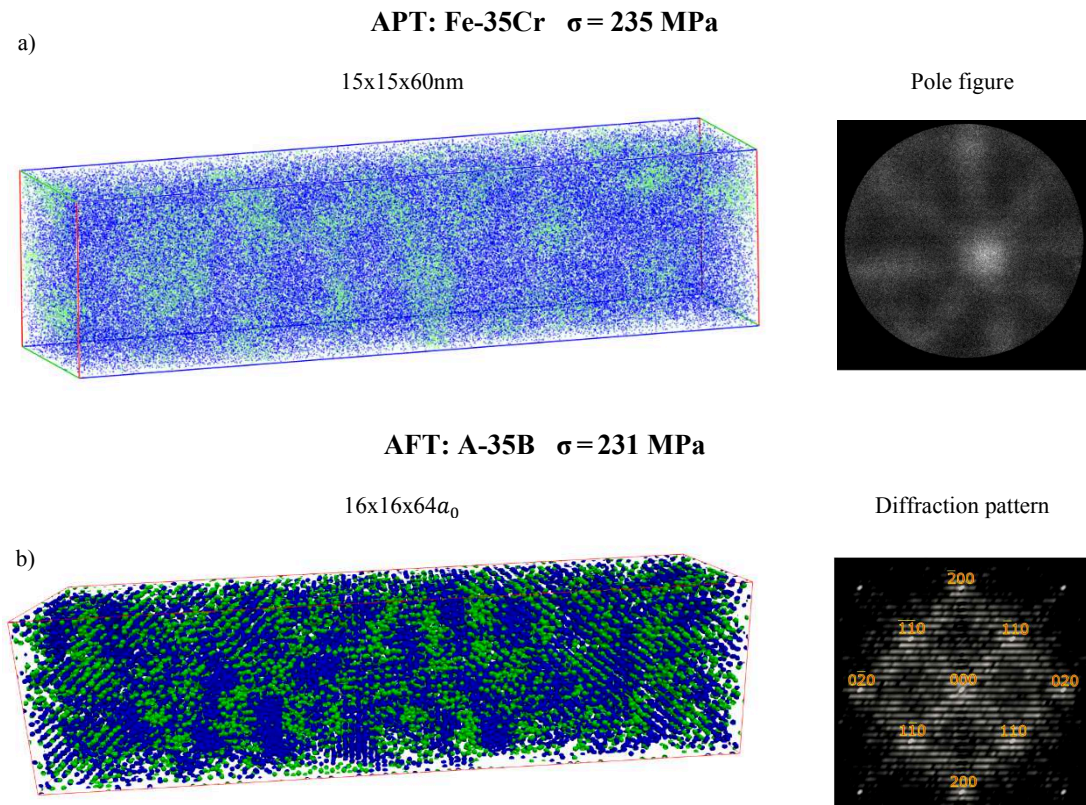
Figure 7-1. Comparison between a) APT experiment \sigma = 235 \text{ MPa} in \langle 001 \rangle direction, it is 75.8% of yield strength at room temperature for this Fe-35Cr alloy, b) AFT modelling with \sigma = 231 \text{ MPa} in \langle 001 \rangle direction.
