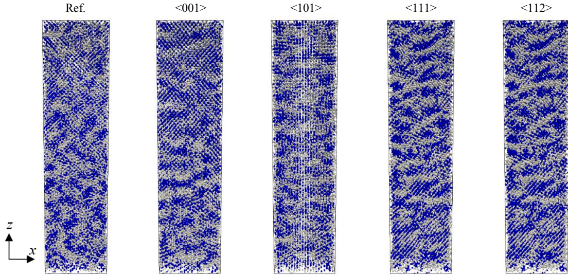
Figure 6-10. Orientation dependent decomposition of A-35B ( \rho_A = 0.052 , \rho_B = 0.028 ), at time step t = 2 \cdot 10^6 , tensile yield strain is 75%, the characteristic wavelength is compiled in Table 6-2.
