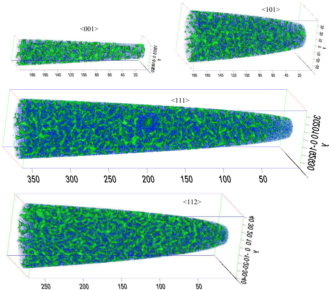
Figure 11-2. Orientation dependent APT reconstructions, iso -surface at 50at.%-Cr.
