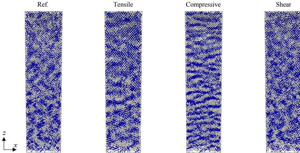
Figure 6-12. View of the {010}-plane with \langle 001 \rangle - strain direction, loading 75% of yield limit in tension/compression. The characteristic wavelength is for: reference state 14.12Å, tensile 13.35Å, compression 8.40Å and shear 11.68Å.
