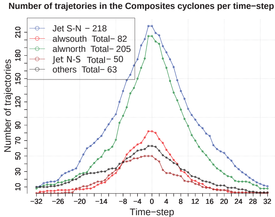
FIGURE 5.15: Number of trajectories used at each time step of the composites for the 5 types of trajectories separated according to their relative position to the jet stream .
