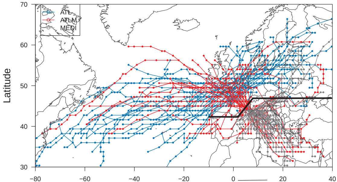
FIGURE 5.1: Trajectories for France with the highest MI separated into three categories : the ones always on the northern side of the separation line (the black straight legs), Atlantic (ATL, blue tracks); the ones that cross that line, Atlantic-Mediterranean (ATLM with red tracks) and the ones always south of this line, Mediterranean (MEDI, grey tracks).
