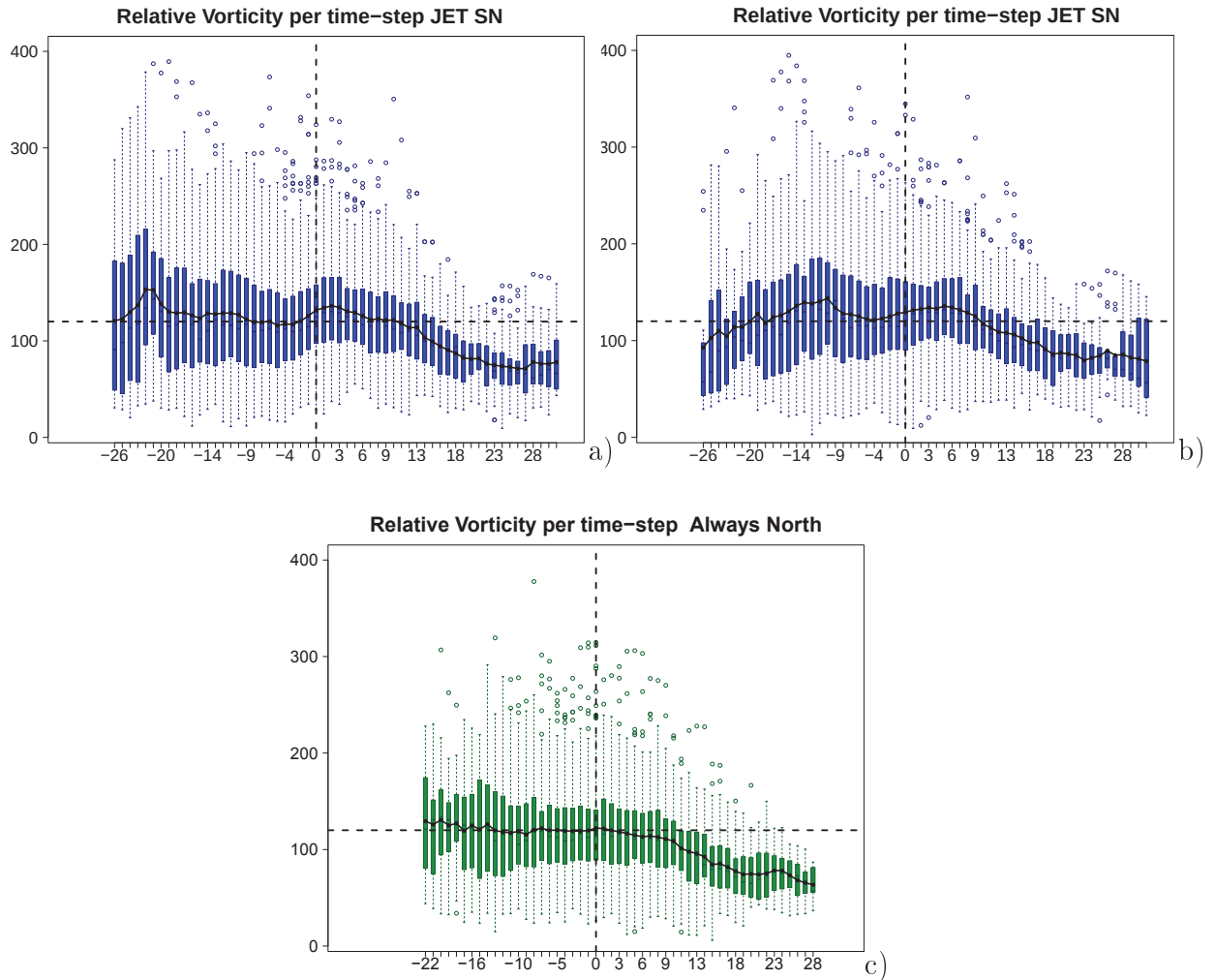
FIGURE 5.19: Boxplot (blue) and mean (black) relative vorticity per time step for the JET SN centred at t_0 (a) and centred at newt_0 (b). boxplot (green) and mean (black) relative vorticity for the Always North (c).
