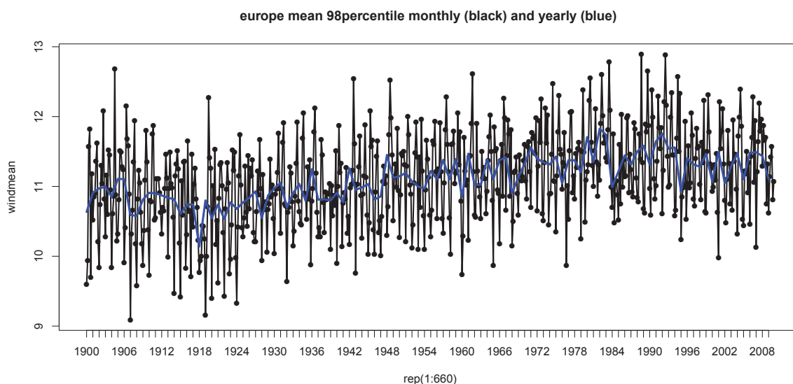
FIGURE 4.2: The temporal evolution of the average V_{98} for the Europe grid points. The black line represents the mean monthly time series and the blue one the yearly time series of this wind.
