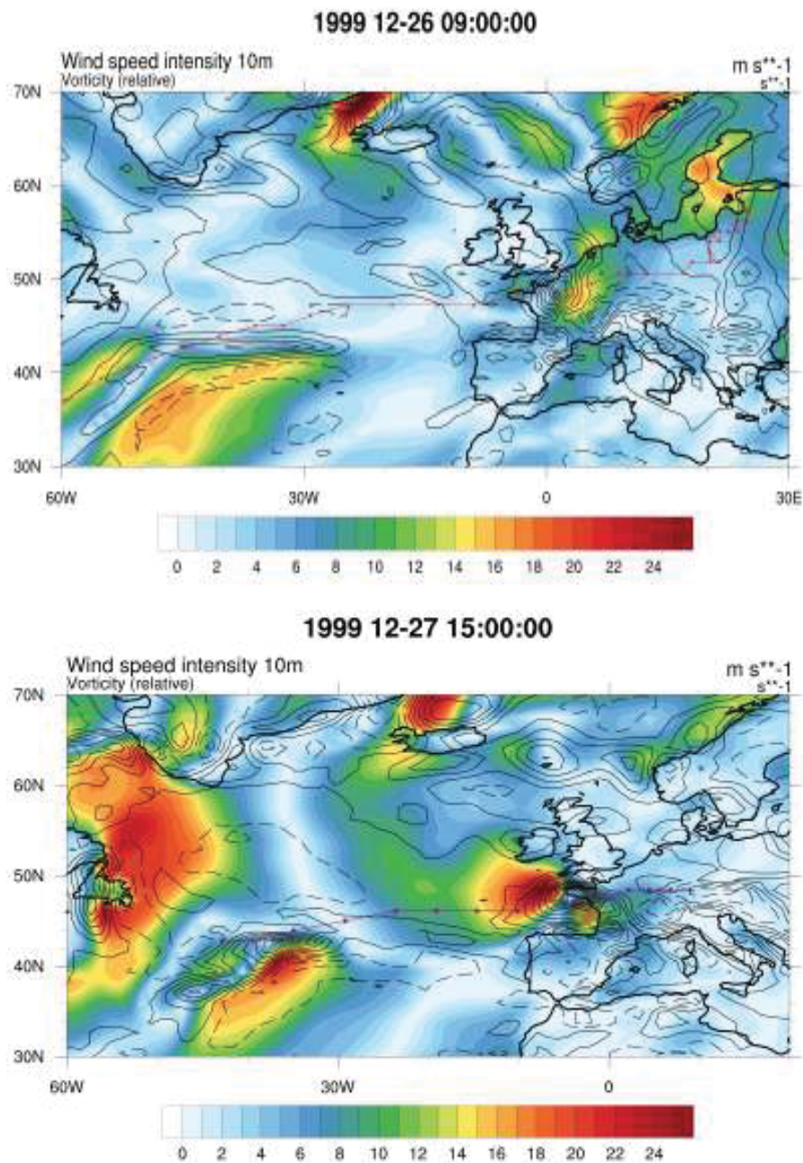
FIGURE 2.6: Trajectory obtained from the tracking algorithm (purple line) with the wind (shaded color contours) and vorticity (black line contours) for the storms :Lotar (top ) Martin (bottom).
