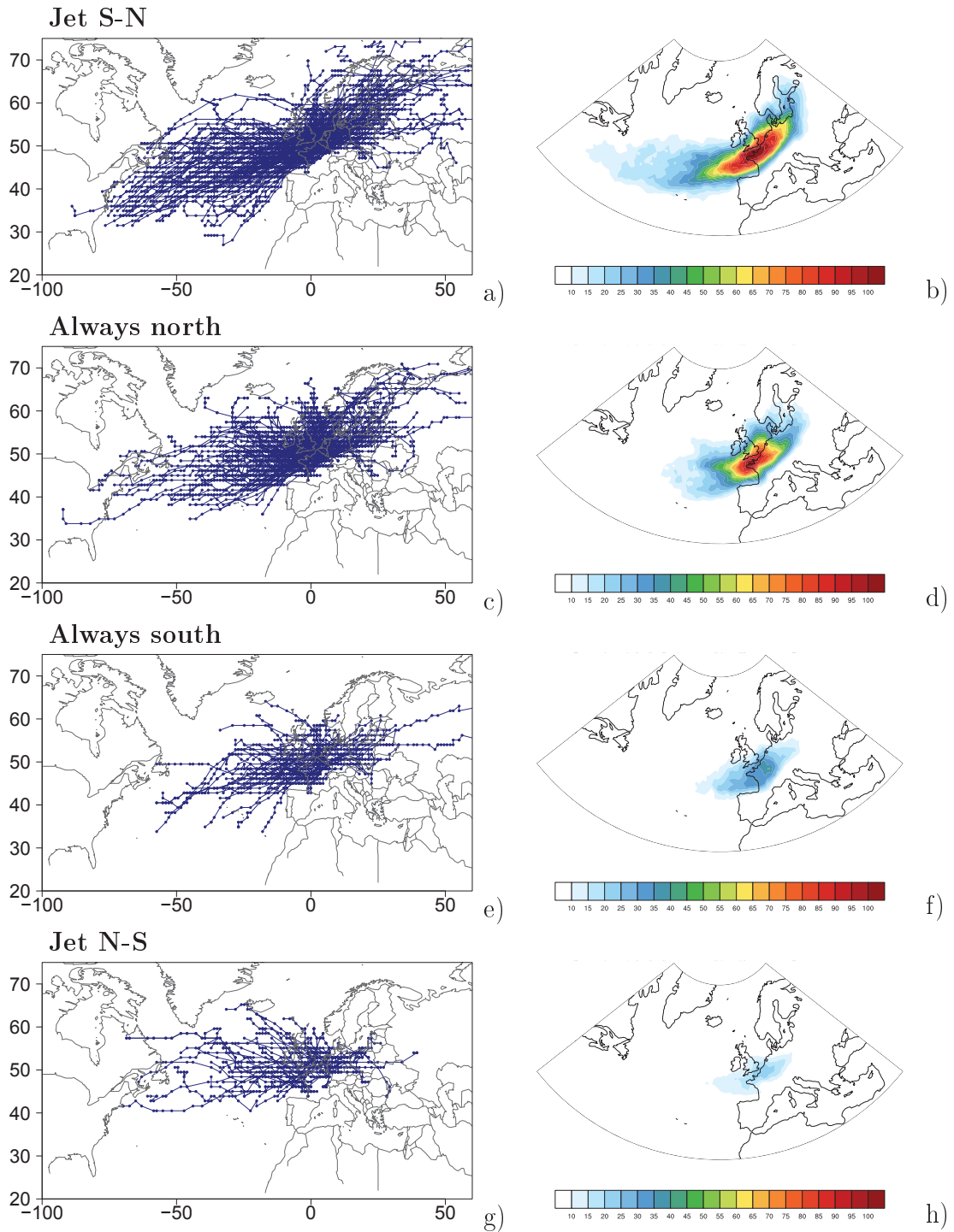
FIGURE 5.6: Trajectories (left) and Densities (right) of trajectories types for the ATL storms.
