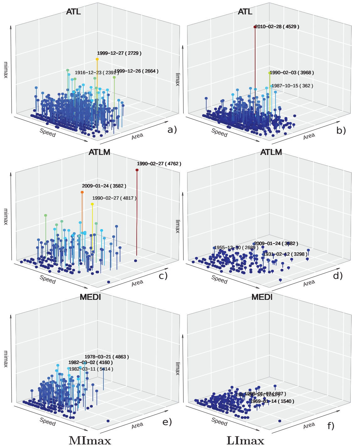
FIGURE 5.2: Mimax (left column) and LImax (right columns) in the Z axis and colours as a function of the displacement speed of the trajectory and Area of each trajectory of the ATL type( a and b); ATLM; (c and d) MEDI( e and f).
