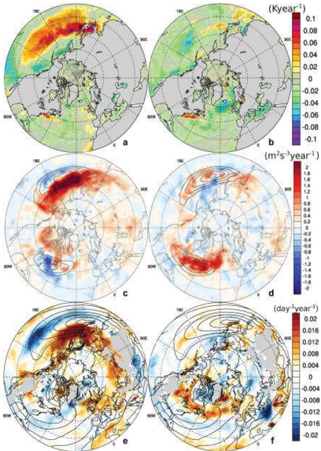
Fig. 11 a, b Sea surface temperature, c, d baroclinic conversion and e, f baroclinicity trends for (left column) period IIa and (right column) period IIb. Contours represent the mean field of the variable for each period in the same units as the trends (contour intervals of
