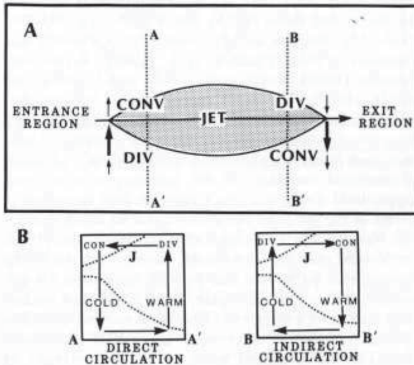
FIGURE 1.7: Schematic representation of the circulation around a jet streak (on the top). At the entrance zone the direct circulation (bottom left panel) creates divergence (convergence) at the right (left) region and at the exit zone an indirect circulation create the opposite. From Uccellini (1990).
