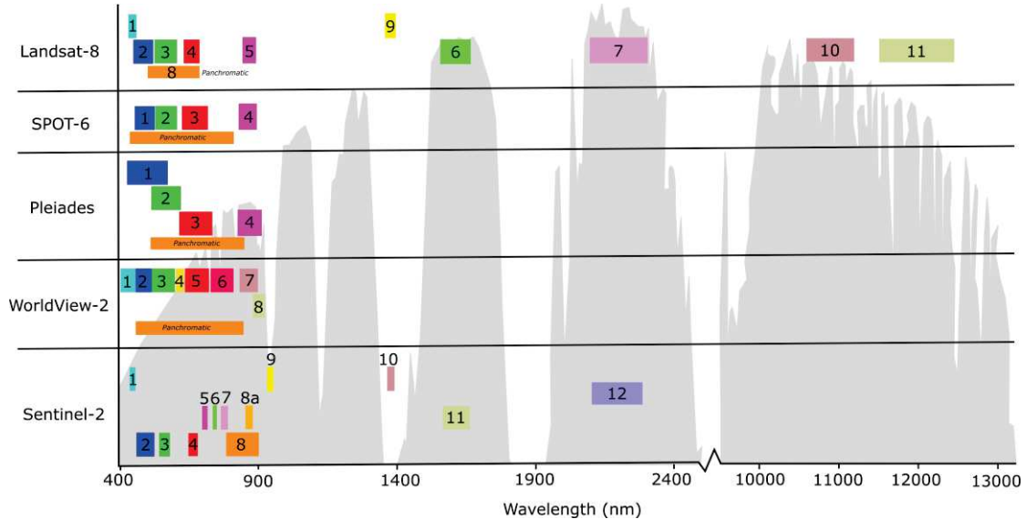
Figure 1. 6. Bands and their wavelength from several optical remote sensing data.
