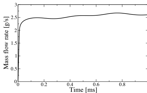
Figure 6.19: Injection mass-flow rate over time.
