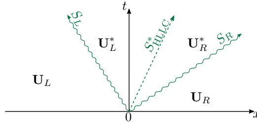
Figure 4.8: Approximation of the Riemann problem solution by the HLLC flux.
