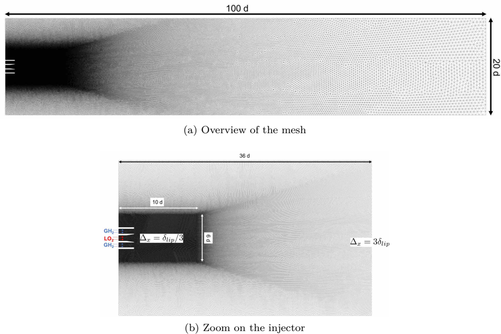
Figure 6.3: Computational domain and grid distribution for the two-dimensional simulations. d refers to the inner injector diameter, \delta_{lip} is the inner injector lip thickness and \Delta_x is the characteristic cell size.
