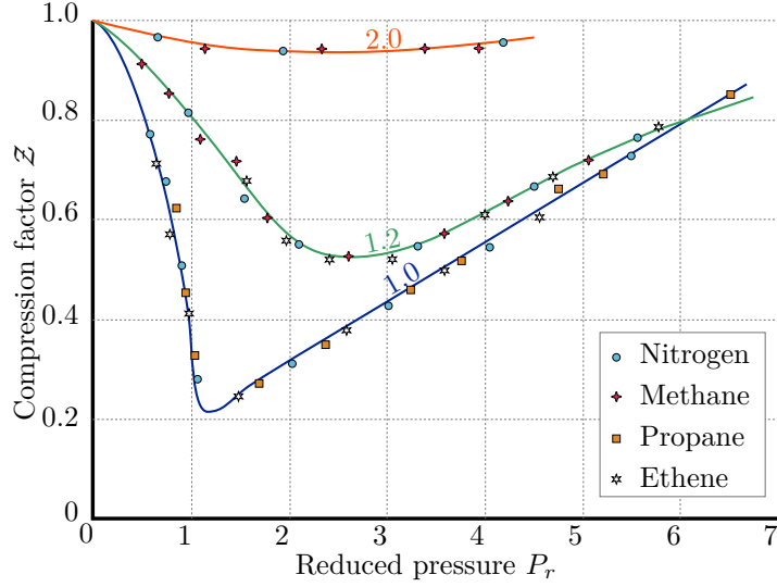
Figure 2.6: Compressibility factor \mathcal{Z} with respect to the reduced pressure P_r for different values of T_r and different pure species. The data for this image is taken from [Atkins et al., 2018]
