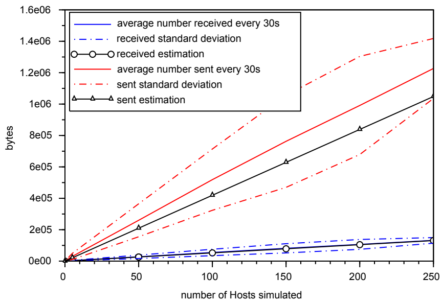
Figure 4.9 – Network traffic of the webmail server
