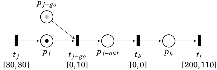
Figure 5.4: Transitions and places from a STPN model of a metro network.
