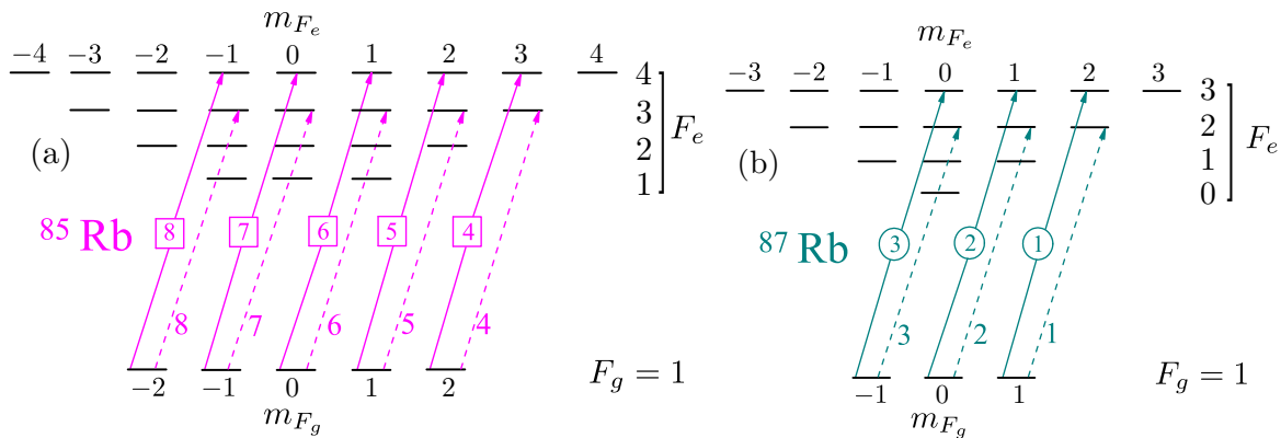
Figure 3.11: Diagram of the relevant transitions between the Zeeman sub-levels of Rb D_2 line with \sigma^+ laser excitation for the case of (a) ^{85}\text{Rb} (nuclear spin I = 5/2 ), and (b) ^{87}\text{Rb} (nuclear spin I = 3/2 ). Each transition is labeled to facilitate identification in the following graphs.
