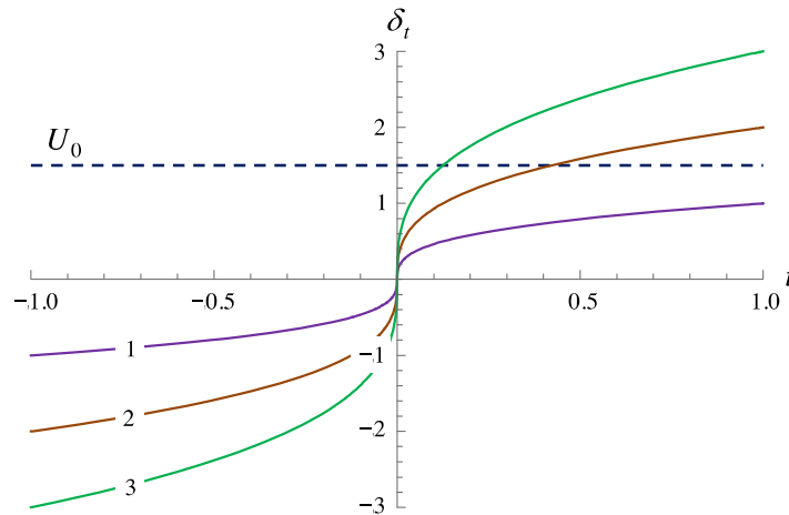
Fig. 5. Bi-confluent Heun class k = +1/2 , z(t) = t^{2/3} , U_0 = 1.5 . Detunings corresponding to \Delta_2 = 1; 2; 3 (curves 1, 2, 3, respectively).
