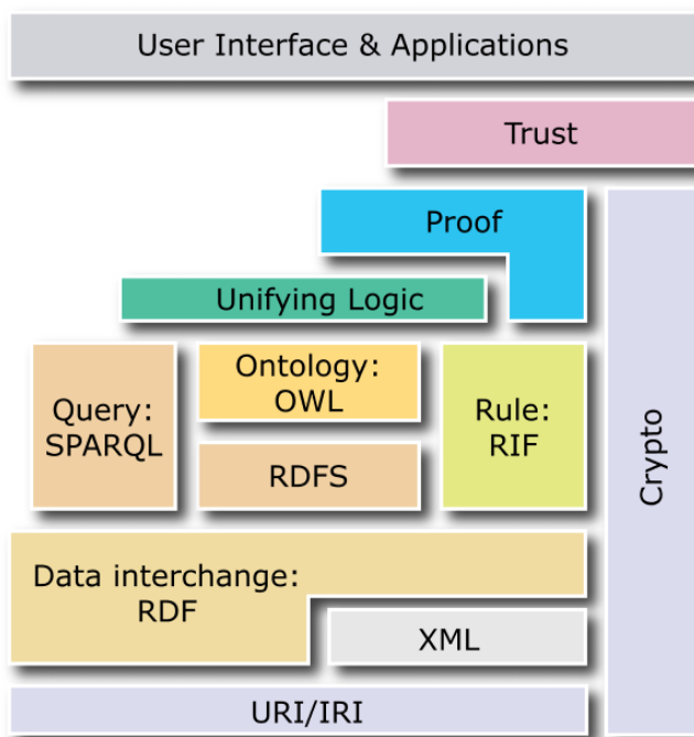
FIGURE 2.3 – Pile du web sémantique [Working Group, 2012b]
