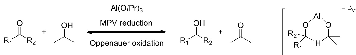
Scheme B III .1 Equilibrium between MPV reduction and Oppenauer oxidation.
