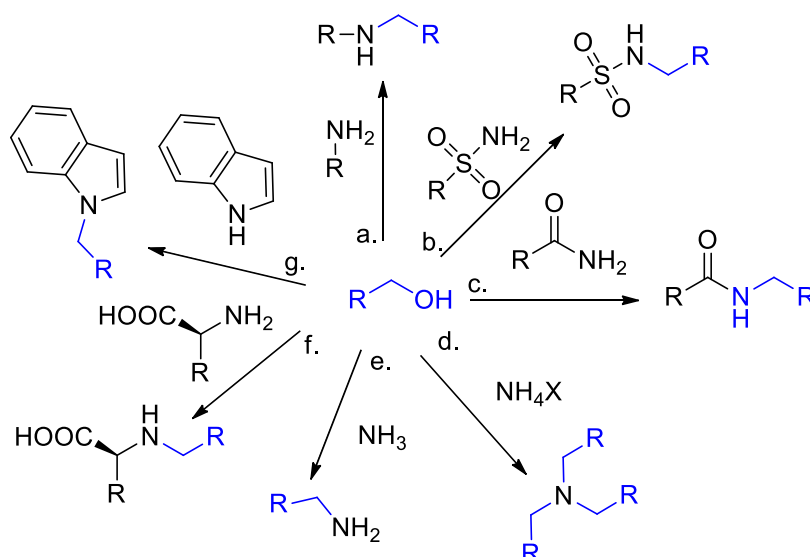
Scheme B 1111 .6 Substrate scope for C-N bond formation with alcohol.
