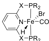
Fe-2 Milstein 2011 X=CH 2 Fe-3 Kirchner 2014 X=NH Fe-4 Mezzetti 2018 X=CH 2
