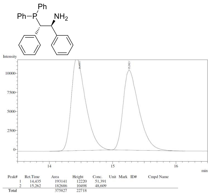
Figure S57: Chromatogram of enantio-enriched 1-phenylethanol b'1 with L 3B .31
