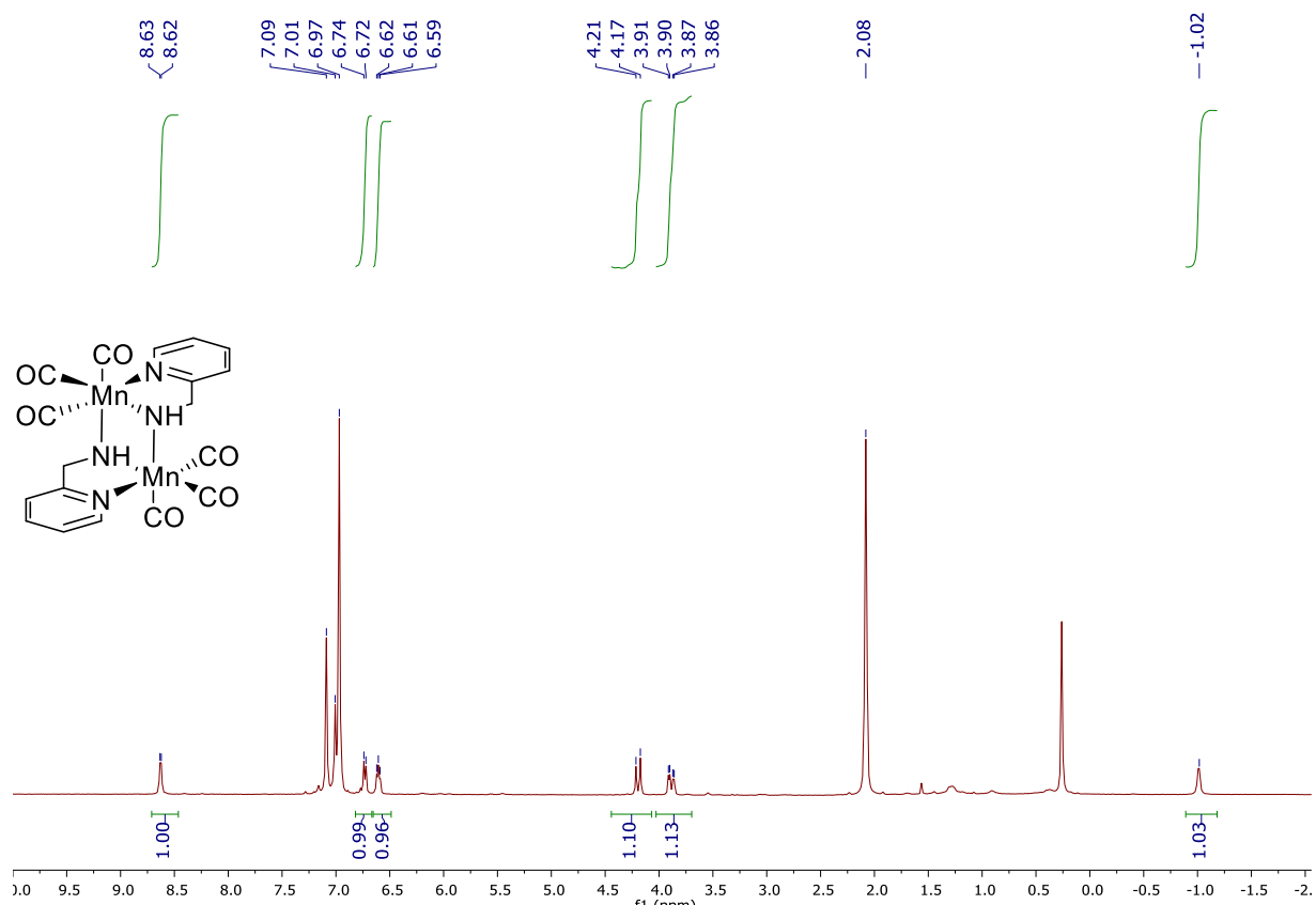
Figure S39: ^1\text{H} NMR spectrum of manganese complex C 3B .1b in toluene- d_8 (400 MHz).
