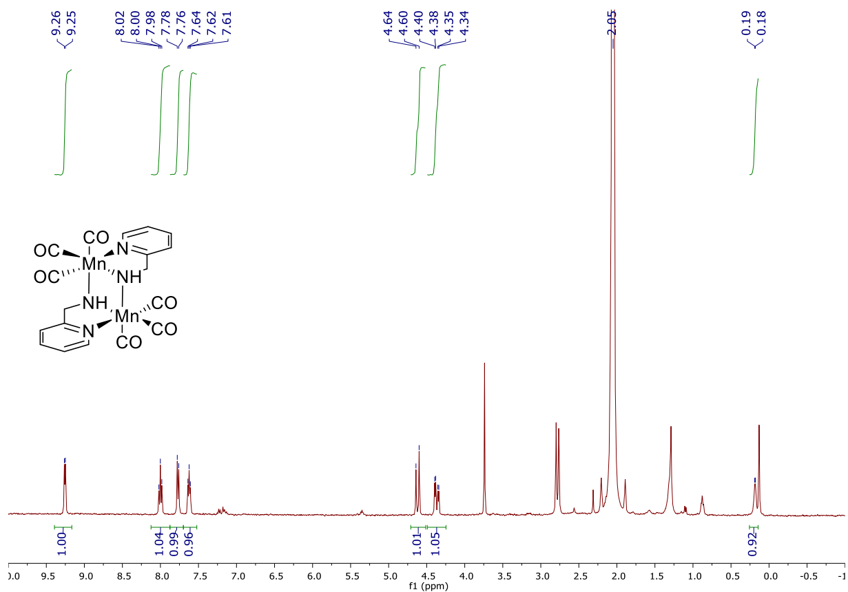
Figure S40: ^1\text{H} NMR spectrum of manganese complex C 3B .1b in (\text{CD}_3)_2\text{CO} (400 MHz).
