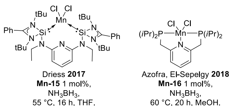
Figure A 4II .2 Manganese complexes used to catalyze transfer hydrogenation of alkynes
