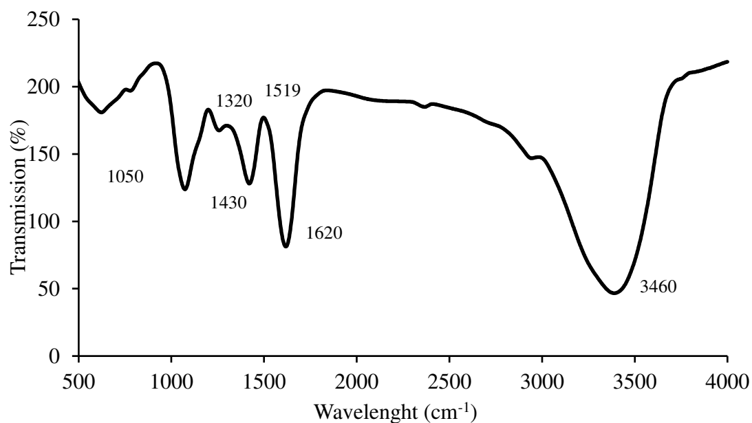
Fig. 3 FTIR spectrum for 2.5 mg of cactus solid material (CSM)
