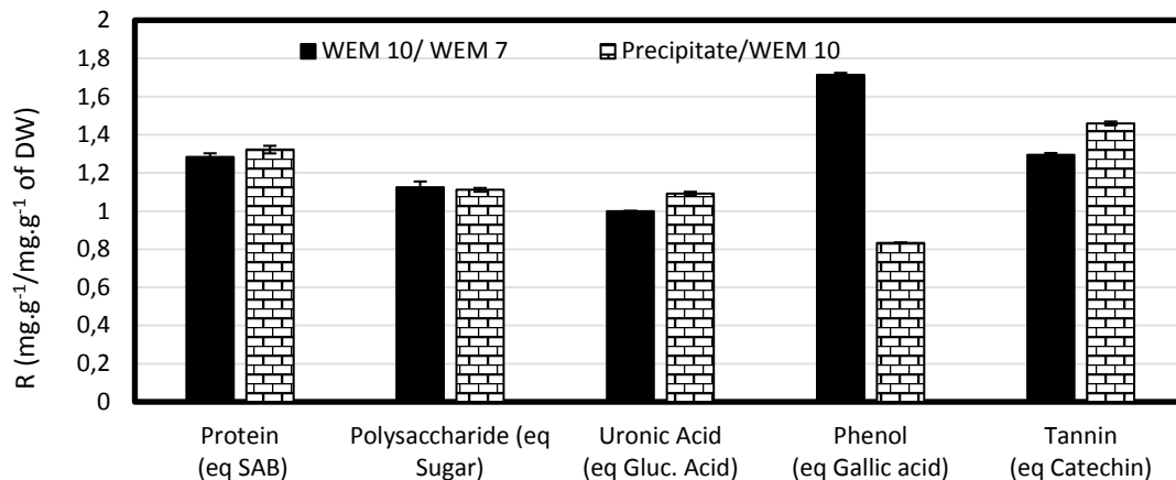
Fig. 3: Ratio (R) of the content of specific biochemical molecules between two cactus extract fractions: the WEM 10/WEM 7 and precipitate/WEM 10 ratios
