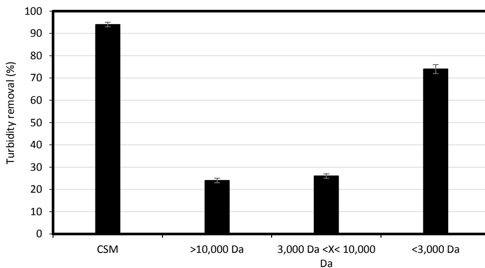
Fig. 1: Coagulation flocculation results of the size-fractionated parts of the PP (precipitate), compared to CSM (cactus solid material) under optimal conditions ( 35 \text{ mg L}^{-1} , pH 10)
