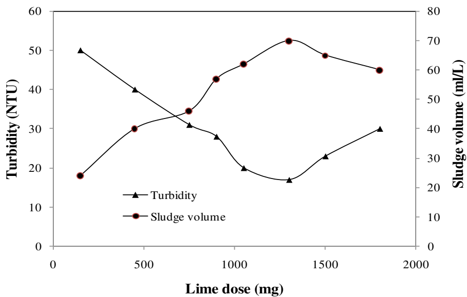
Figure 1c: Evolution of turbidity and sludge volume depending on the dose of \text{Ca(OH)}_2
