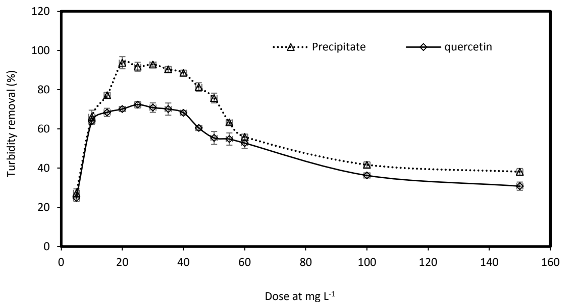
Fig. 5: Comparison of turbidity removal rates between quercetin and the precipitate (PP) by means of coagulation flocculation and settling at pH 10 for various material doses ( \text{mg} ) n = 3
