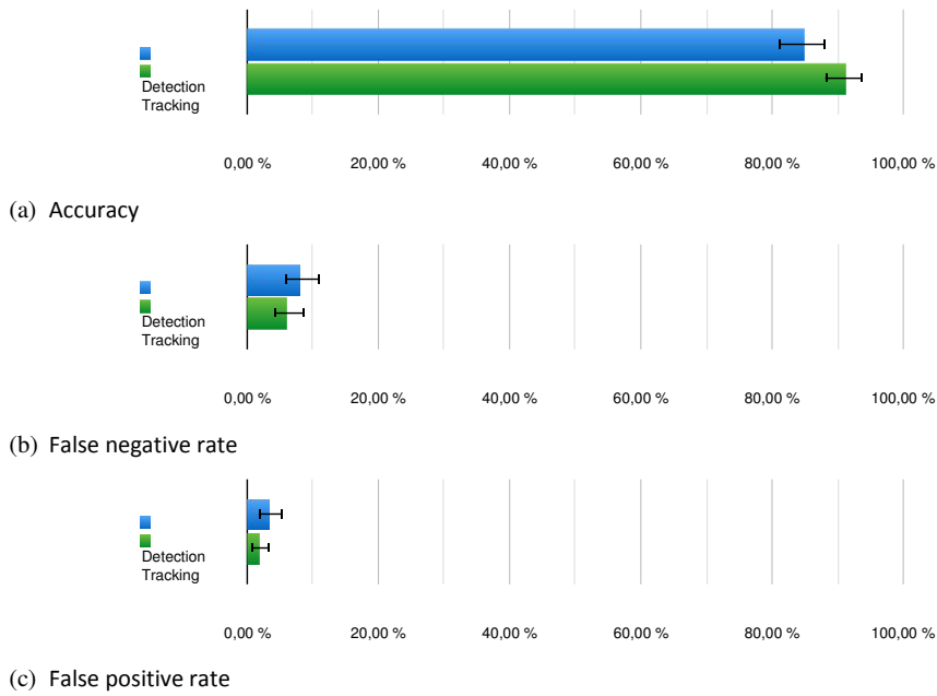
FIGURE 5.5: Average results over 8 random frames
