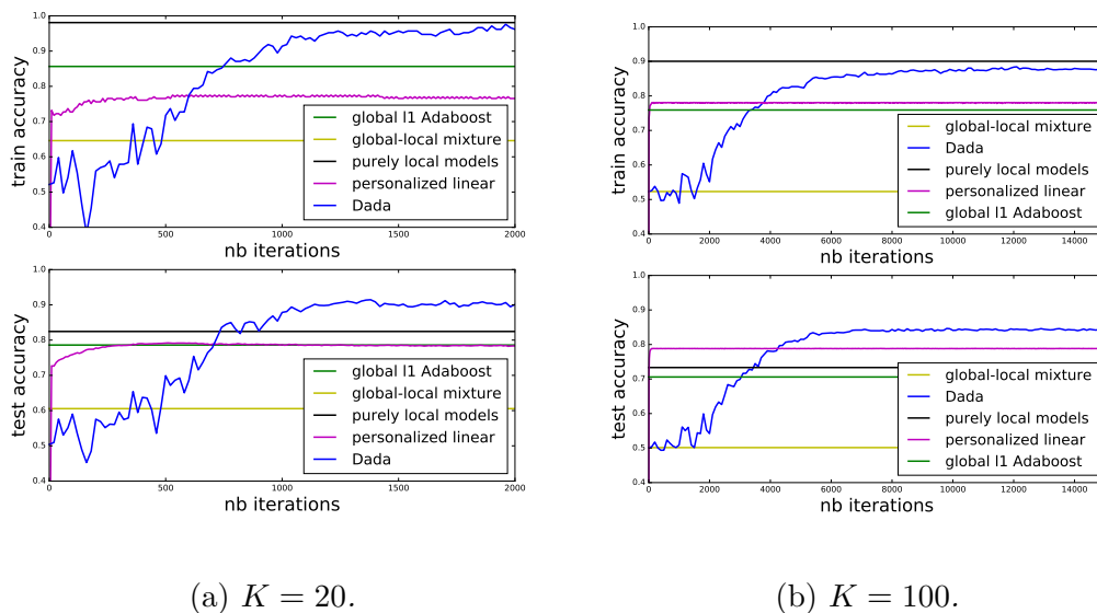
Figure 4.4 – Training and test accuracy w.r.t. number of iterations.
