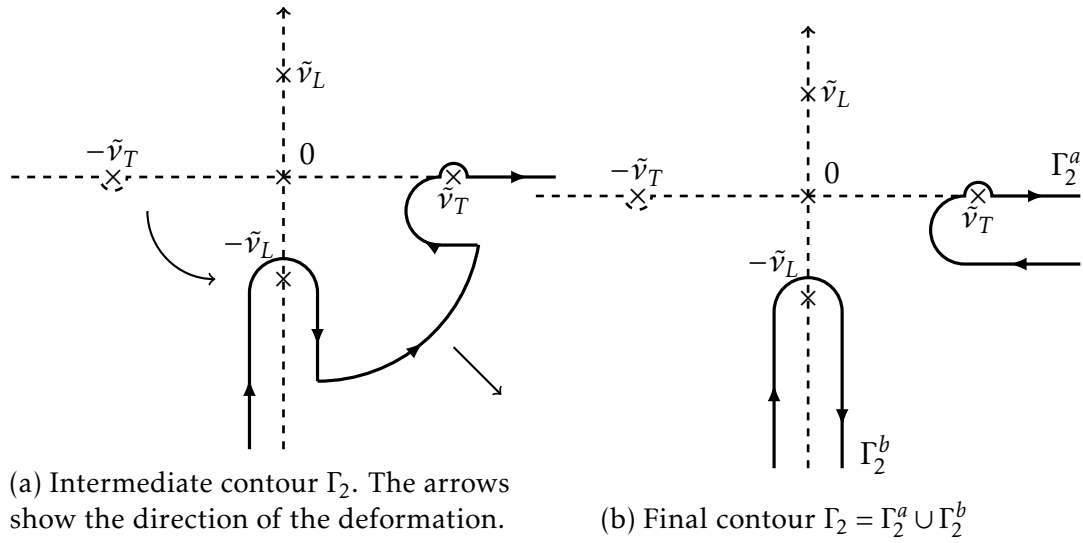
Figure 4.9 – Deformation of contour \Gamma_0 onto contour \Gamma_2 = \Gamma_2^a \cup \Gamma_2^b in the case \tilde{\nu}_L \in i\mathbb{R} .
