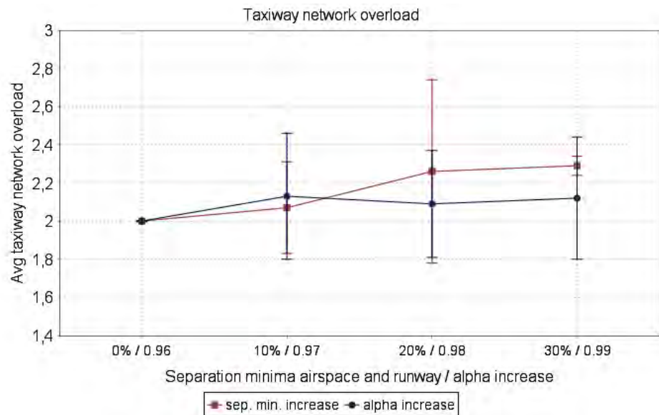
Figure 4.16: Number of taxiway network conflicts.
