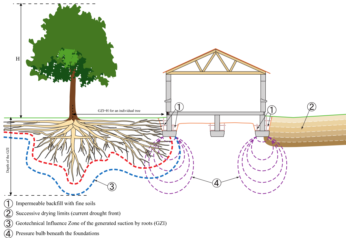
Figure 1.20 - Schematic representation of the influence of trees on the differential soil movements of constructions. (Béchade, 2015)
