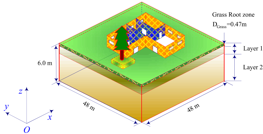
Figure 1.35 - The 3D geometry of the Arlington site modelled in ABAQUS (Zhang & Briaud, 2015)
