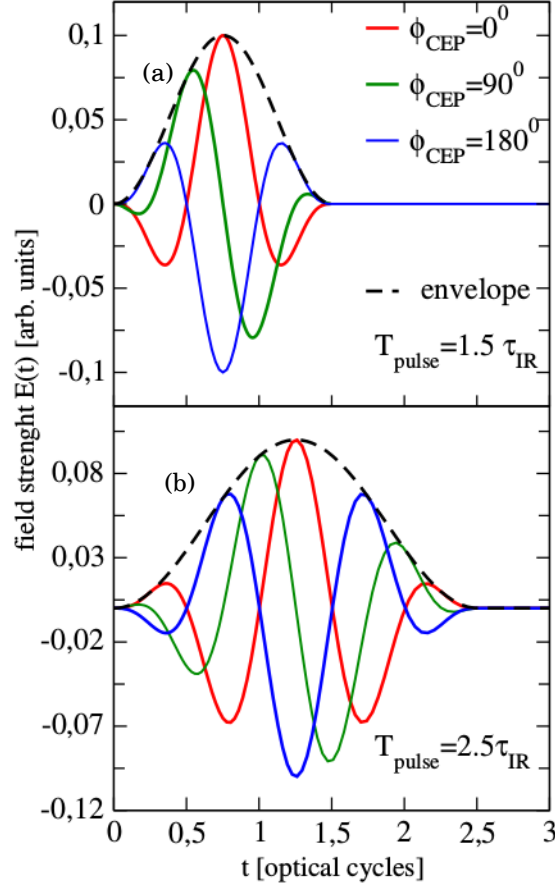
Figure 4.22: Shape of the laser pulse for (a) T_{pulse} = 4.0 fs and (b) T_{pulse} = 6.6 fs. In both cases three values of the CEP parameter are represented \phi_{CEP} = 0^{\circ}, 90^{\circ}, 180^{\circ} , the envelope is plotted with a thin dashed line.
