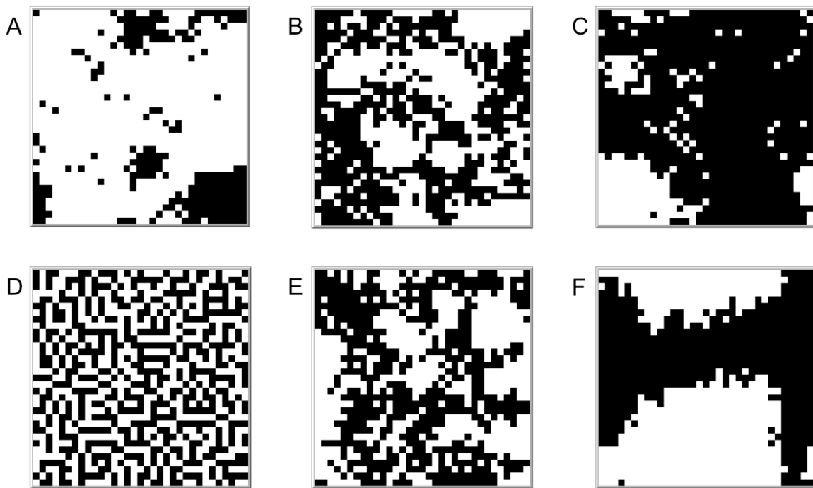
Figure 5: examples of the two scenarios of spatial heterogeneity in our model. White areas correspond to patches with a high level of fertilization. Black areas correspond to patches with a lower fertilization level. In the upper line, we change the proportion of patch type. A: 80/20%; B: 50/50% and C: 20/80% of strongly and less fertilized patches respectively. The aggregation level in landscapes A, B and C is 5.2 similar neighbours in average. In the lower line, we vary the level of patch aggregation. D: low aggregation landscape, E: average aggregation landscape and F: high aggregation landscape, corresponding to 3.2, 5.2 and 7.2 similar neighbours in average respectively.
