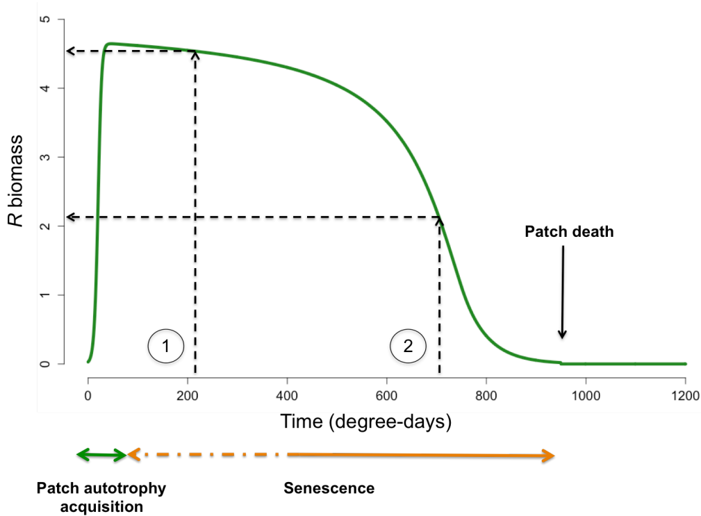
Figure 3 : within (healthy) patch dynamics of resources R . After patch creation, R increases simulating patch development and acquisition of patch autotrophy to carbon and nitrogen. Once the patch becomes mature, R starts decreasing mimicking patch senescence and patch resource re-allocation to other patches in younger organs higher in the canopy. Patch death occurs after R drop under a viability threshold R_{min} . Pathogens infecting at different times (1 and 2 for example) do not encounter the same resource environment: the pathogen infecting in (1) having access to twice the resource level of a pathogen infecting in (2).
