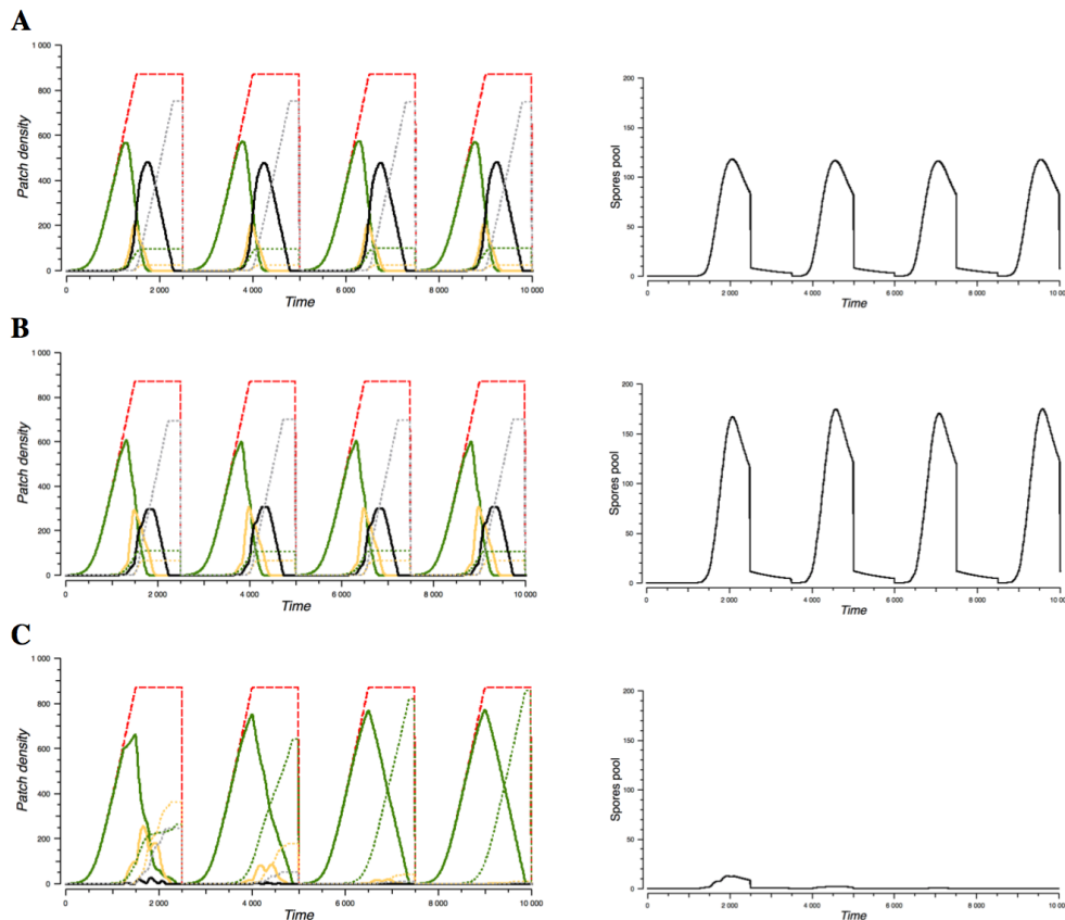
Figure 14. Times series for three values of the latent period. Left panels: canopy and epidemics. Right panels: dynamics of the spores pool P(t) . A: \lambda=90 . B: \lambda=150 . C: \lambda=240 . The epidemics are stable from year to year in panels A and B whereas it is ephemeral in panel C. Parameters: T_{inoc}=1000 , and see Table 1.
