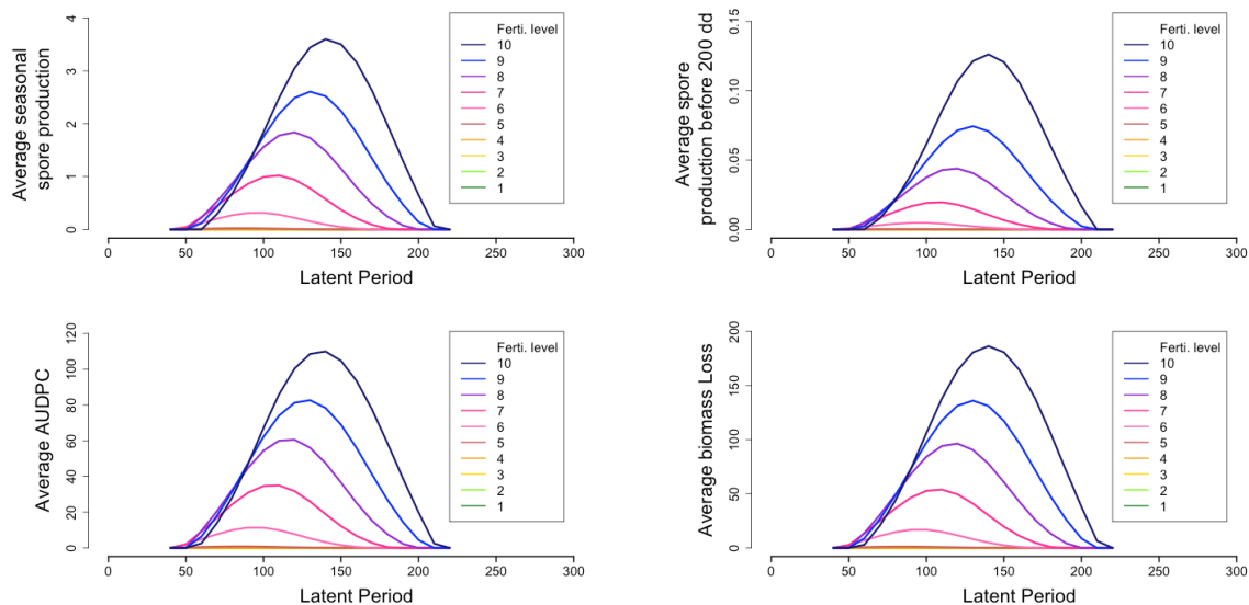
Figure 11: effect of latent period on pathogen development for different fertilization levels in a homogeneous landscape. A: seasonal spore production; B: spore production from the beginning of the epidemic to 200 dd; C: the area under disease progress curve (AUDPC) and D: biomass loss. For the sake of comparison with Figure 10, we represented per patch average values for all four quantities. In panel A, B and C, the summit of each curve corresponds to the optimal latent periods (see Figure 16).
