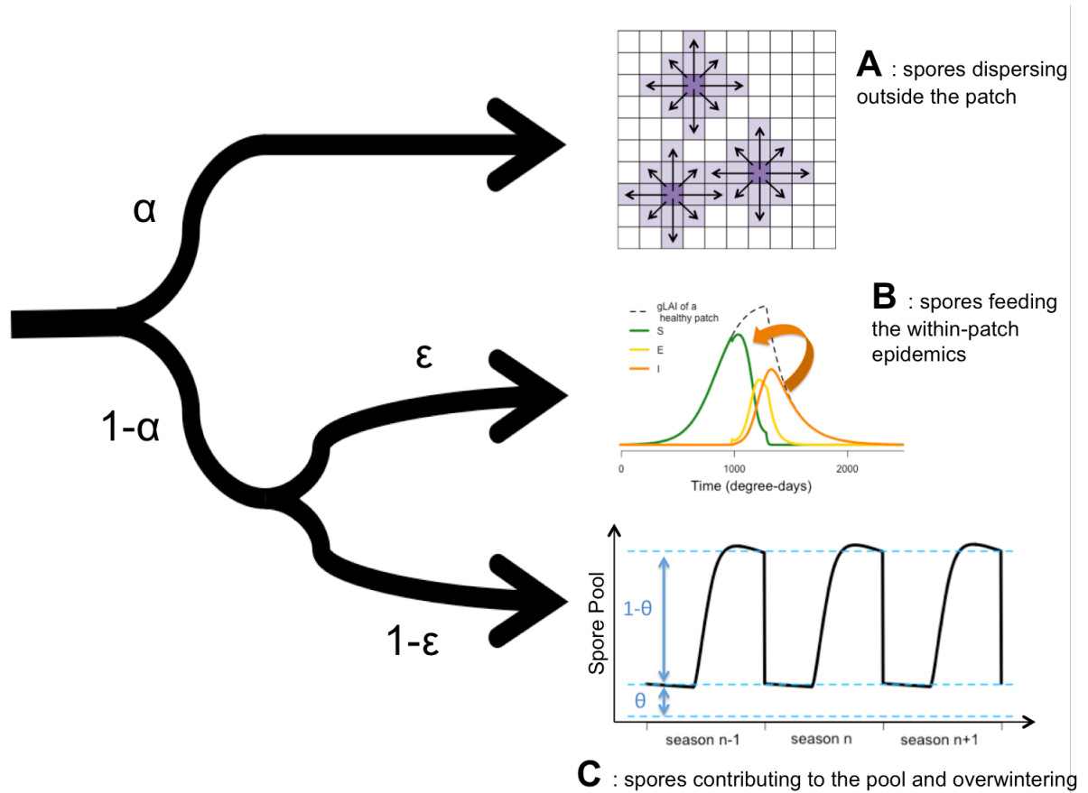
Figure 4: overview of the different fates of pathogen spores in the model. The black arrow represents the sporulation rate in a given field at a given time. A: a fraction \alpha of spores disperses to other fields within a radius \Delta . In this example, dark purple patches are already infected. Light purple ones are their - yet uninfected - neighbours within a range \Delta = 2 . The amount of spores received by each neighbour is inversely proportional to its distance to the sporulating patch (Equations 18 to 22). B: a fraction \epsilon of the non dispersing spores feeds the local epidemic (Equations 12 and 13 and Figure 2). C: The fraction (1 - \epsilon) enters the field's spore pool P . Spores in this compartment decay at a rate \rho . At the end of a season, only a fraction \theta of the spore pool survives harvesting and the interseason and make it to the next season and form the internal primary inoculum of the new season. For more details, see Equations 11 and 16.
