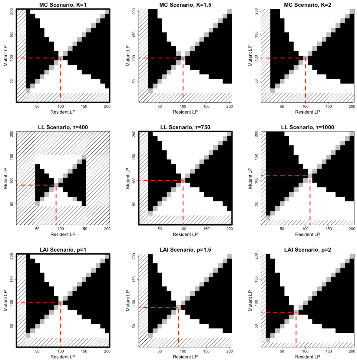
Figure 1: pairwise invisibility plots for three fertilization levels of each modelling scenario. Modelling scenarios correspond to the main effects of fertilization on the pathosystem. Upper line: “Metabolite Concentration” (MC) effect. Middle line: “Leaf Lifespan” (LL) effect. Lower line: “Leaf Area Index” (LAI) effect. Corresponding fertilization parameters ( K , \tau , and \rho respectively) increase from left to right. In black areas, mutants have a positive invasion fitness. In white areas, they have negative ones. The singular strategies are highlighted by dashed red segments. There are no sustainable epidemics in the dashed areas of the parameter space. Black boxes indicate standard parameter values in Précigout et al. (2017).
