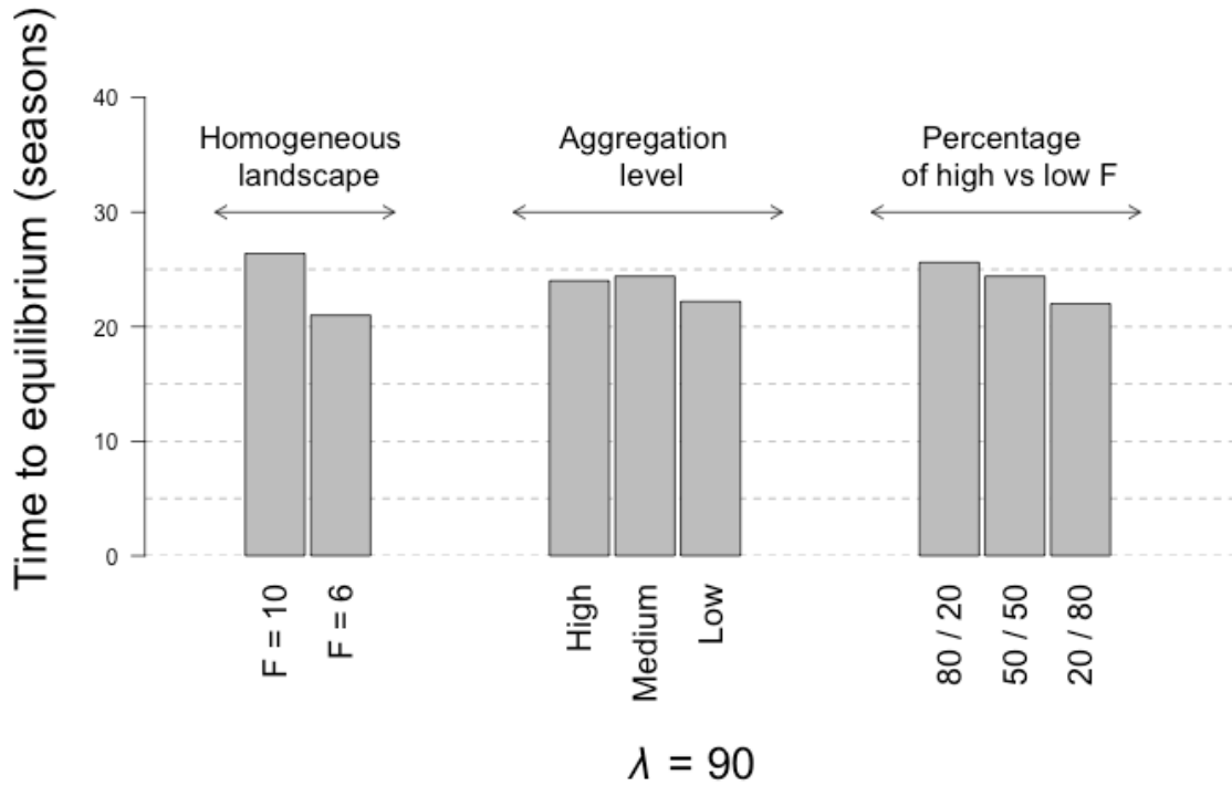
Figure SM2: effect of spatial heterogeneity on the speed of landscape colonization by the pathogen with \lambda = 90 dd, measured as the time for the epidemics to reach a steady state. Here, we compare homogeneous landscapes with high ( F = 10 ) and low ( F = 6 ) fertilization and heterogeneous landscapes with various aggregation levels or various proportions of field types. The aggregation level is the same in landscapes with different field type proportions (medium aggregation) and reciprocally, the proportion of fields of each type is the same in landscapes with different aggregation levels (50/50). Data are average values from 5 repetitions. \lambda = pathogen latent period; F = fertilization level.
