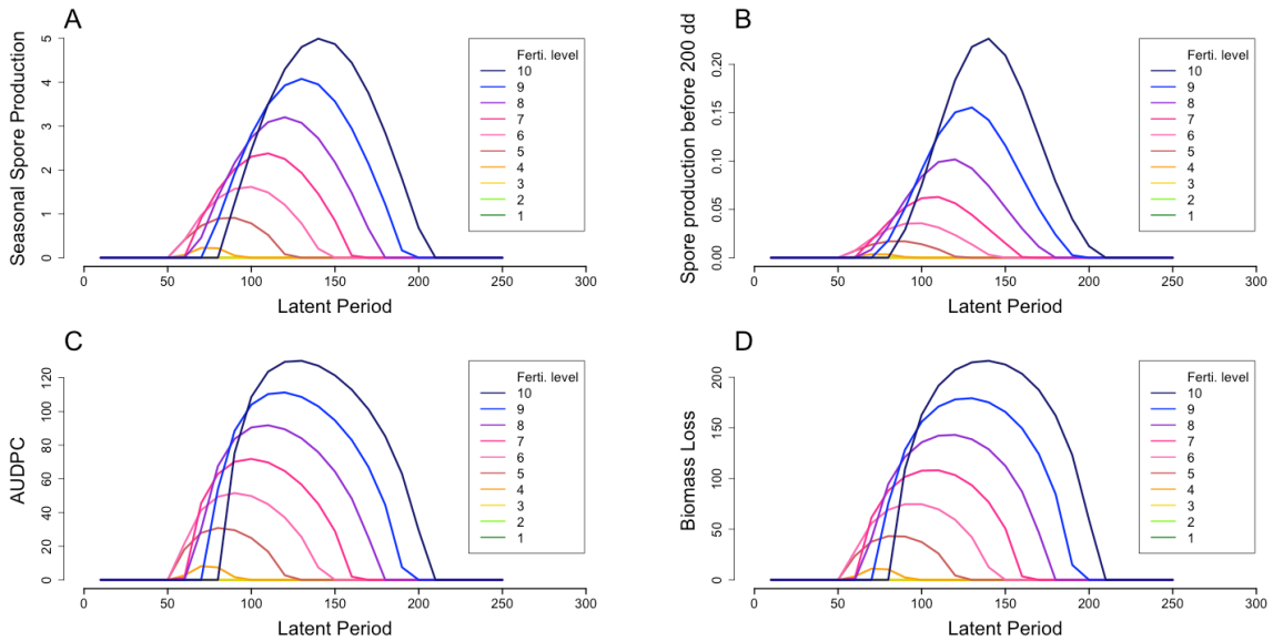
Figure 8: field-scale effect of pathogen latent period on A: seasonal spore production; B: spore production from the beginning of the epidemic to 200 dd; C: the area under disease progress curve (AUDPC) and D: biomass loss. Colors from green to blue represent a range of fertilization from F = 1 to F = 10 . In panel A, B and C, the summit of each curve corresponds to the optimal latent periods (see Figure 15).
