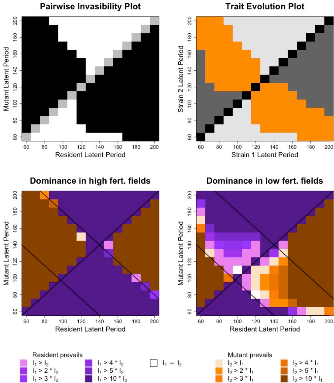
Figure 21: pairwise invisibility plot (PIP), trait evolution plot (TEP) and dominance plots for a medium aggregation heterogeneous landscape with a 50/50 percentage of patch types. Top-left: PIP. Black areas correspond to mutant strategies capable to invade the resident population. White areas correspond to mutants that fail in the invasion process. The first diagonal has been highlighted in grey for the sake of clarity. Top right: TEP. Light grey areas correspond to strategies where only strain 1 can invade strain 2. Dark grey areas correspond to strategies where only strain 2 can invade strain 1. Orange areas correspond to strategies allowing for mutual invisibility, that is coexistence in adaptive dynamics. The first diagonal has been highlighted in black for the sake of clarity. Bottom left: dominance in the high fertilization fields of the heterogeneous landscape 100 seasons after the start of the epidemics. Warm colours indicate dominance by the mutant strain. Cold colours indicate dominance by the resident strain. White area indicate even coexistence. Bottom right: dominance in the low fertilization fields of the heterogeneous landscape 100 seasons after the start of the epidemics. The legend is the same for both coexistence plots. In this figure, I_1 and I_2 refer to the AUDPCs of the resident and mutant strains respectively. The first diagonal and the zero isoclines from field-scale PIPs ( F = 6 and F = 10 ) have been superimposed as solid grey or black lines on both dominance plots for the sake of interpretation.
