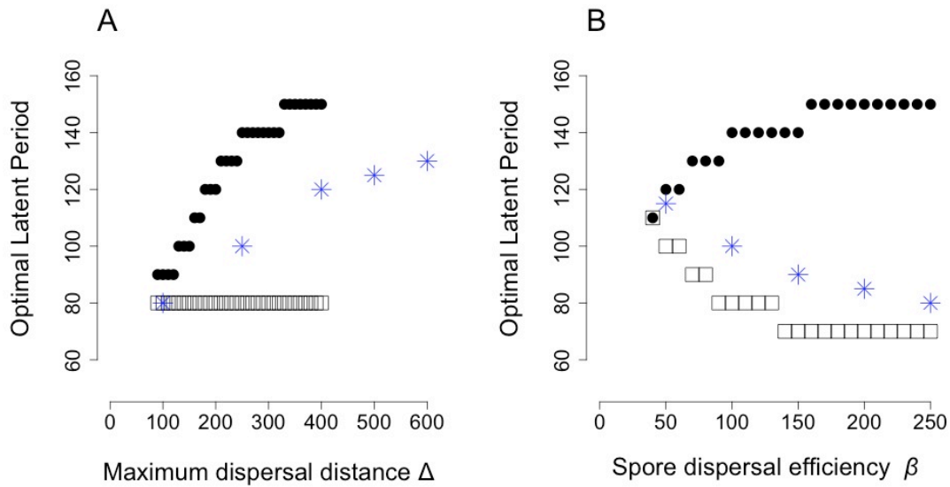
Figure 1 : Variation of optimal latent periods with A : the maximum dispersal distance \Delta and B : the spore dispersal efficiency \beta in the reference fertilization parameters ( K = 1 , \tau = 750 , \rho = 1 ; default values are \beta = 100 and \Delta = 250 ). Full circles are optimal latent periods corresponding to seasonal spore production as a fitness measure. Open squares are optimal latent periods corresponding to within-season exponential growth rate as a fitness measure of the pathogen. Blue stars correspond to the evolutionary singular strategies (ESS).
