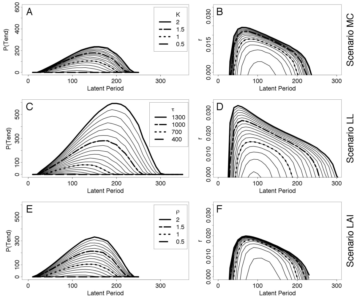
Figure 6: Fitness curves for range of fertilization and for two different fitness definitions. The summit of each curve indicates the optimal latent period. A, C, and E, Variation of total seasonal spore production P(T_{end}) with pathogen's latent period. B, D, and F, Variation of within-season exponential growth rate of the pathogen r with latent period (see equation 5 in the text for r calculation). K = patch resource carrying capacity, \rho = maximum patch creation rate, and \tau = patch lifespan.
