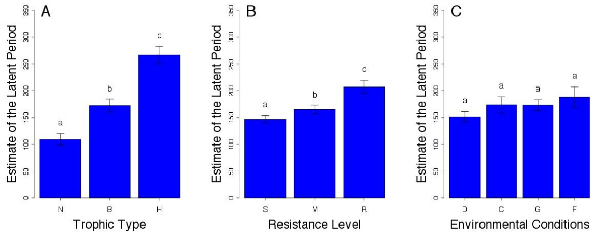
Figure 3: Least squares means latent periods and standard errors obtained using the statistical model for each mode of the three explanatory variables. Main effects of: A: trophic type (N: necrotrophs; B: biotrophs; H: hemibiotrophs; contrasts: N-B, p = 0.0016 ; B-H, p < 0.0001 ; N-H, p < 0.0001 ); B: Resistance level of the host (S: susceptible; M: moderately resistant; R: resistant; contrasts: S-M, M-R and S-R, p < 0.0001 ); C: Environment of the study (D: detached leaves or leaf disks; C: controlled environment cabinet; G: greenhouse; F: field; contrasts: C-D, p = 0.4179 ; C-F, p = 0.8739 ; C-G, p = 1.000 ; D-G, p = 0.1464 ; D-G, p = 0.2715 ; F-G, p = 0.6675 ). Within the same graph, different letters indicate significant contrasts. Latent periods are in degree-days.
