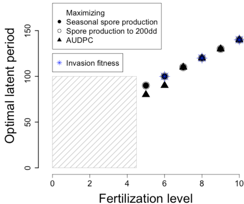
Figure 12: variation of the optimal latent periods and the ESS with fertilization in a homogeneous landscape. Full circles correspond to seasonal spore production as a fitness measure. Open circles correspond to spore production at the beginning of the epidemics as a fitness measure (see Figure 20). Full triangles correspond to canopy colonization as a fitness measure (measured as the AUDPC, see Equation 23). Blue stars correspond to the evolutionary singular strategy derived from invasion analysis. There are no sustainable epidemics in the striped area of the parameter space
