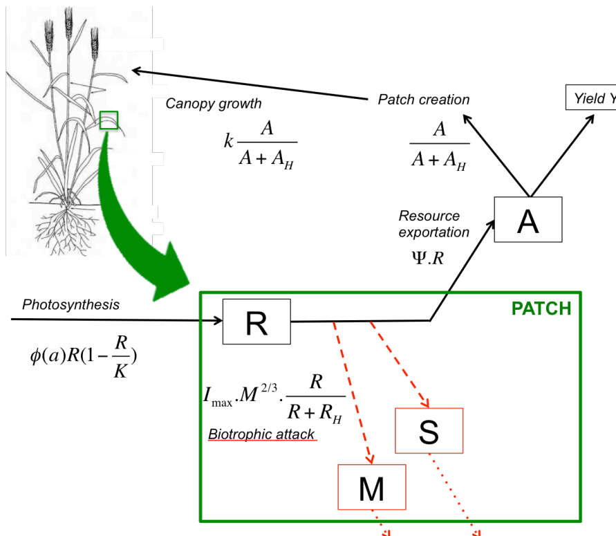
Figure 2: schematic view of patch functioning and of the role of patches in the building-up of a healthy canopy. A patch is defined as a unit of leaf tissue the size of a mature lesion (about 0.1 cm 2 ). It is characterized by patch-level state variables that define patch age a , time since infection b , within-patch resource level R and pathogen biomass M and S . Resources created in all patches are in part exported towards a common resource
