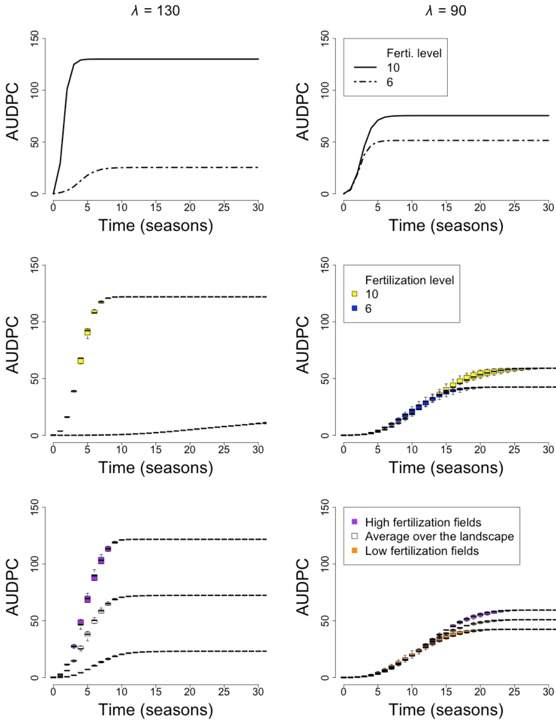
Figure 10: time series describing within-field epidemics (upper line) and landscape colonization by the pathogen (middle and lower lines). Upper line: area under disease progress curve (AUDPC) for a single field. Solid lines: high fertilization ( F = 10 )/ Dotted line: low fertilization ( F = 6 ). Middle line: average AUDPC of fields in a homogeneous landscape. Boxplot represent average values for 5 repetitions. Yellow: high fertilization landscapes ( F = 10 ); blue: low fertilization landscapes ( F = 6 ). Lower line: average AUDPC of fields in a heterogeneous landscape. Boxplot represent average values for 5 repetitions. Aggregation index = 5.2 and there is an even proportion of both patch types. Purple: high fertilization fields within the heterogeneous landscape; orange: low fertilization fields within the heterogeneous landscape; open boxplots: AUDPC values averaged over the landscape. Latent period decreases from left to right. Left column: \lambda = 130 dd. Right column: \lambda = 90 dd.
