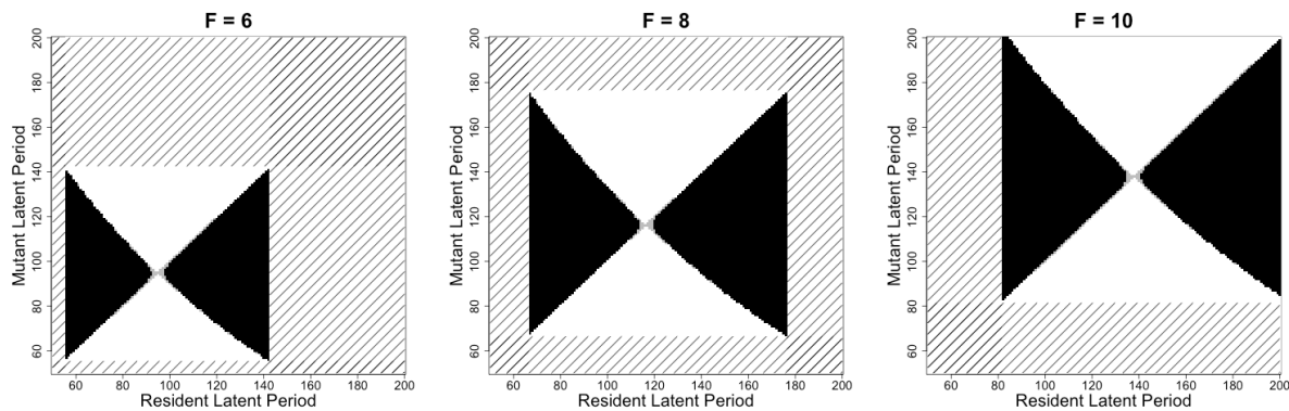
Figure 18: field-level pairwise invisibility plots for three fertilization levels. From left to right: F = 6 ; F = 8 and F = 10 . Black area correspond to winning mutant strategies while white area correspond to mutants unable to invade the resident population. Similar strategies on the first diagonal have been highlighted in grey for the sake of clarity. Corresponding evolutionary singular strategies are 9.5, 11.7 and 13.8 for fertilization levels 6, 8 and 10 respectively.
