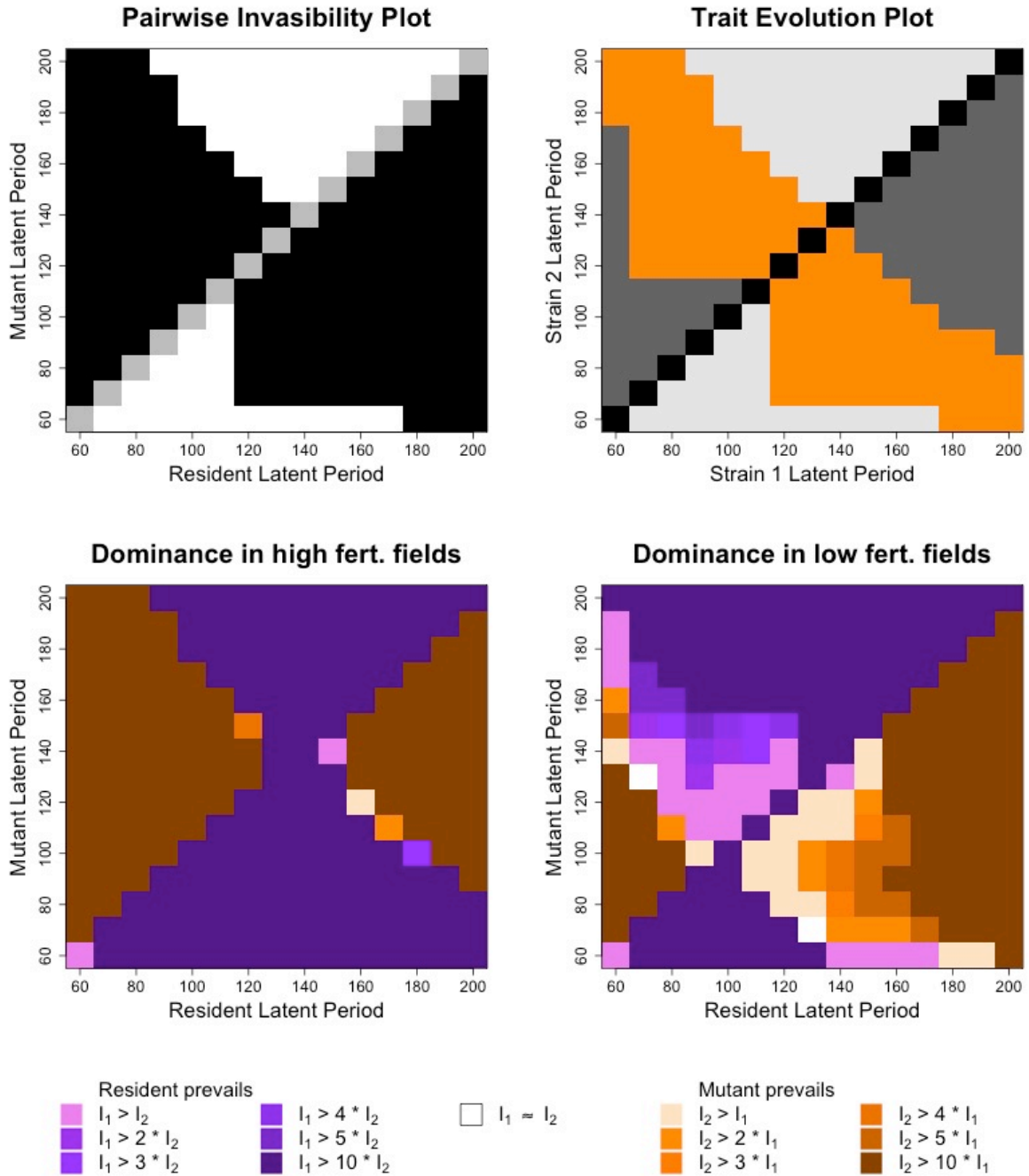
Figure SM4: pairwise invisibility plot (PIP), trait evolution plot (TEP) and dominance plots for a medium aggregation heterogeneous landscape with a 20(F6)/20(F10) percentage of patch types. Top-left: PIP. Black areas correspond to mutant strategies capable to invade the resident population. White areas correspond to mutants that fail in the invasion process. The first diagonal has been highlighted in grey for the sake of clarity. Top right: TEP. Light grey areas correspond to strategies where only strain 1 can invade strain 2. Dark grey areas correspond to strategies where only strain 2 can invade strain 1. Orange areas correspond to strategies allowing for mutual invisibility, that is coexistence in adaptive dynamics. The first diagonal has been highlighted in black for the sake of clarity. Bottom left: dominance in the high fertilization fields of the heterogeneous landscape 100 seasons after the start of the epidemics. Warm colours indicate dominance by the mutant strain. Cold colours indicate dominance by the resident strain. White area indicate even coexistence. Bottom right: dominance in the low fertilization fields of the heterogeneous landscape 100 seasons after the start of the epidemics. The legend is the same for both coexistence plots. In this figure, I_1 and I_2 refer to the AUDPCs of the resident and mutant strains respectively.
