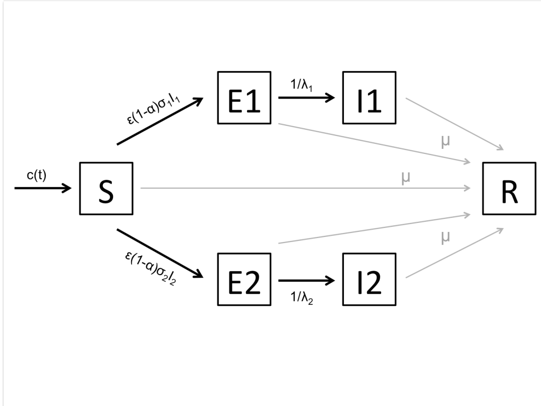
Figure 2: visual representation of the patch dynamics of the disease. Susceptible tissue S represents the canopy green leaf area index. It becomes infected (“exposed”, E ) at a rate proportional to patch spore production \sigma I . Exposed tissue E becomes infectious ( I ) at a rate \lambda corresponding to the pathogen latent period. Both S , E and I tissue become senescent at a rate \mu and are thus “removed” ( R ) from the system. Here, we consider two separate pathogen strain 1 and 2 co-infecting the same patch.
