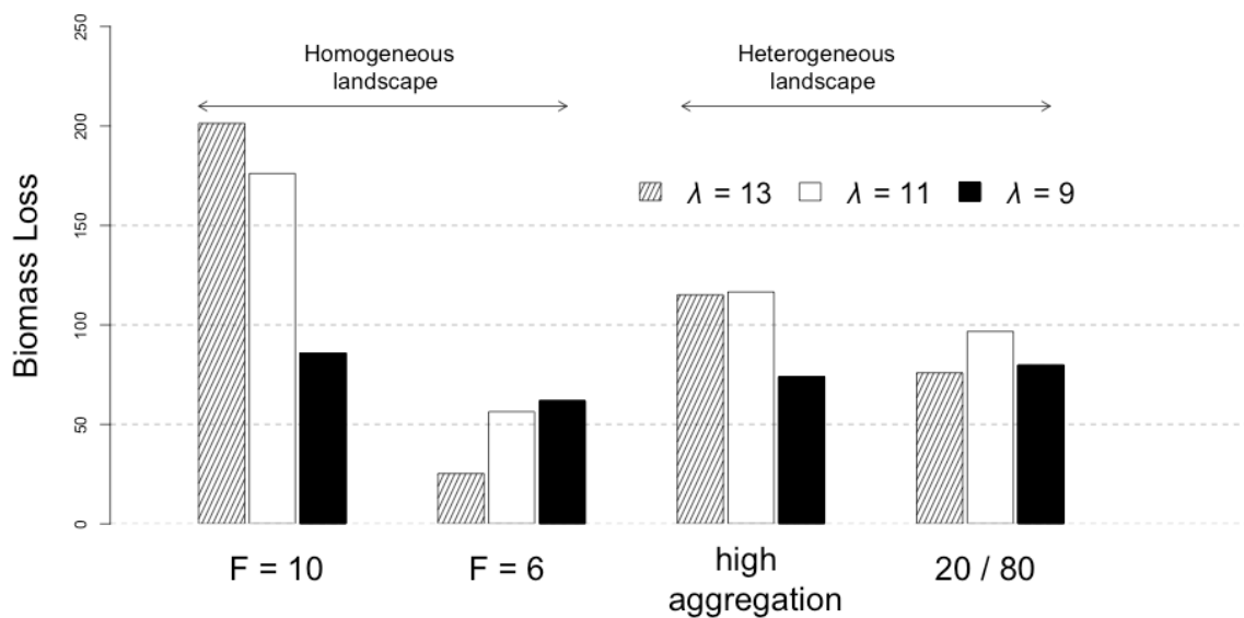
Figure 16: effect of spatial heterogeneity on disease-induced green leaf area reduction for different pathogen strains. Here we compare the reduction of green leaf area in high fertilization ( F = 10 ) and low fertilization ( F = 6 ) homogeneous landscapes, a high aggregation heterogeneous landscape with 50/50 field proportion and a medium aggregation landscape with 20% of high fertilization fields and 80% of low fertilization ones. The first two columns correspond to landscapes colonized by only one pathogen strain, with either \lambda = 130 dd or \lambda = 90 dd.
