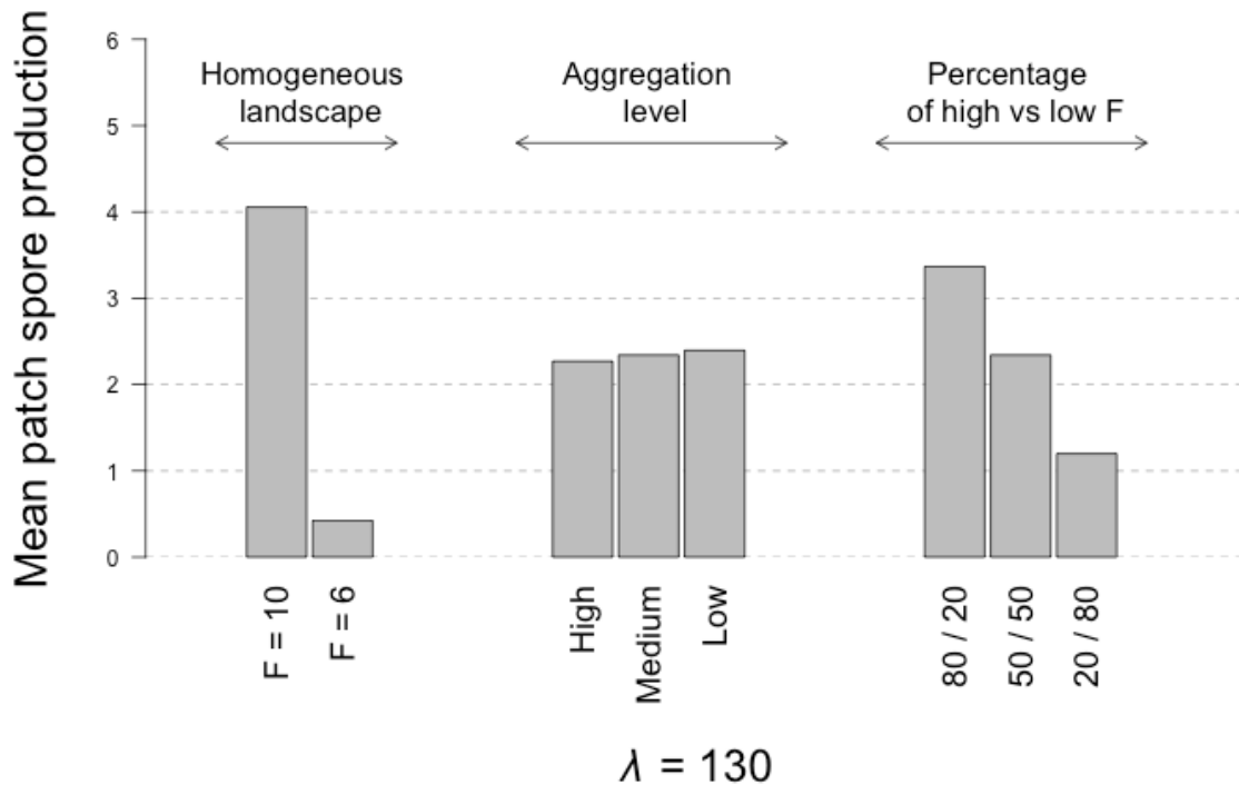
Figure 13: effect of spatial heterogeneity on landscape-scale spore production at equilibrium for \lambda = 130 dd. Here, we compare homogeneous landscapes with high ( F = 10 ) and low ( F = 6 ) fertilization and heterogeneous landscapes with various aggregation levels or various proportions of field types. The aggregation level is the same in landscapes with different field type proportions (medium aggregation) and reciprocally, the proportion of fields of each type is the same in landscapes with different aggregation levels (50/50). \lambda = pathogen latent period; F = fertilization level.
