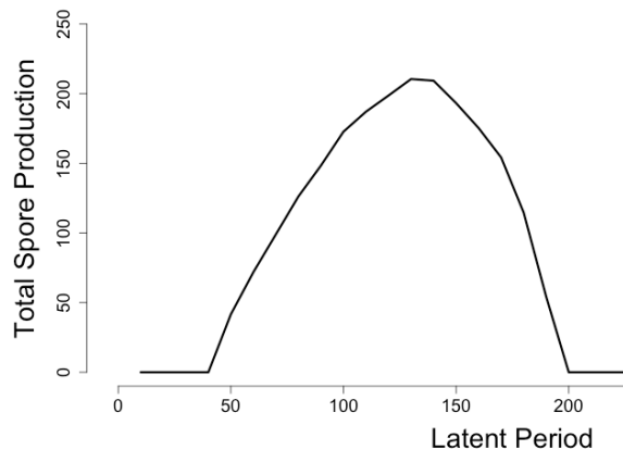
Figure 16. Total spores production at canopy level, over a range of latent periods \lambda .
