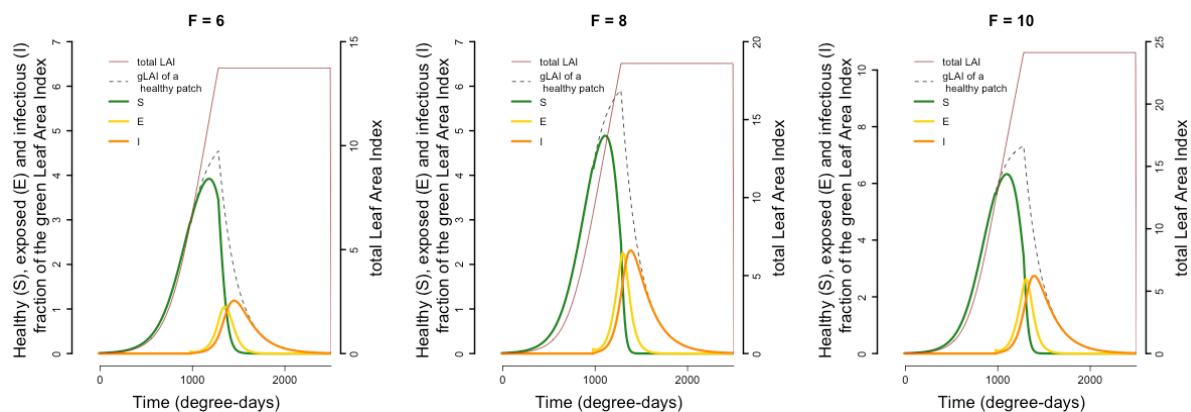
Figure 6: seasonal dynamics of within-field epidemics at equilibrium for three fertilization levels ( F ). Solid lines describe canopy growth and epidemic development: green = susceptible leaf area (green leaf area index, gLAI); yellow = exposed leaf area; orange = sporulating (infectious) leaf area; brown: total leaf area corresponding to the field leaf area index (LAI). Dotted lines indicate the gLAI of a corresponding uninfected field. Fertilization increases from left ( F = 6 ) to right ( F = 10 ). \lambda = 130 dd.
