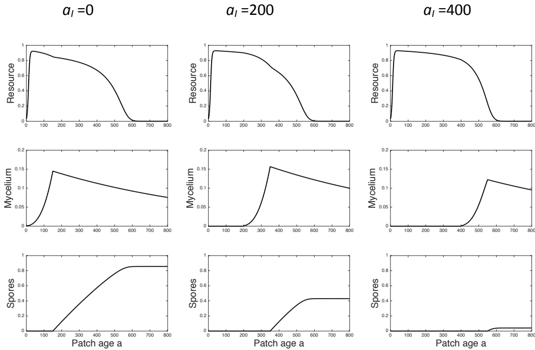
Figure 6. The effect of the age-at-infection on within patch dynamics of resource R , mycelium M and spores production S , representing time series for a given patch. Top: Dynamics of R(a) for a patch becoming infected at patch age a_i = 0, 200, 400 , respectively. Middle: Idem, dynamics of M(a) . Bottom: Idem, dynamics of S(a) . Parameters: \lambda = 100 and see Table 1.
