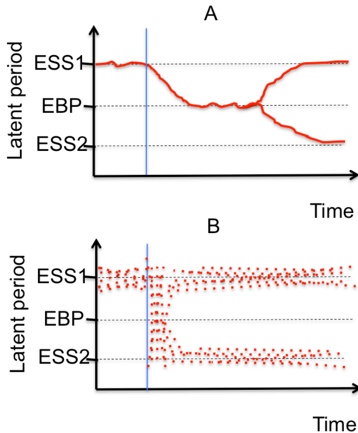
Figure 25: two scenarios of diversification in response to spatial fertilization heterogeneity depending on the size of mutation steps. A: small mutation steps; B: large mutation steps; EBP: evolutionary branching point identified in Figures 20 to 23; ESS1 and ESS2: evolutionary singular strategy identified in high ( F = 10 ) and low ( F = 6 ) fertilization fields in Figure 18.
