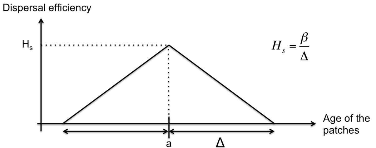
Figure 4: dispersal kernel at the vicinity of patches cohort of age a . \beta is the dispersal efficiency, \Delta the maximum dispersal distance and H_s an area-conservation value. Patches in a cohort of age a receive spores from cohorts of age a \pm \Delta . Dispersal efficiency linearly decreases with distance to reference cohort of age a .
