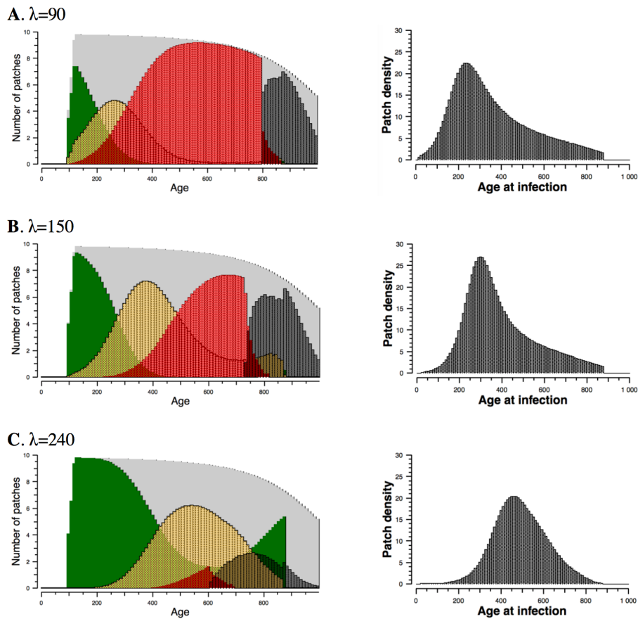
Figure 15. Left column: the canopy age structure of healthy, latent, sporulating and dead infected patches at date T=1600 dd. Right column: the distribution of age at infection ( a_i ) at the end of the season. A: \lambda=90 . B: \lambda=150 . C: \lambda=240 . In A and B the epidemics are stable from year to year whereas it is ephemeral in panel C. Note that A, B and C correspond to Figure 14A, B and C. Parameters: T_{inoc}=1000 , and see Table 1.
