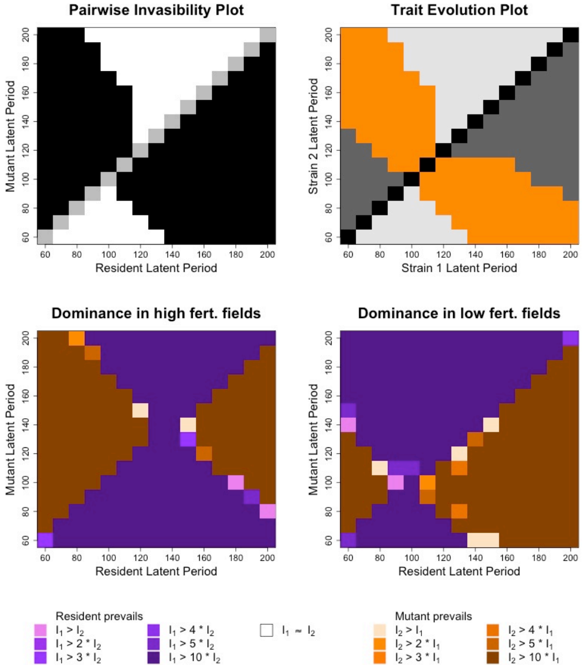
Figure SM3: pairwise invisibility plot (PIP), trait evolution plot (TEP) and dominance plots for a medium aggregation heterogeneous landscape with a 20(F10)/80(F6) percentage of patch types. Top-left: PIP. Black areas correspond to mutant strategies capable to invade the resident population. White areas correspond to mutants that fail in the invasion process. The first diagonal has been highlighted in grey for the sake of clarity. Top right: TEP. Light grey areas correspond to strategies where only strain 1 can invade strain 2. Dark grey areas correspond to strategies where only strain 2 can invade strain 1. Orange areas correspond to strategies allowing for mutual invisibility, that is coexistence in adaptive dynamics. The first diagonal has been highlighted in black for the sake of clarity. Bottom left: dominance in the high fertilization fields of the heterogeneous landscape 100 seasons after the start of the epidemics. Warm colours indicate dominance by the mutant strain. Cold colours indicate dominance by the resident strain. White area indicate even coexistence. Bottom right: dominance in the low fertilization fields of the heterogeneous landscape 100 seasons after the start of the epidemics. The legend is the same for both coexistence plots. In this figure, I_1 and I_2 refer to the AUDPCs of the resident and mutant strains respectively.
