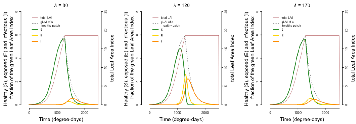
Figure 7: seasonal dynamics of within-field epidemics at equilibrium for three pathogen latent periods ( \lambda ). Solid lines describe canopy growth and epidemic development: green = susceptible leaf area (green leaf area index, gLAI); yellow = exposed leaf area; orange = sporulating (infectious) leaf area; brown: total leaf area corresponding to the field leaf area index (LAI). Dotted lines indicate the gLAI of a corresponding uninfected canopy. Latent period increases from left ( \lambda = 80 dd) to right ( \lambda = 170 dd). Note that the diseased surface is maximal at intermediate latent period as a result of the trade-off between spore production and latent period implemented at the field scale. F = 10 .
