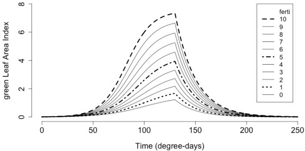
Figure 1: response of the green leaf area index (gLAI) to fertilization in our model. Results are obtained by integrating equation 1 for eleven fertilization levels. Parameter values are given in Table 1.
