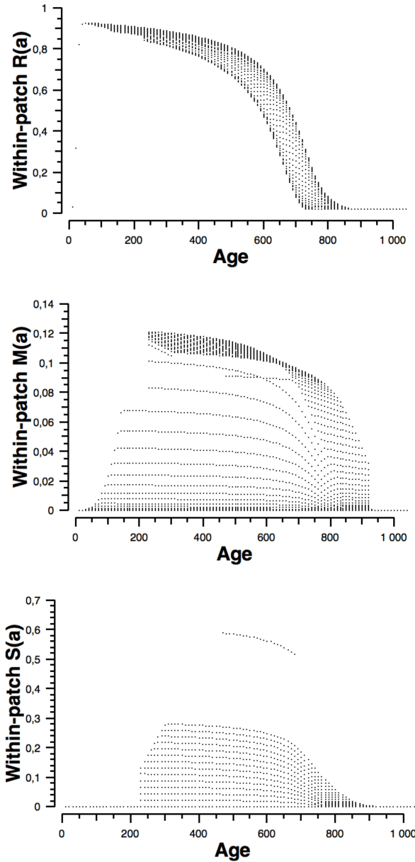
Figure 12: Scatter plots of the patch-level variables R(a) , M(a) and S(a) versus patch age a ( T=1450 dd). Same run as in Figure 9B, 10 and 11.
