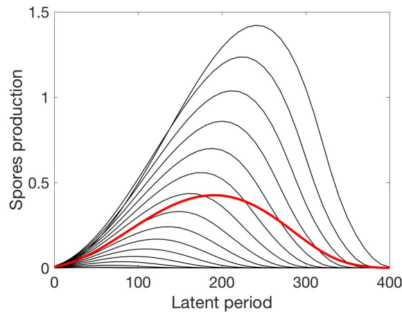
Figure 8: patch-level spore production depending on latent period and age at infection. Black curves: each curve represents a specific age at infection ( a_I=0, 50, 100, \dots ). The upper curve is for a_I=0 . Each subsequent curve represents the data for an infection occurring 50 dd later. Red curve: the mean spores production, averaged over all a_I . See Table 1 for other parameter values.
