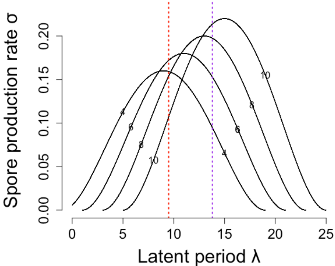
Figure 3: trade-off between latent period and spore production. In accordance with the results of chapters 1 to 3, the spore production rate of the pathogen is maximal at intermediate latent periods. These maximum values increase with fertilization levels. The curves correspond to different fertilization levels ( 4 \leq \mathcal{F} \leq 10 ). For the sake of comparison, vertical dotted lines have been drawn for latent periods corresponding to the ESS of field-scale invasion analysis: red line: \mathcal{F} = 6 ; purple line: \mathcal{F} = 10 (cf. Figure 16)
