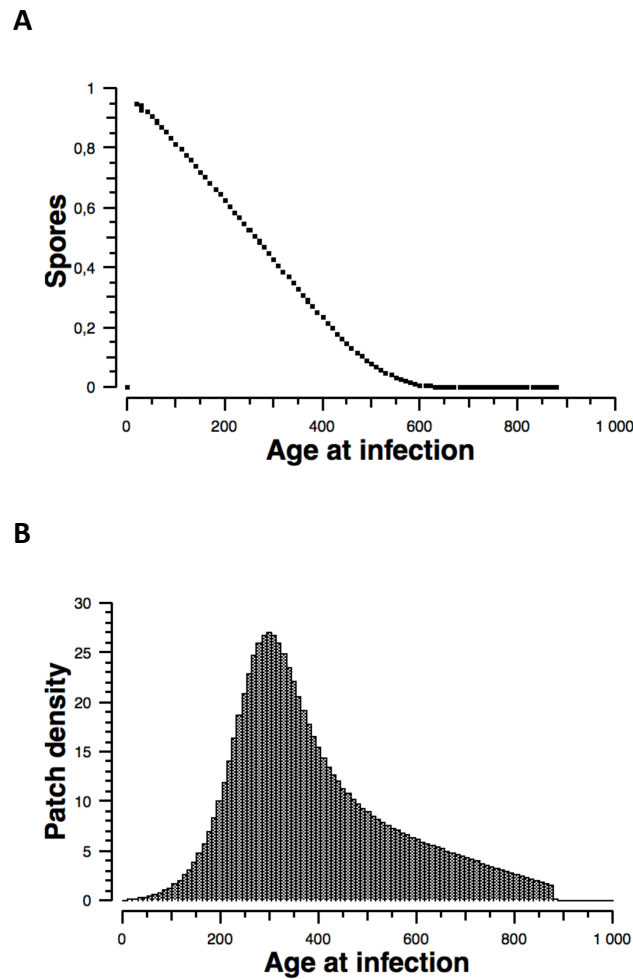
Figure 13. A: The relation between the end-of-season, within-patch cumulative spore production S(T_{\text{season}}) and age at infection for all patches in the population. NB patches with the same age at infection ( a_i ) need not have the same patch age a nor infection age b . (cf Figure 11). B: The distribution of patch age at infection ( a_i ) on the final day in the time series of Figure 9B and Figure 10. The distribution peaks at 300 dd. Parameters: \lambda = 150 , \Delta = 250 and Table 1.
