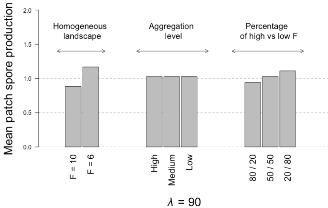
Figure SM1: effect of spatial heterogeneity on landscape-scale spore production at equilibrium for \lambda = 90 dd. Here, we compare homogeneous landscapes with high (F = 10) and low (F = 6) fertilization and heterogeneous landscapes with various aggregation levels or various proportions of field types. The aggregation level is the same in landscapes with different field type proportions (medium aggregation) and reciprocally, the proportion of fields of each type is the same in landscapes with different aggregation levels (50/50). \lambda = pathogen latent period; F = fertilization level.
