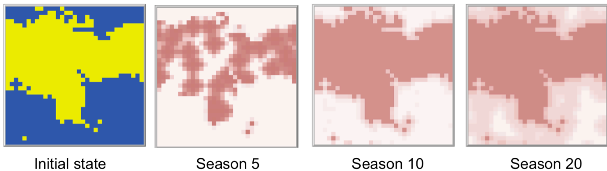
Figure 15: high spatial aggregation in a heterogeneous landscape impedes pathogen development in low fertilization areas. Except for the initial state, the red colour scale corresponds to field-scale spore production and thus represents the intensity of the epidemics: the darker the field, the stronger the epidemic. First panel: initial state. High fertilization fields have been coloured in yellow, low fertilization fields in blue. The aggregation level is 7.2 identical neighbours in average. The whole landscape has been colonized by the pathogen during the first season (data not shown). At the end of the fifth cropping season (Second panel), the pathogen causes consequent epidemics in almost all the high fertilization fields, while epidemics remain limited in low fertilization ones. After 10 seasons (Third panel), all high fertilization fields house strong epidemics. Low fertilization patches at the edge of the high fertilization clusters show a higher spore production than those further from the high fertilization clusters. This “ring” extends towards the centres of the low fertilization clusters (Fourth panel) until the system reaches a steady state.
