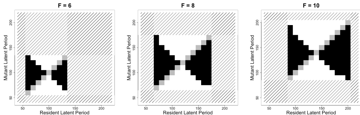
Figure 19: pairwise invisibility plots for three fertilization homogeneous landscapes. From left to right: F = 6 ; F = 8 and F = 10 . Black area correspond to winning mutant strategies while white area correspond to mutants unable to invade the resident population. Similar strategies on the first diagonal have been highlighted in grey for the sake of clarity. Corresponding evolutionary singular strategies are 10, 12 and 14 for fertilization levels 6, 8 and 10 respectively.
