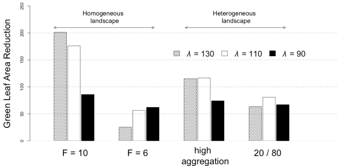
Figure 17: effect of spatial heterogeneity on infected canopy green leaf area index (gLAI) for different pathogen strains. Here we compare per patch average yields in high fertilization ( F = 10 ) and low fertilization ( F = 6 ) homogeneous landscapes, a high aggregation heterogeneous landscape with 50/50 field proportion and a medium aggregation landscape with 20% of high fertilization fields and 80% of low fertilization ones.
