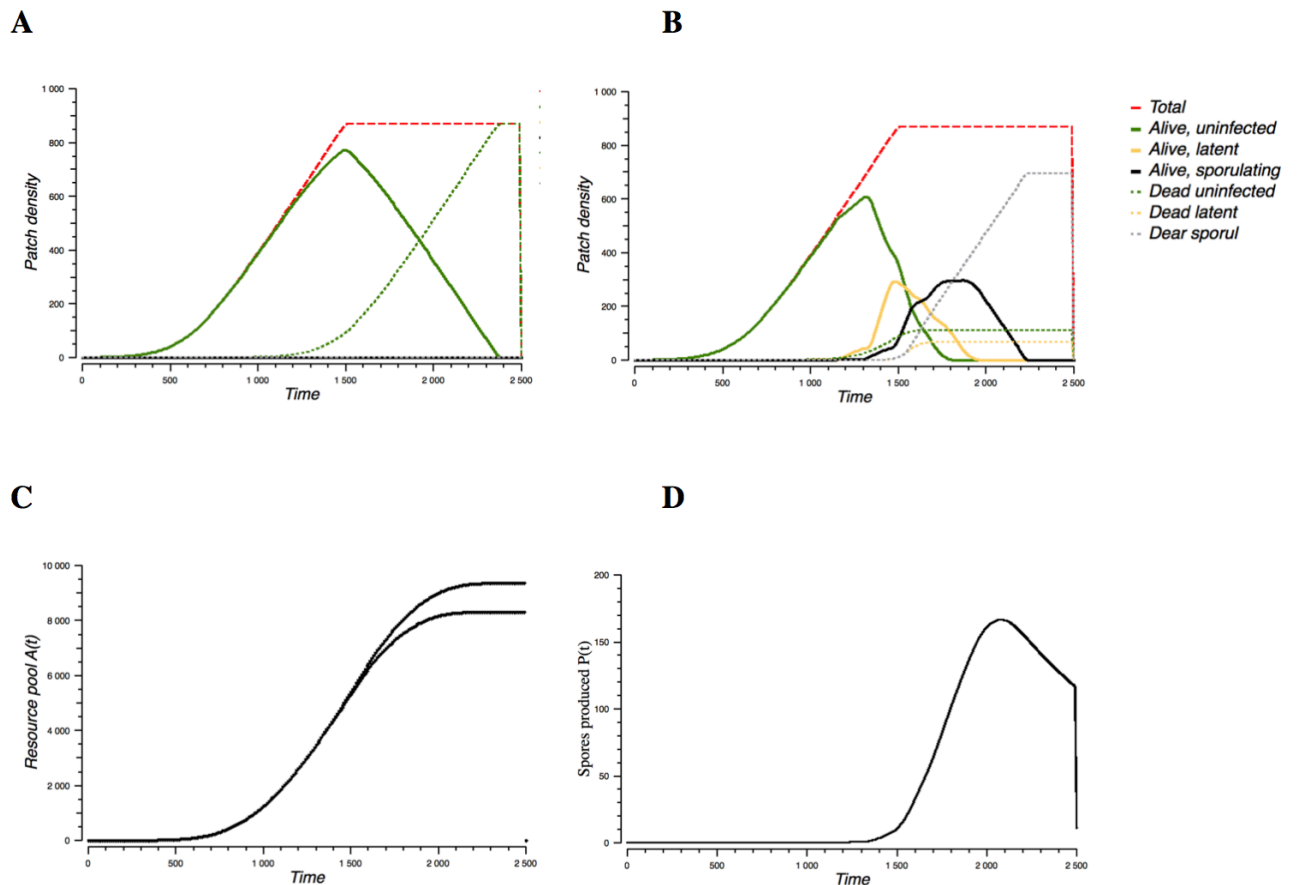
Figure 9: Single-year dynamics of the canopy level model, for a latent period of \lambda = 150 . A: Simulation of canopy without disease, showing the dynamics of healthy, senesced and all patches. B: Simulation of canopy with epidemics, showing the dynamics of healthy, latent and sporulating patches. Inoculum arrives at date T=1000 dd. For dead patches, the curves distinguish between patches according to their status at the onset of their senescence. C: the accumulated resource in the common pool A(t) , for the runs in A (upper curve) and B (lower curve), showing the disease's impact on yield. D: The dynamics of the total spores pool P(t) , for the run in panel B. Parameters: default values in Table 1.
