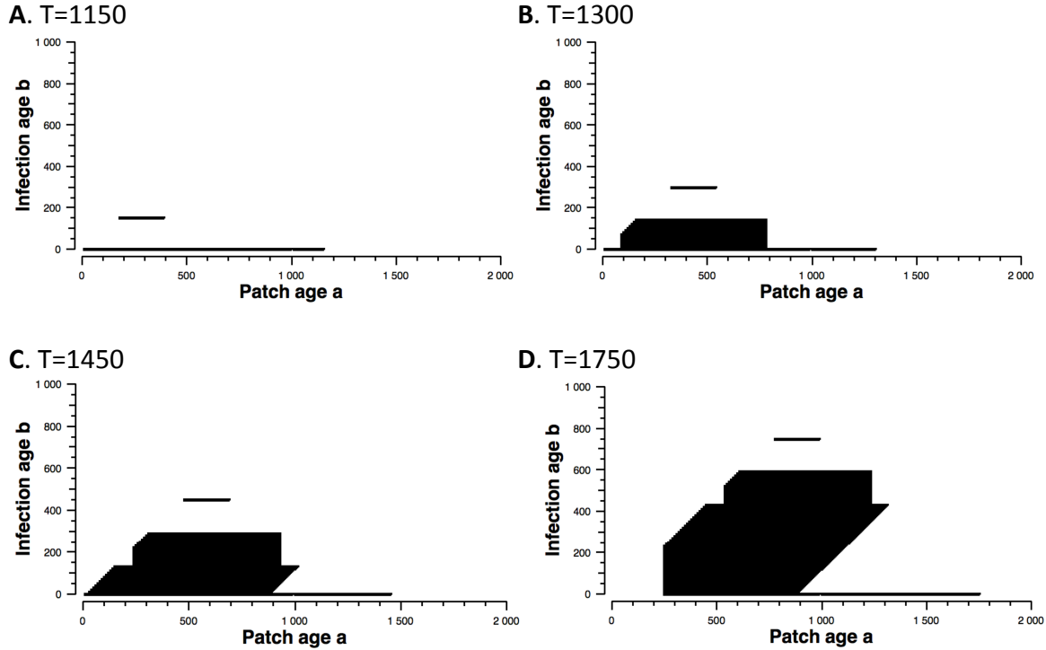
Figure 11. Snapshots of the double age structure of the population, in terms of patch age a , and infection age b , for the same run as in Figs 9B and 10 ( \lambda = 150 ). The black region is made up of discrete dots representing the cohorts that make up the canopy. The number of cohorts k increases over time: at times T=1150 , 1300, 1450, and 1750 dd, the number of cohorts is, respectively: k=140 , 1000, 2188, and 3826. At T=1150 , the horizontal line at b=150 dd corresponds to the primary infections resulting from inoculation at T=1000 . The line at b=0 corresponds to the uninfected population (infection age is arbitrarily set to b=0 ) and span the range a=(0,1150) . At T=1300 the second generation of (still latent) patches is visible as the black area between b=0 and b=150 . At T=1450 this generation is sporulating and a new generation of latent patches is visible. At T=1500 the canopy stops growing and thus by T=1750 no patches younger than a=250 dd exist. The right-hand side limit of the black area results from the assumption that dead patches cannot be infected.
