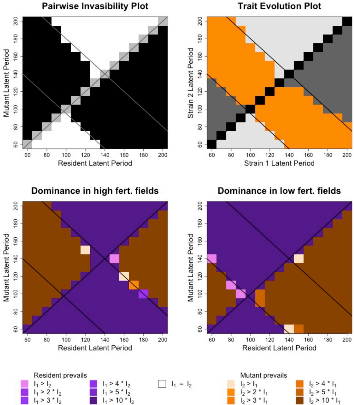
Figure 20: pairwise invisibility plot (PIP), trait evolution plot (TEP) and dominance plots for a high aggregation heterogeneous landscape with a 50/50 percentage of patch types. Top-left: PIP. Black areas correspond to mutant strategies capable to invade the resident population. White areas correspond to mutants that fail in the invasion process. The first diagonal has been highlighted in grey for the sake of clarity. Top right: TEP. Light grey areas correspond to strategies where only strain 1 can invade strain 2. Dark grey areas correspond to strategies where only strain 2 can invade strain 1. Orange areas correspond to strategies allowing for mutual invisibility, that is coexistence in adaptive dynamics. The first diagonal has been highlighted in black for the sake of clarity. Bottom left: dominance in the high fertilization fields of the heterogeneous landscape 100 seasons after the start of the epidemics. Warm colours indicate dominance by the mutant strain. Cold colours indicate dominance by the resident strain. White area indicate even coexistence. Bottom right: dominance in the low fertilization fields of the heterogeneous landscape 100 seasons after the start of the epidemics. The legend is the same for both coexistence plots. In this figure, I_1 and I_2 refer to the AUDPCs of the resident and mutant strains respectively. The first diagonal and the zero isoclines from field-scale PIPs ( F = 6 and F = 10 ) have been superimposed as solid grey or black lines on all subplots for the sake of interpretation.
