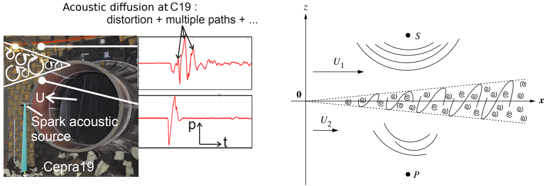
Figure 1 – Anechoic wind tunnel with open-jet test section (nozzle exit \varnothing = 2\text{-}3\text{ m} , U_1 \leq 100\text{ m/s} ); the configuration at CEPR19 [50] (left) and a sketch of the experiment (right).
