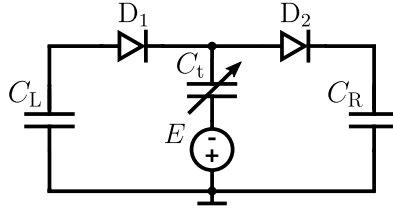
Figure 4.2: Schematic of the charge-pump conditioning circuit proposed by Roundy et al.
