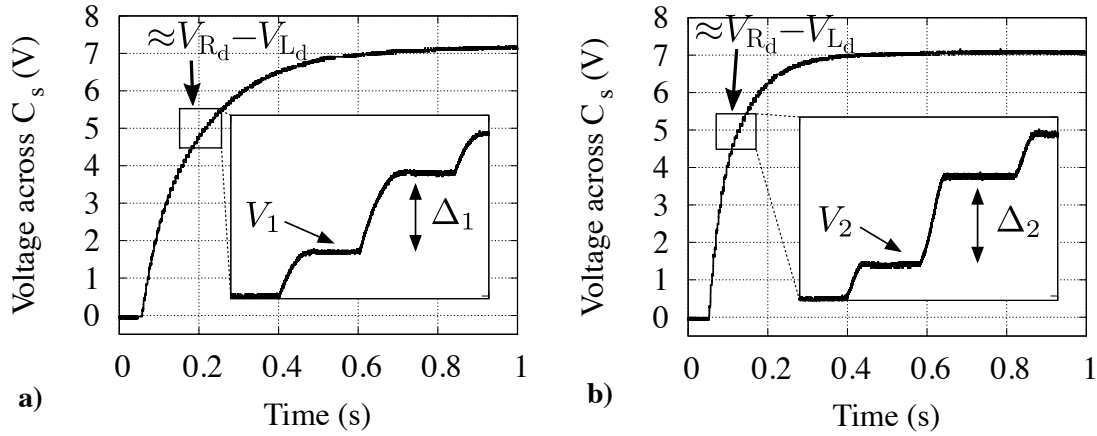
Figure 5.8: Experimental measurement of (\Delta_1, \Delta_2, V_1, V_2) , measured on the MEMS electret transducer characterized in section 5.3.4 and reported in [LOC16].
