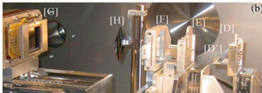
Figure 4-1: a) Illustration of the pump probe configuration used in the resonant small angle X-ray scattering experiment at DiProI. Positive and negative scattering orders recorded at the Co M_3 edge give rise to the intense spots on the CCD camera. b) Photo of the experimental setup inside the DiProI vacuum chamber (from Ref [6]). The beam pass through the aperture
