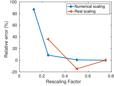
(d) \langle D_h \rangle with respect to RF = 0.75 at Pe = 16.5
