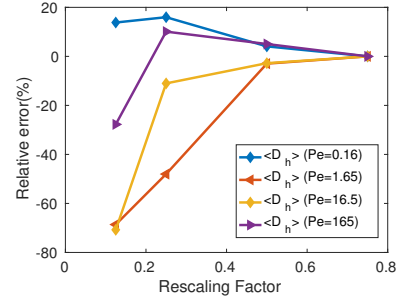
(f) \langle D_h \rangle with respect to RF = 0.75 only numerical scaling cases
