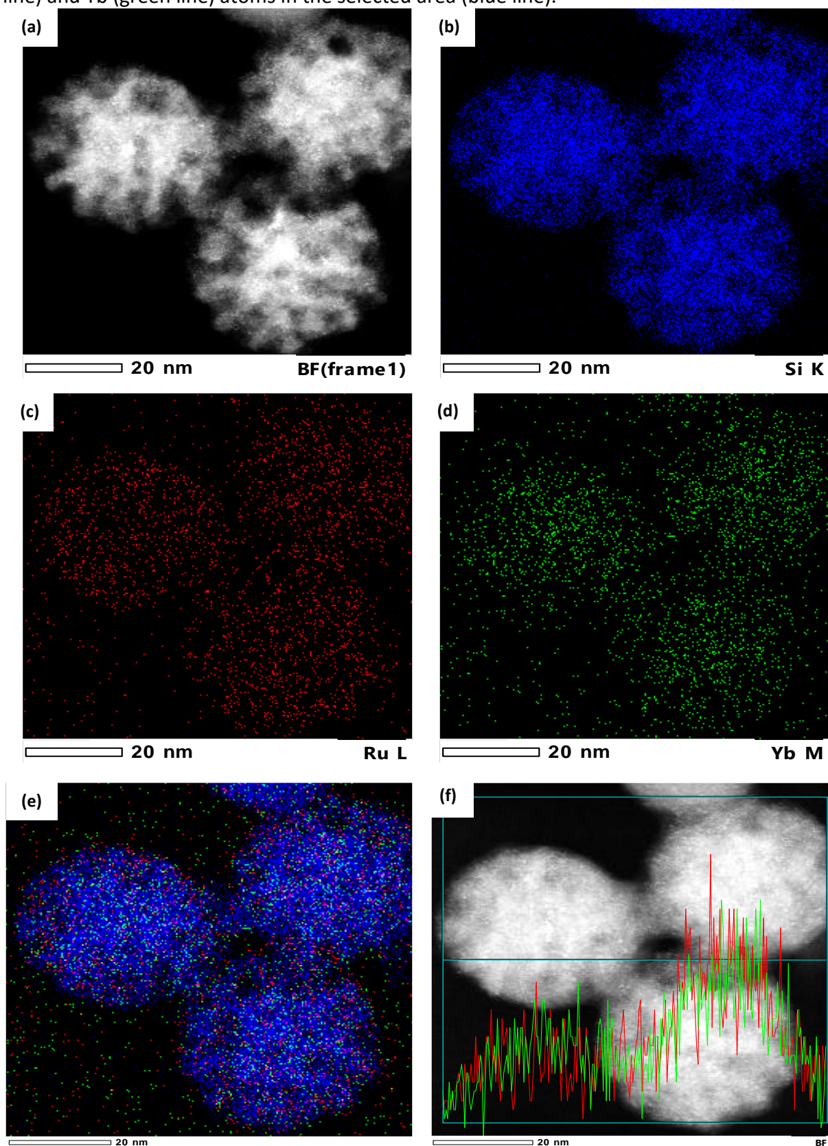
Figure 95. Electron microscope images and elemental cartography of the \text{SiO}_2\text{-YbRuL} : (a) STEM image, (b) Si cartography, (c) Ru cartography, (d) Yb cartography, (e) Si (blue color), Ru (red color) and Yb (green color) cartographies. (f) STEM image with a line profile of Ru (red line) and Yb (green line) atoms in the selected area (blue line).
