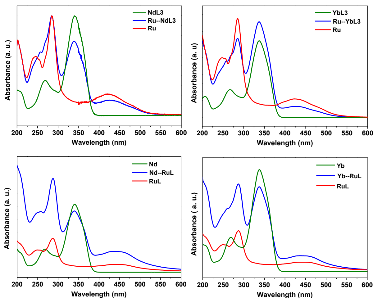
Figure 49. Absorption spectra ( 2,5 \times 10^{-5} mol/L, ethanol) of (a) NdL3 (green line), Ru—NdL3 (blue line), Ru (red line); (b) YbL3 (green line), Ru—YbL3 (blue line), Ru (red line); (c) Nd (green line), Nd—RuL (blue line), RuL (red line) and (d) Yb (green line), Yb—RuL (blue line), RuL (red line).
