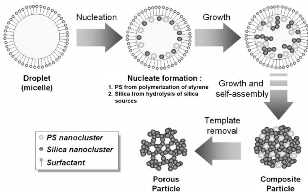
Figure 18. Representation of synthetic route of the mesoporous silica nanoparticles (MSNs). 78 Reference: Adapted from Nandiyanto et al. (2019a) with permission. Copyright 2009 Elsevier n°3898390718024.
