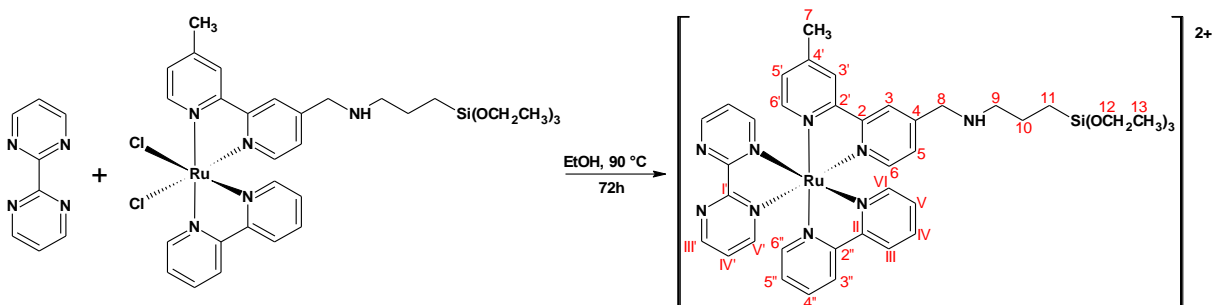
Figure 11. Synthetic route of the [\text{Ru}(\text{bpy})(\text{bpy-Si})(\text{bpmd})]\text{Cl}_2 silylated complex ( RuL ).
