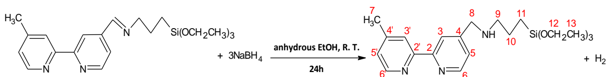
Figure 7. Synthetic route of the 4-methyl-4'-(n-triethoxysilylpropyl)amine-methyl-2,2'-bipyridine ligand ( bpy-Si ).
