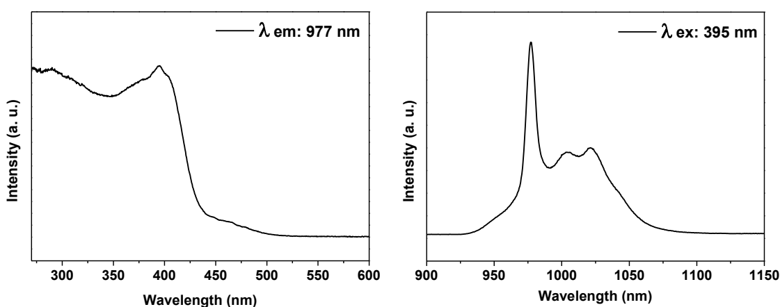
Figure 54. Room temperature excitation (on the left, monitoring at \lambda_{\text{emission}} = 977 \text{ nm} ) and emission (on the right, monitoring at \lambda_{\text{excitation}} = 395 \text{ nm} ) spectra of the Yb complex in solid state.
