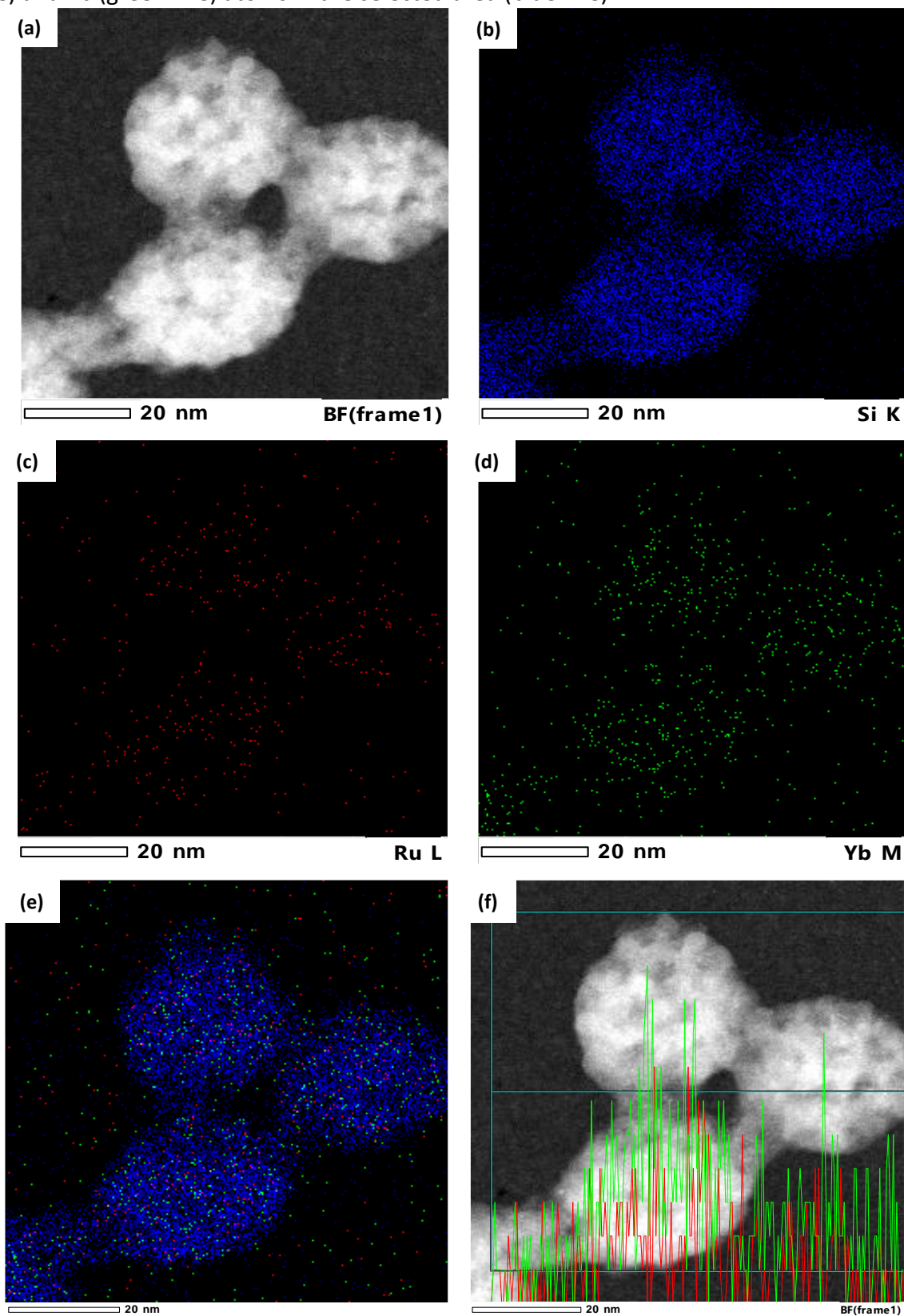
Figure 93. Electron microscope images and elemental cartography of the \text{SiO}_2\text{-RuYbL3} : (a) STEM image, (b) Si cartography, (c) Ru cartography, (d) Yb cartography, (e) Si (blue color), Ru (red color) and Yb (green color) cartographies. (f) STEM image with a line profile of Ru (red line) and Yb (green line) atoms in the selected area (blue line).
