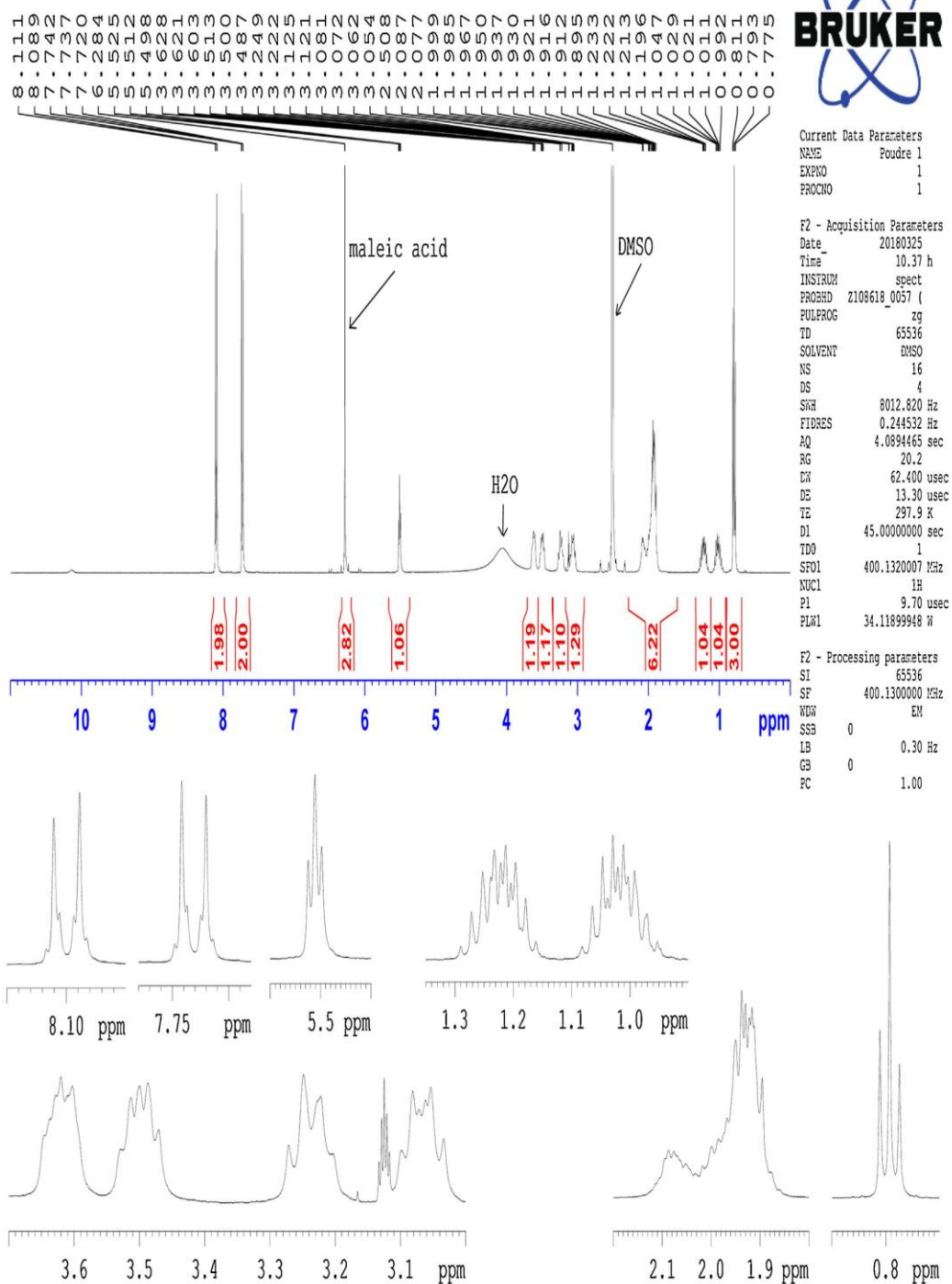
Fig. 2. (A–G) Responses of the 7 powders (1H spectra). (A) 4-Chloro- \alpha -pyrrolidinopentiophenone, (B) dibutylone, (C) 4-chloroethcathinone, (D) 4- \alpha -pyrrolidinohexuiphenone, (E) 3,4-methylenedioxy- N -benzylcathinone, (F) 3-methoxy- p .
