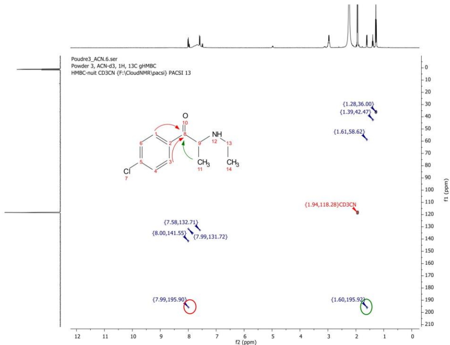
Figure 21 - 1 H, 13 C gHMBC of powder 3 in Acetonitrile-d 3 .
