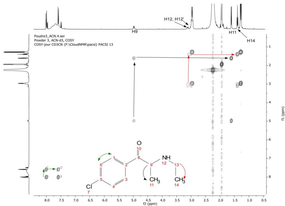
Figure 19 - ^1\text{H} gCOSY spectrum of powder 3 in acetonitrile- d_3
