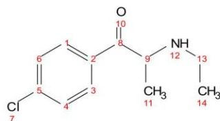
Figure 22 - Structure of 4-CEC
