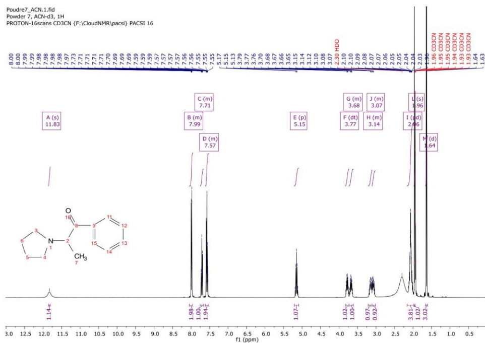
Figure 50 - 1 H NMR spectrum of powder 7 in acetonitrile-d 3 .
