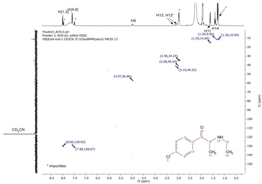
Figure 20 - 1 H, 13 C edited gHSQC of powder 3 in acetonitrile-d 3 .
