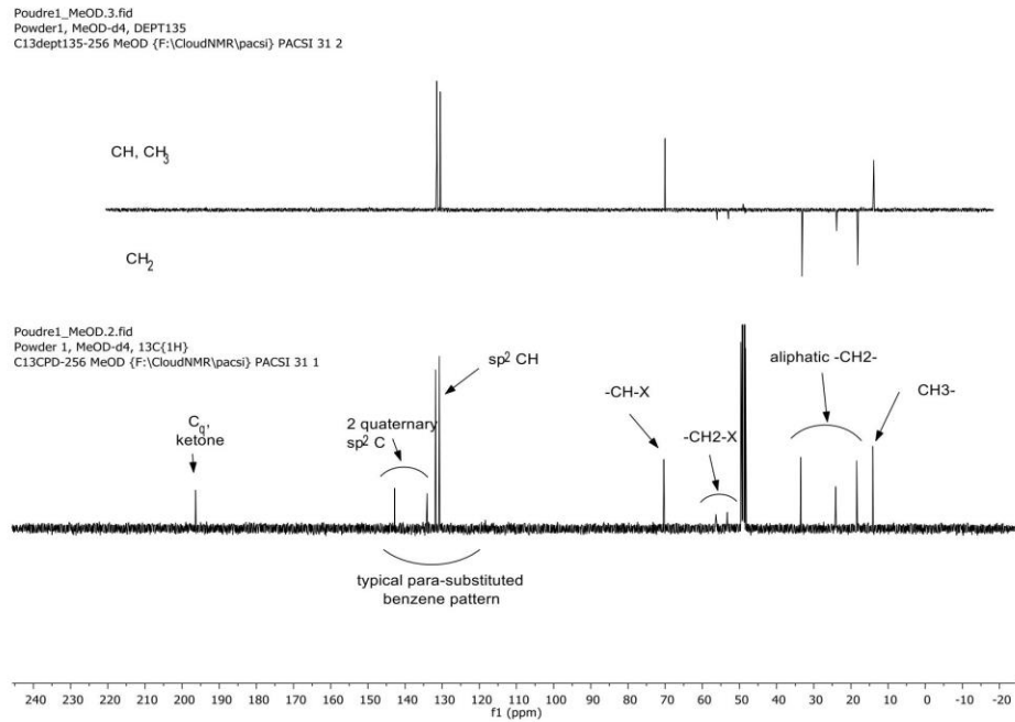
Figure 6 - Superimposed annotated 13 C{ 1 H} and DEPT135 spectra of powder 1 in MeOD-d 4 . X stands for electronegative atom. Please note that quaternary C are not visible in DEPT135.
