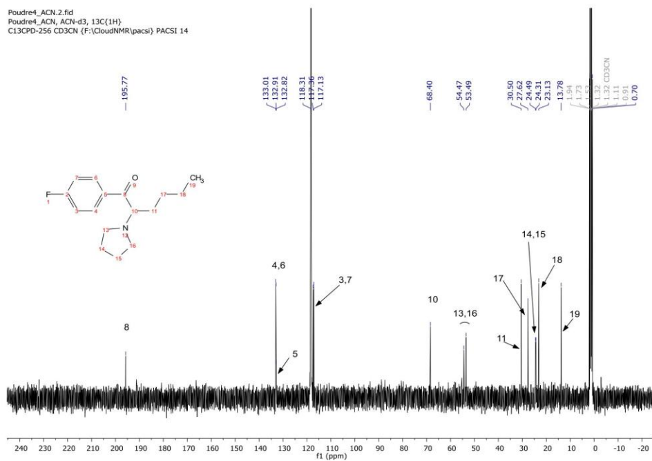
Figure 25 - ^{13}\text{C}\{^1\text{H}\} NMR spectrum of powder 4 in acetonitrile- d_3
