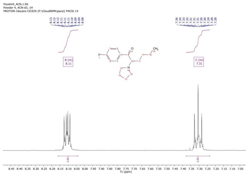
Figure 24 - Zoom on the 8.5–7.0 ppm region of the ^1\text{H} NMR spectrum of powder 4 in acetonitrile- d_3 .
