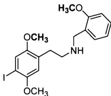
Figure 1. Chemical structure of 25I-NBOMe.
