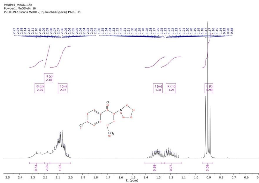
Figure 4 - Zoom of the lower frequency part of the aliphatic region of the ^1\text{H} spectrum of powder 1 in \text{MeOD-d}_4
