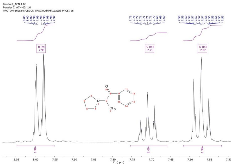
Figure 51 - Zoom on the aromatic region of the 1 H NMR spectrum of powder 7 in acetonitrile-d 3 .
