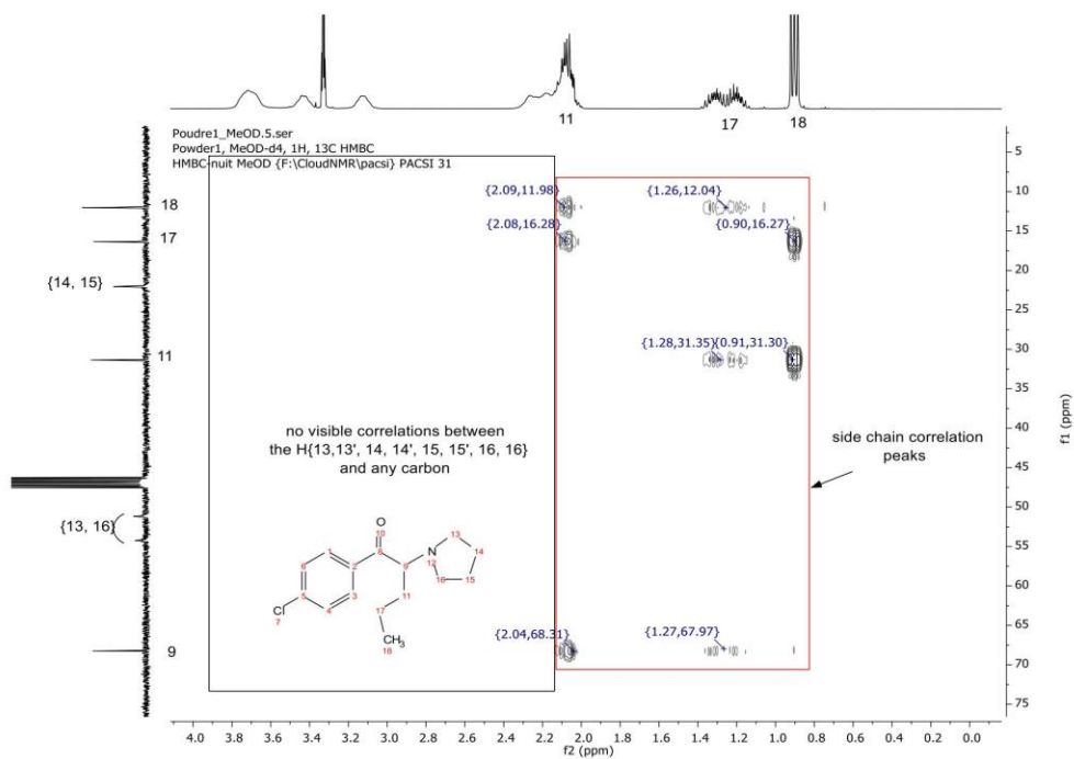
Figure 9 - Zoom of the ^1\text{H} , ^{13}\text{C} gHMBC spectrum of powder 1 in MeOD- d_4 .
