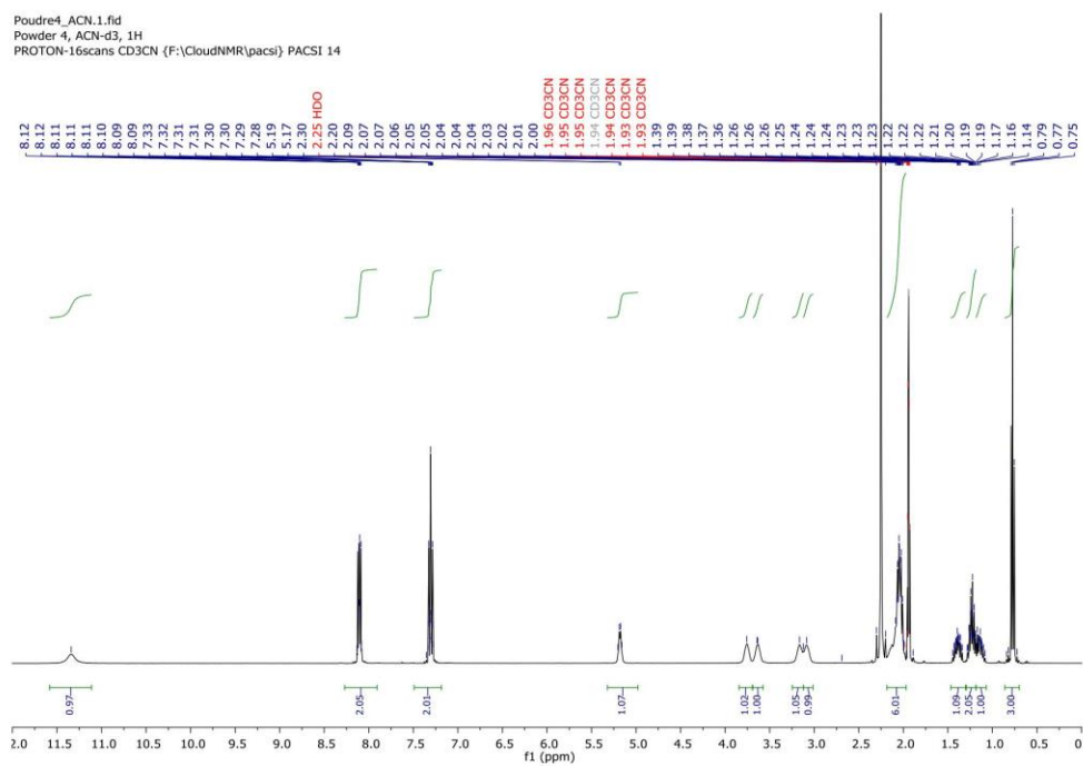
Figure 23 - 1 H NMR spectrum of powder 4 in acetonitrile- d 3 .
