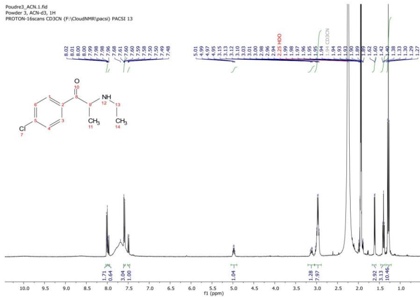
Figure 18 - ^1\text{H} NMR spectrum of powder 3 in Acetonitrile- d_3
