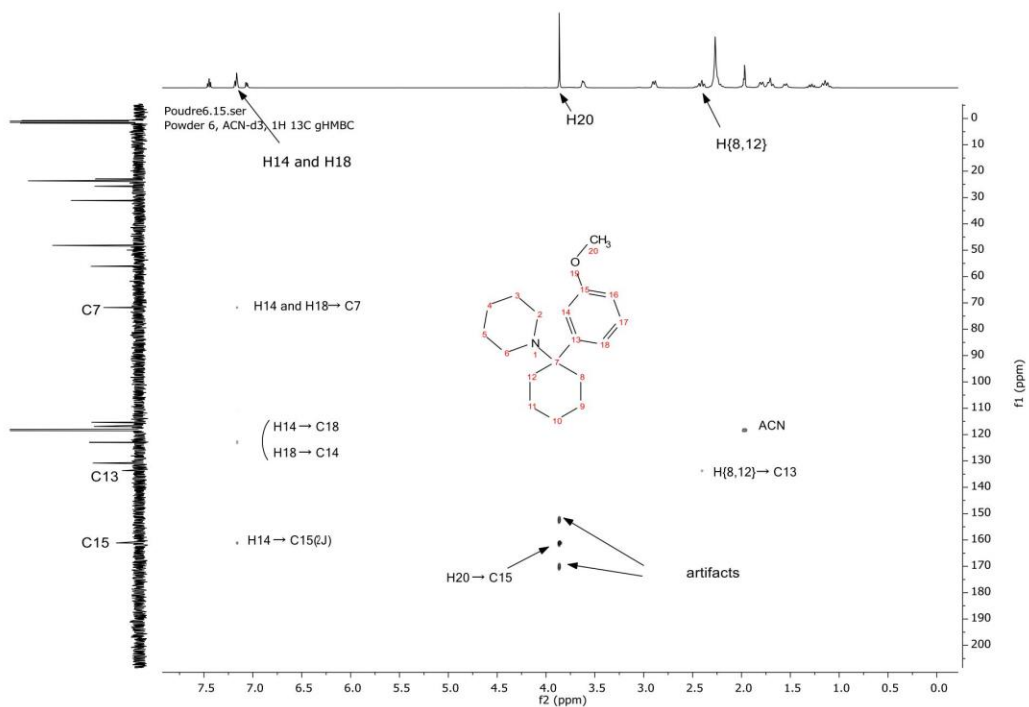
Figure 44 - ^1\text{H} , ^{13}\text{C} gHMBC of powder 6 in acetonitrile- d_3 .
