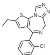
Figure 1. Chemical structure of metizolam.
