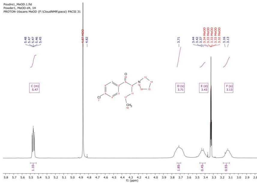
Figure 3 - Zoom of the higher frequency part of the aliphatic region of the ^1\text{H} spectrum of powder 1 in \text{MeOD-d}_4
