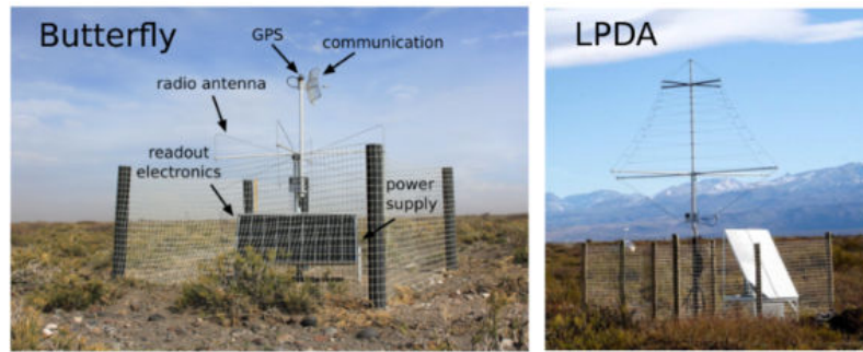
Figure 3.23 – Photography of radio antennas at AERA [131].
