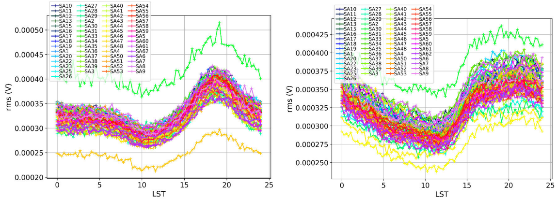
Figure 5.3 – The \langle \text{RMS} \rangle of the 1W data in Local Sidereal Time (LST) for the EW (left) and NS (right) polarizations at 50 MHz (sub-bands of 10 MHz width) and for an arbitrary month. For each LST bin, the \langle \text{RMS} \rangle is calculated from the distribution of the RMS values of the background noise. Outliers in green and yellow are antennas with an electrical problem and come out of the range. However, we will see that this type of behavior is perfectly regulated by the proposed calibration.
