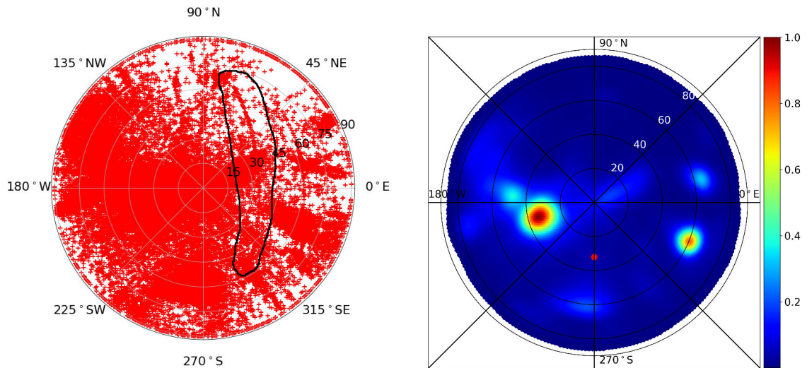
Figure 6.2 – Left: Sky map of events accepted by the central DAQ. The reconstructed direction of arrivals are represented by the red crosses. The azimuth angle is indicated on the outskirts of the circle, the zenith angle is indicated inside the circle. The North is oriented with the geographical North (top). Two plane trajectories are visible, corresponding to the curved trajectories formed by the succession of the reconstructed direction of arrivals. One of them is surrounded in black. Right: same as left, 10^\circ gaussian smoothed sky map.
