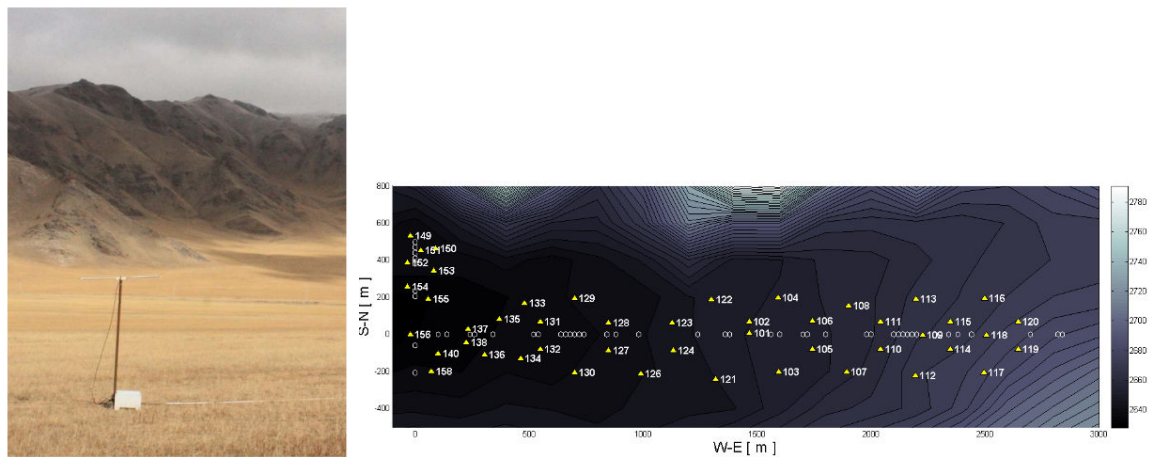
Figure 3.26 – Left: photo of one radio antenna at TREND. Right: TREND layout [143]. The ground extension is ~ 2.7 km for easting and ~ 0.8 km for northing.
