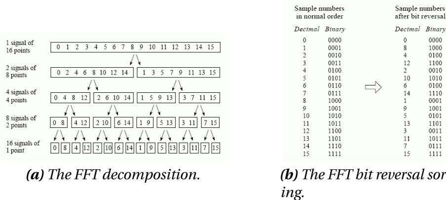
Figure A.1 – The FFT procedure [259].
