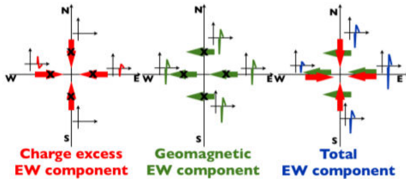
Figure 3.7 – Interferences of the two main mechanisms: depending on the observer location (represented by the black crosses), the interferences can be destructive or constructive, giving an asymmetric total electric field. The orientation of the measured electric field in the EW polarization at ground level is represented for four antennas at different positions but equivalent distance from the shower axis: left for the charge excess mechanism, center for the geomagnetic mechanism and right for the summation of the two mechanisms. Taken from [84].
