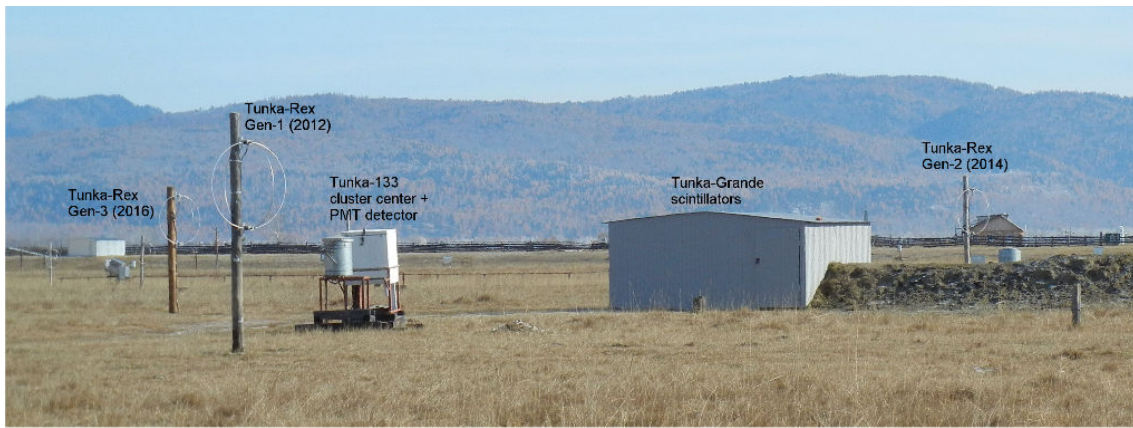
Figure 3.25 – Photo of one cluster center at Tunka, with three antenna stations, a particle-detector station and underground scintillators, and a photomultiplier detector [137].
