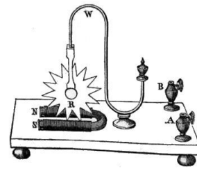
Figure 1.10 – Barlow's wheel.
