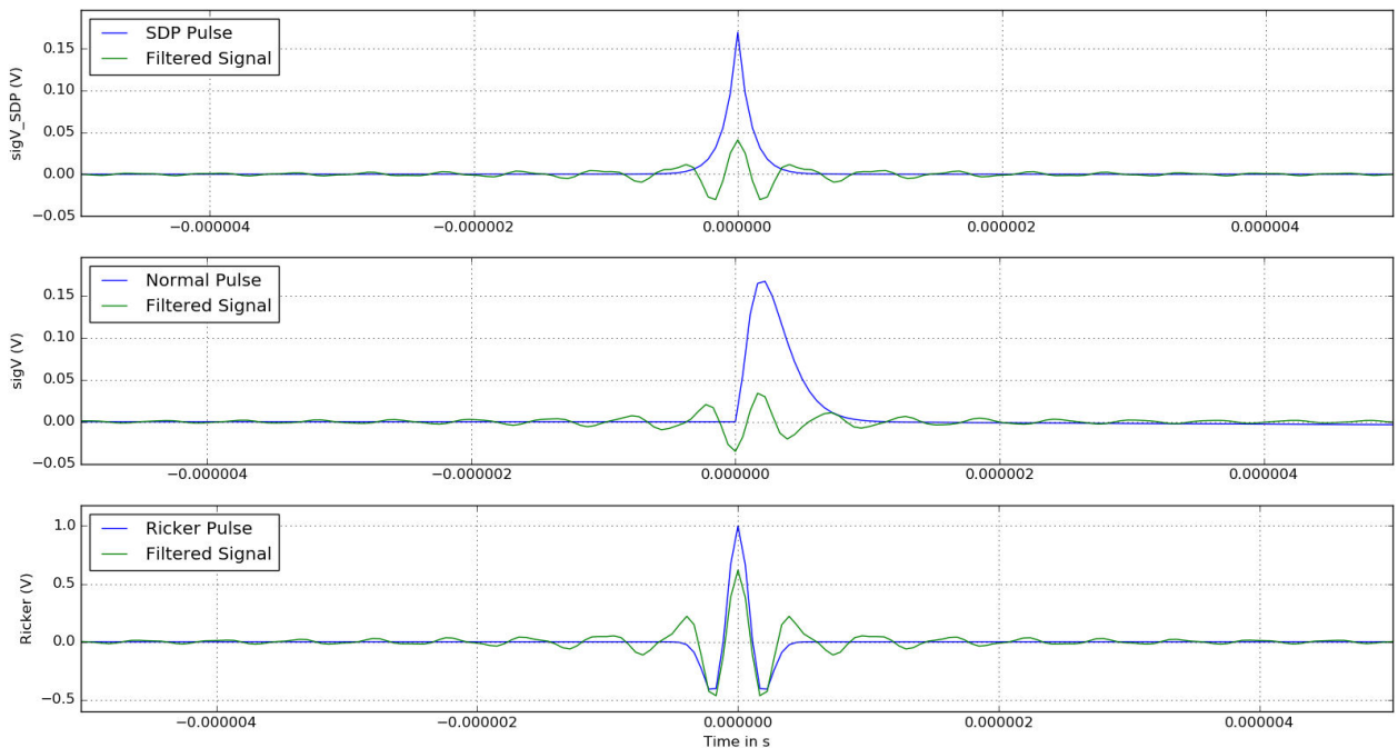
Figure A.3 – Filtered simulated pulses (see text for explanations).
