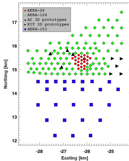
Figure 3.22 – Map of the AERA experiment, with the different deployment stages [71]. The red circles represent the LPDA antennas. The green diamonds represent the Butterfly antennas externally and internally triggered, the blue squares represent the Butterfly antennas only internally triggered.
