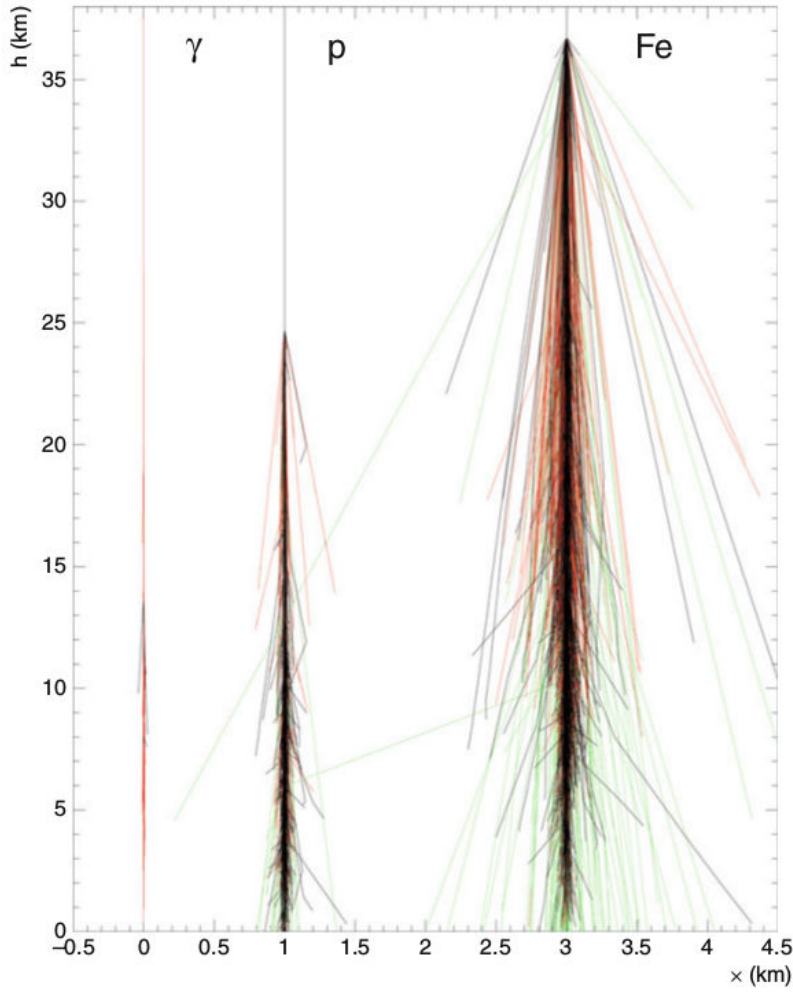
Figure 2.4 – Extensive air shower development for different primary cosmic rays. The three primaries are simulated with an energy of 10^5 GeV. Red component is for electromagnetic, green component for muons and black for hadrons. Adapted from [58].
