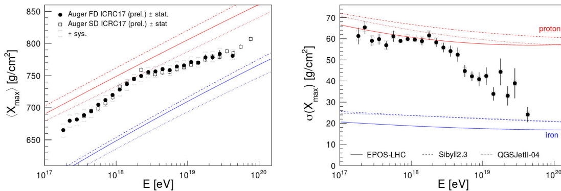
Figure 3.1 – Left: measurement of \langle X_{\max} \rangle as a function of energy by the Pierre Auger Observatory. Red and blue lines represent air-shower simulations of \langle X_{\max} \rangle for proton and iron primaries. Right: its standard deviation. Taken from [18].
