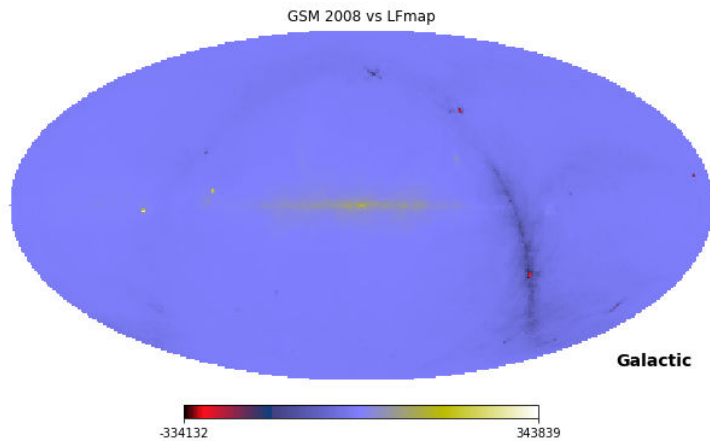
Figure 5.5 – Skymap of differences in Kelvin in galactic coordinates between GSM 2008 and LFmap.
