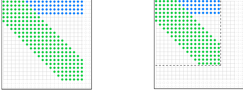
(a) Almost-banded structure of operator \mathbf{K} .
