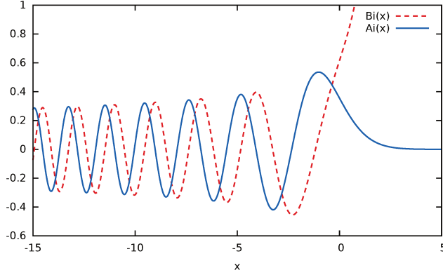
■ Figure 4.3: Airy functions of the first and second kinds
