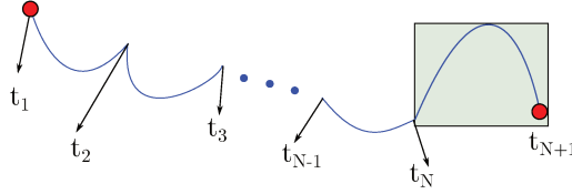
■ Figure 7.3: Steering into the hovering region within N velocity corrections
