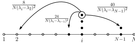
Figure 2.1: Example of the symmetric eigenvector moment flow with a configuration of 7 particles.
