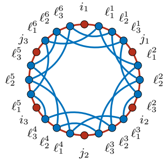
(b) Lower order graph for k = q = 3
