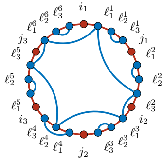
(a) Leading order graph for k = q = 3
