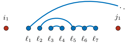
Figure 2.4: Niche where the induced graph is not a perfect matching which raises a fourth moment in the case where k = 7
