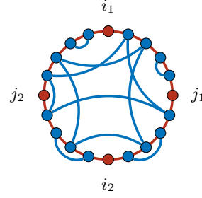
(b) Leading order graph after centering.
