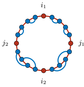
(a) Leading order graph before centering
