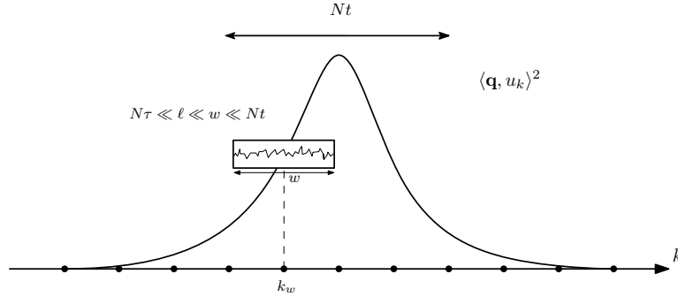
Figure 2.3: We see here a sketch of the variance profile plotted in the spectral dimension: the projection \mathbf{q} is fixed and we plot the profile as a function of the eigenvector u_k . We then localize the dynamics onto the small window plotted here: the window is small enough so that the eigenvector can be seen as "flat" but large enough so that the short-range dynamics will not involve indices outside of this window.
