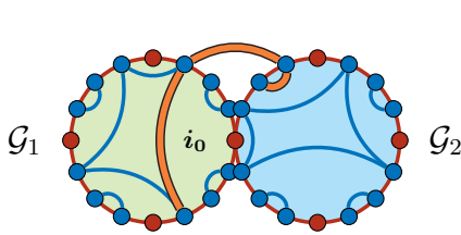
(a) In this figure, the two highlighted cycles correspond to the graph \mathcal{G}_1 and \mathcal{G}_2 which are attached to a common vertex i_0 . We perform a typical blue matching in each graph and then add an identification between the two graphs. The highlighted edges in orange corresponds the common edges between the two graphs which raise a moment of order 4.
