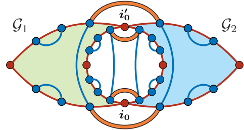
(b) In this figure, the two highlighted cycles correspond to the graph \mathcal{G}_1 and \mathcal{G}_2 which are attached to two vertices i_0 and i'_0 . The graph is non-admissible and we choose the fundamental cycles so that neither \mathcal{G}_1 or \mathcal{G}_2 are fundamental cycles. The typical matching in the chosen cycles create common edges between the two graphs highlighted in orange in the figure. Note that in this case we do not obtain moments of order 4.
