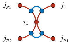
Figure 2.6: Subleading blue identifications around an i -identification
