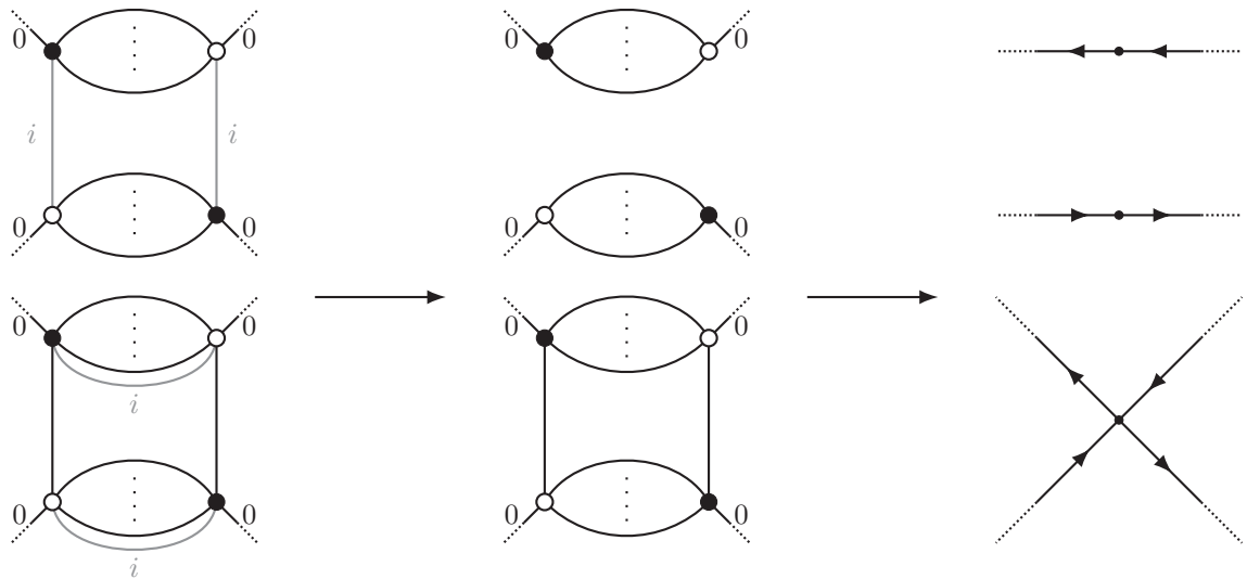
Figure 6.3.3 – Going from Q_p^D to (Q_p^D)_i , and from (Q_p^D)_i to S_p^{D,i} .
