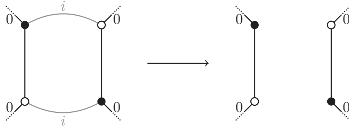
Figure 6.3.2 – Removing a color other than 0 in Q_p^2 .
