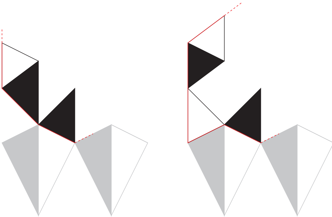
Figure 8.3.5 – There are cases where the boundary of \mathcal{B}_r^\bullet(\mathcal{U}) (depicted in red) has defects (depicted by red stars) in the alternation of colors, at the vertex where the two portions of the boundary meet.
