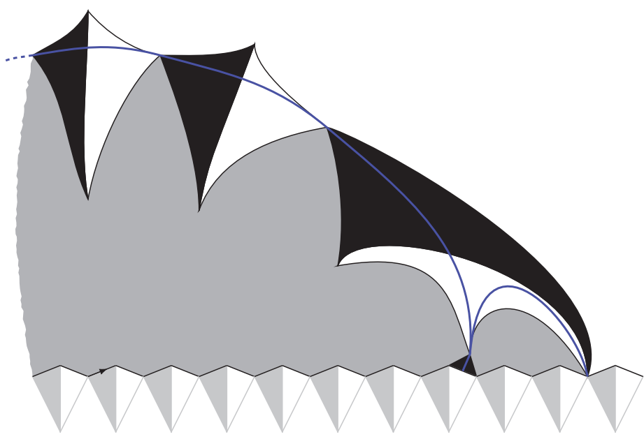
Figure 8.3.10 – Top-bottom identifications on the boundary of \mathcal{U} \setminus \mathcal{B}_r^*(\mathcal{U}) are allowed when r \equiv 2 \pmod{3} , since in that case there is no contradiction.
