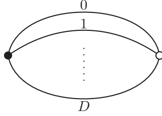
Figure 4.2.1 – Supermelons are the simplest example of colored graphs.
