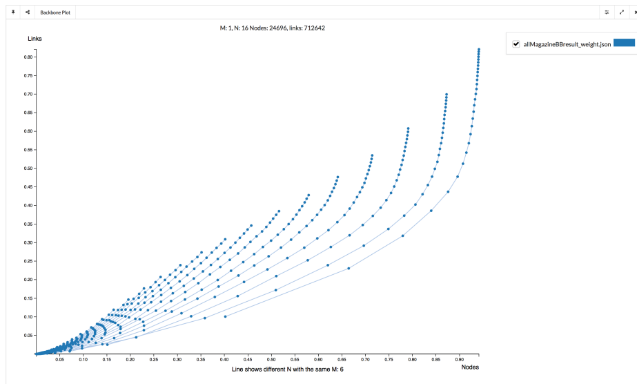
Fig. 5.6 All dots with same N value are connected in turn
