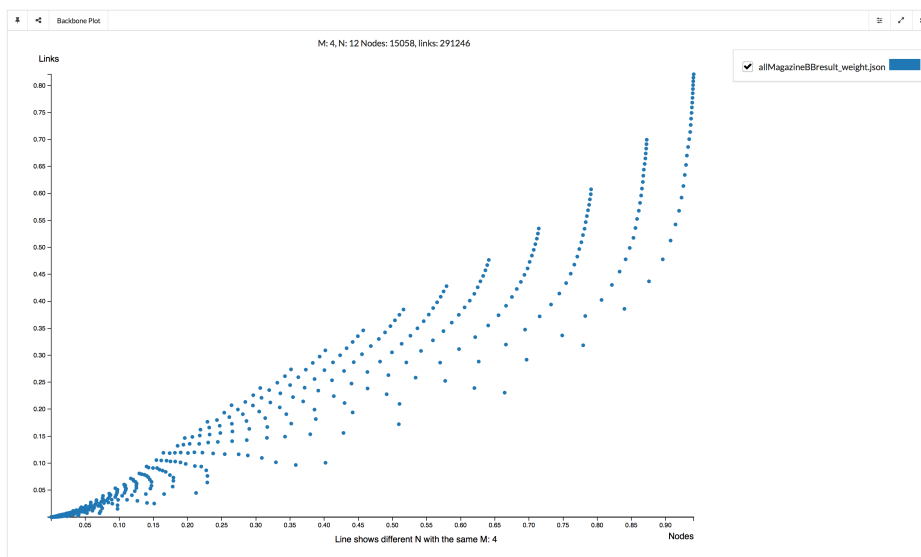
Fig. 5.2 The plot of different results from different Simmelian backbone parameters. Each node correspond to different parameter pairs of m and n
