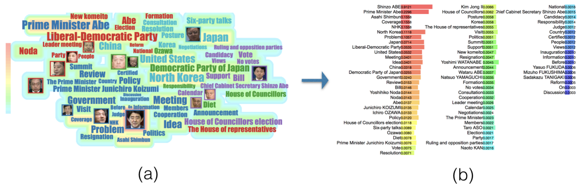
Fig. 3.15 An optional list of concepts view could be displayed. Concepts are ordered by its entanglement index, the bar after each concept represent their degree in the graph, their color is the color of their heat in heat-map which is based on their entanglement index.
