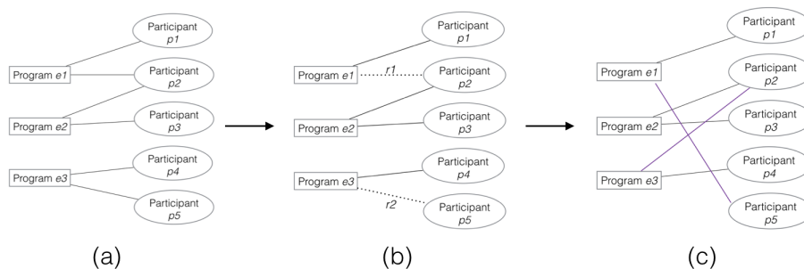
Fig. 5.7 A random process of participating guests in the program.
