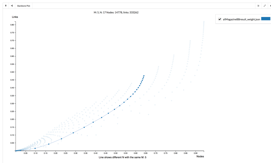
Fig. 5.3 Dots with same m = 5 are connected in turn
