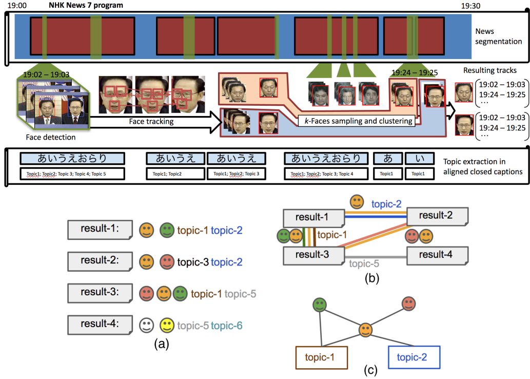
Fig. 3.1 (Top) Indexing each video segment: closed captions-based segmentation, face tracking, and keyword extraction. (Bottom) Abstraction of the search results; (a) indexed video segments; (b) the multiplex network of results; (c) the associated LIN .
