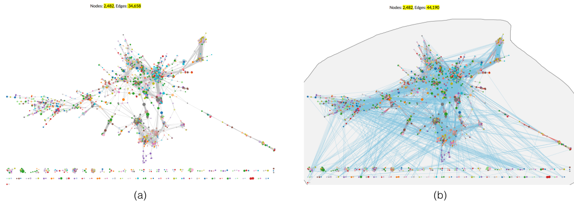
Fig. 4.13 The figures show the hidden edges, (a) is the graph user observed, (b) shows the actual graph data, the blue edge is edge filtered by Simmelian method, we add it to the graph again, it do not participant in the display, but only in the actual calculation.
