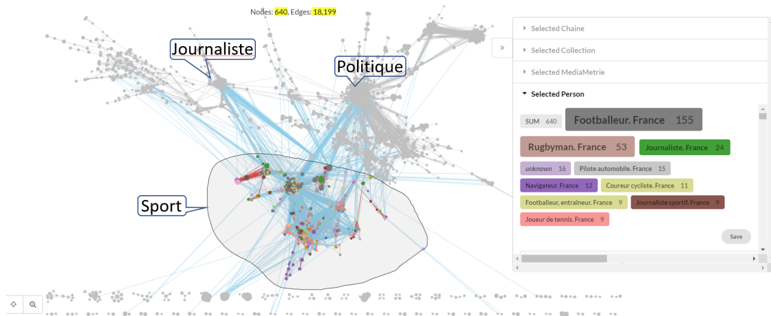
Fig. 4.43 The connection between sport communities and other communities
