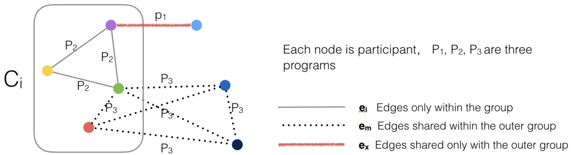
Fig. 4.18 Three different types of contacts between members.
