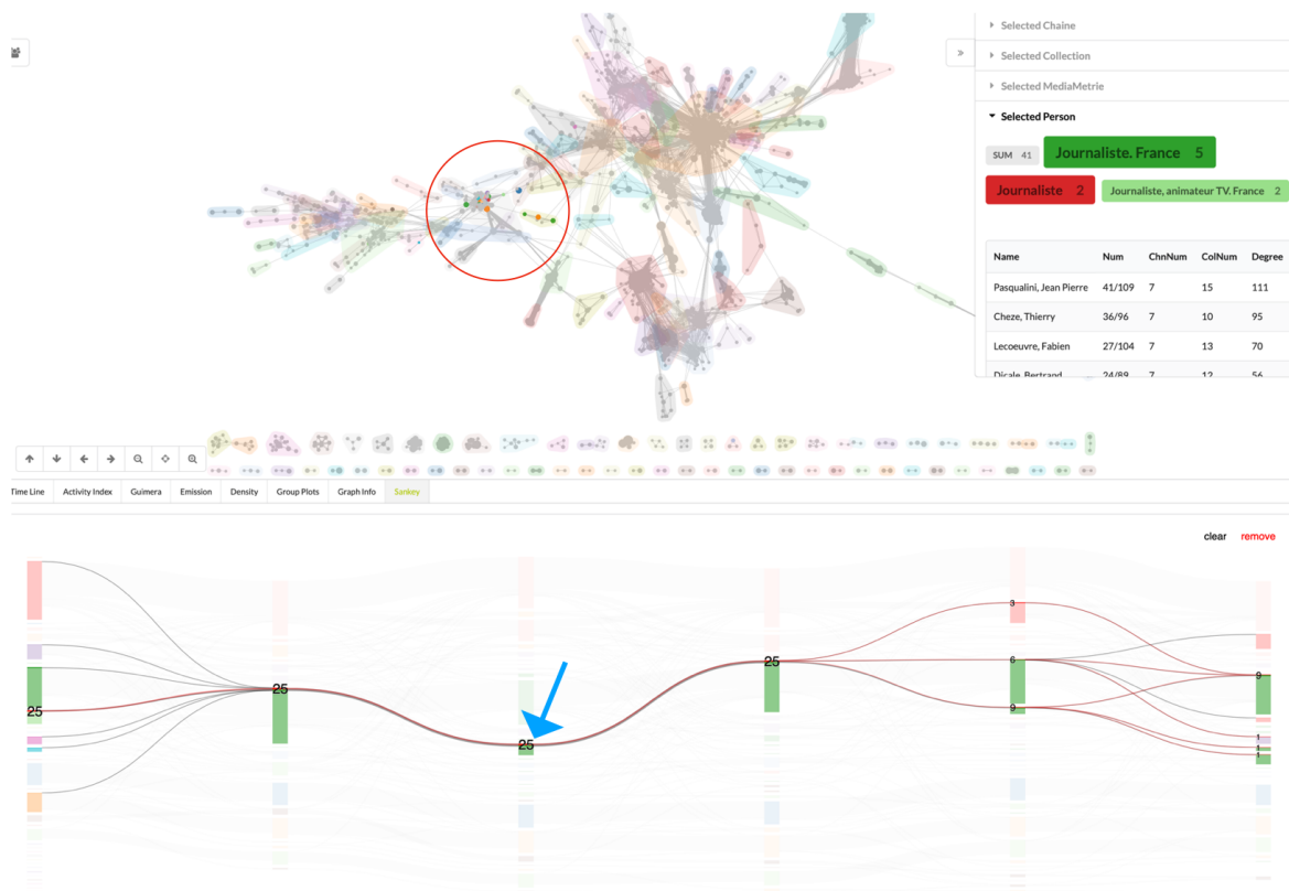
Fig. 4.32 The mouseover interaction is also available on the sankey graph.
