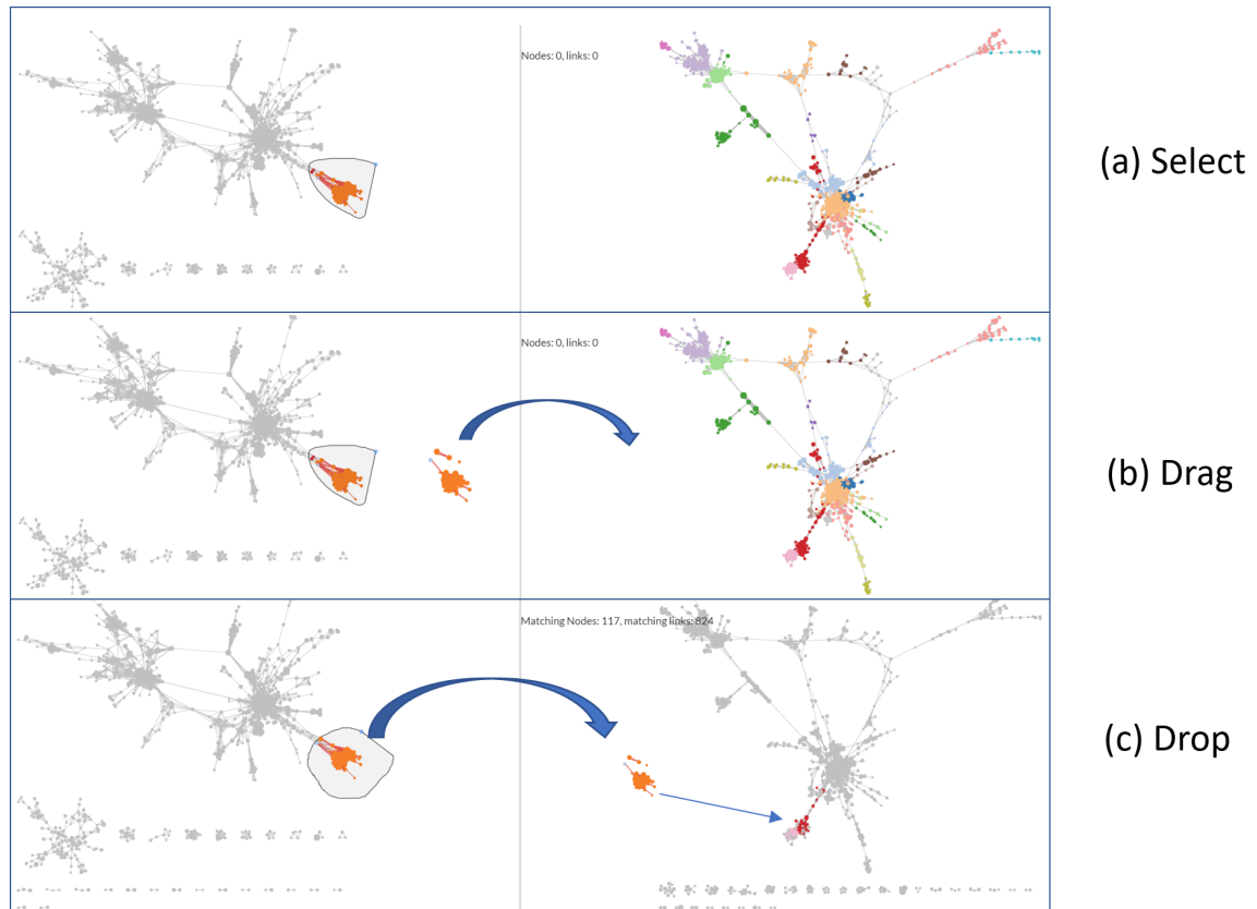
Fig. 4.27 The process of drag-drop interaction. User select a subgraph from left view, then drag the selected subgraph to the right view, then drop the subgraph, the same nodes and links will gradually move to the matching location and then be highlighted.
