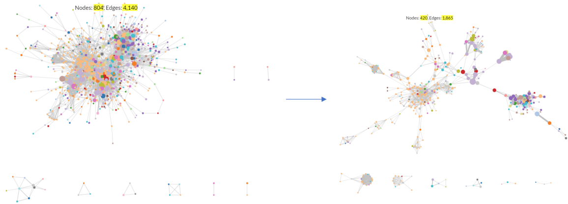
Fig. 4.39 Network built from debat programs, left is the original graph, right is the filtered graph build from using Semmilian backbone method.
