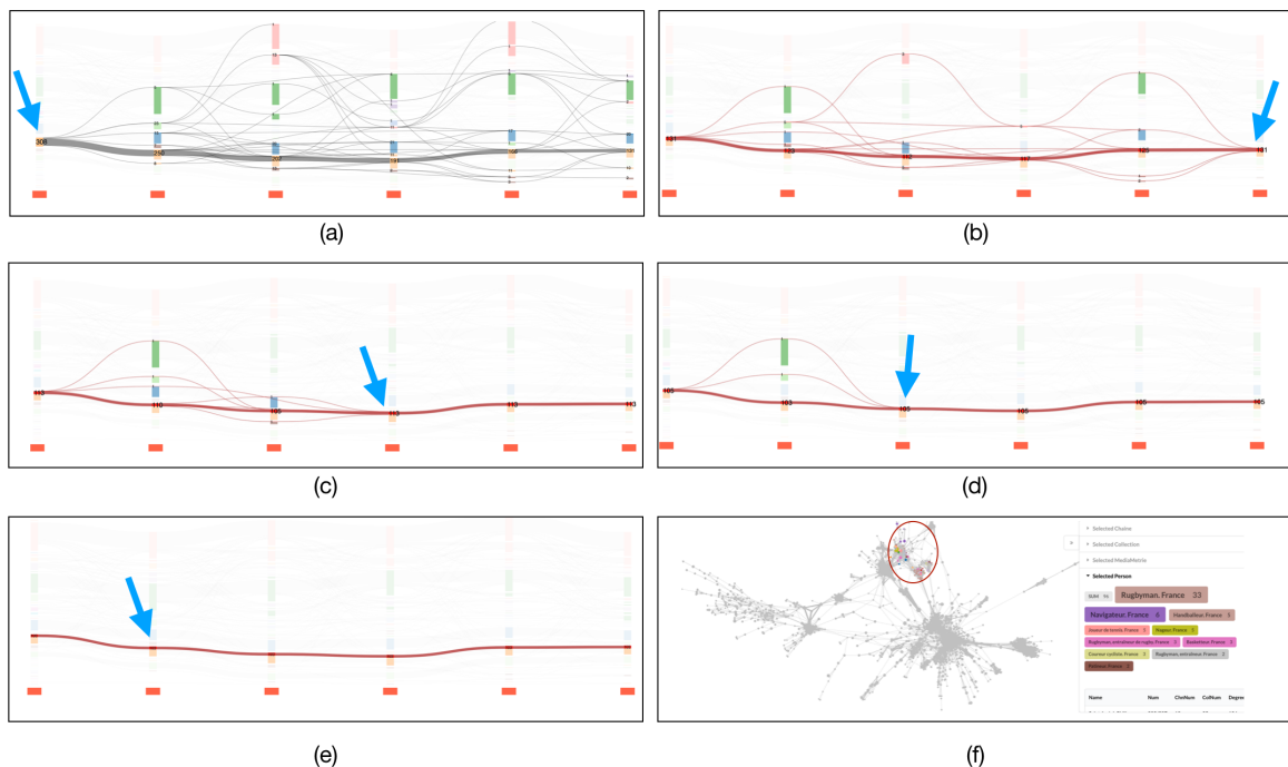
Fig. 4.30 When the user clicks on a band or a link, a subsankey consisting only of the members that are clicked is displayed, and this step can be repeated to narrow the scope.
