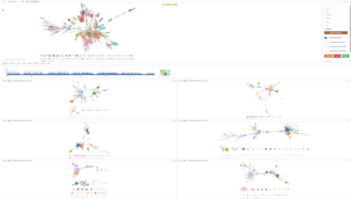
Fig. 4.25 Screenshot of our framework, multiple views of graphs are shown at the same time.
