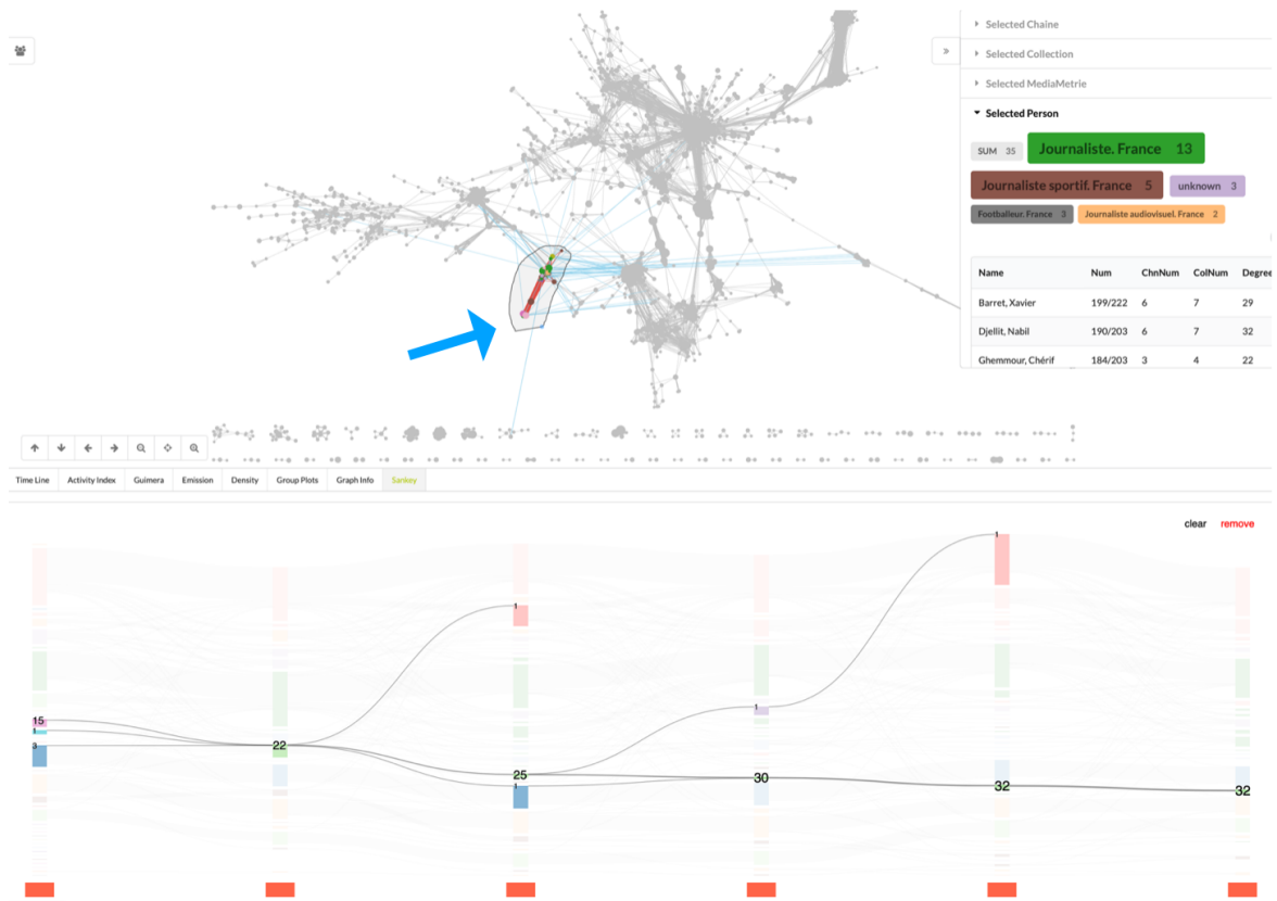
Fig. 4.33 Select a community from node-link graph, the sankey graph display how the communiti's evolution.
