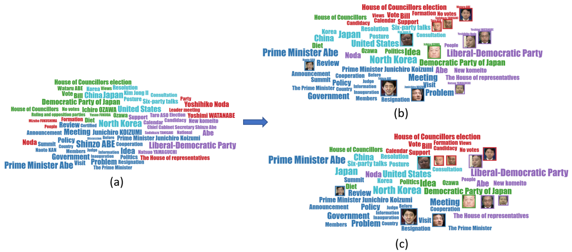
Fig. 3.11 Since the position occupied by the tags is a rectangle and the character image is also a rectangle, we use the character image instead of the tags in the process of calculating the layout, so that the tags and the image can appear at the same time, and the hierarchical placement is kept. (a) displays the normal tagcloud, we use the person’s name instead of their profile photo, (b) displays the profile photo and the name at the same time, (c) displays only profile photo
