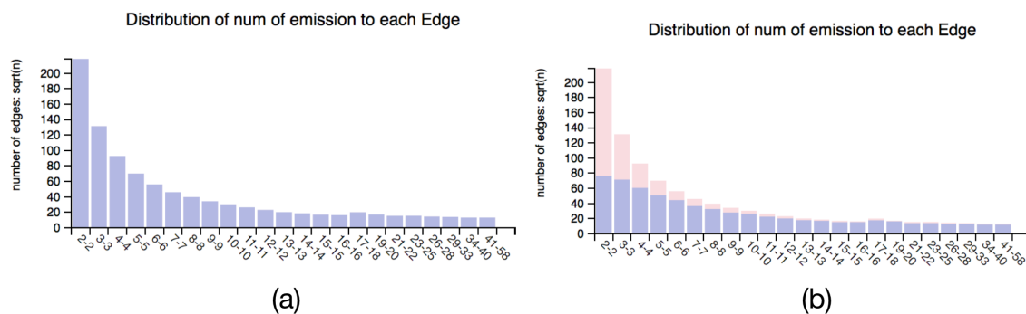
Fig. 4.37 The non-uniform division histogram shows the distribution of number of edges in different number of programs number interval
