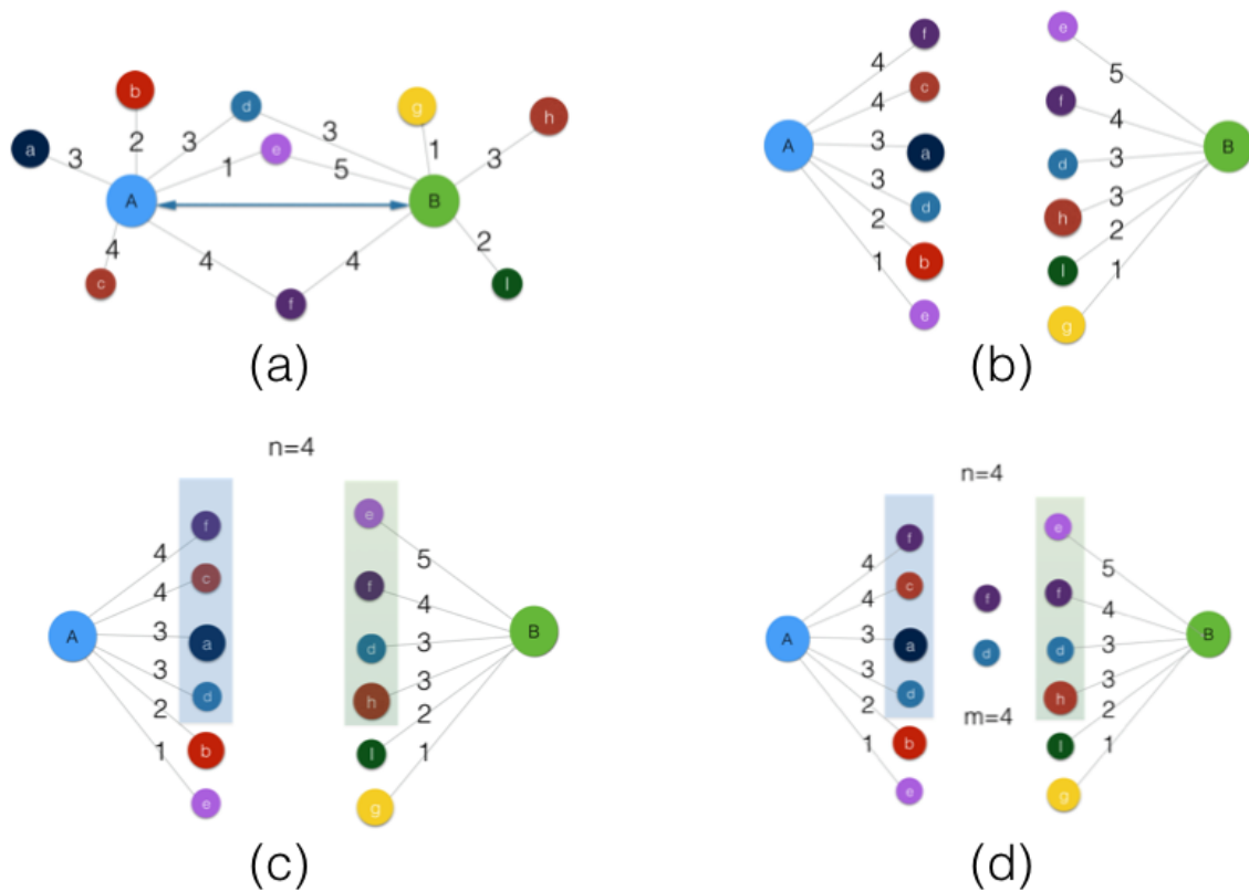
Fig. 5.1 Process of Simmelian backbone
