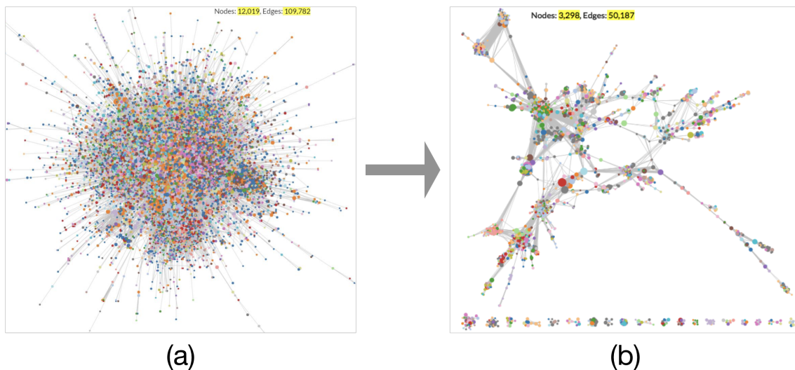
Fig. 4.11 (a) co-participation network built from 'Magazine' programs; (b) filtered network from (a) using Simmelian backbone.
