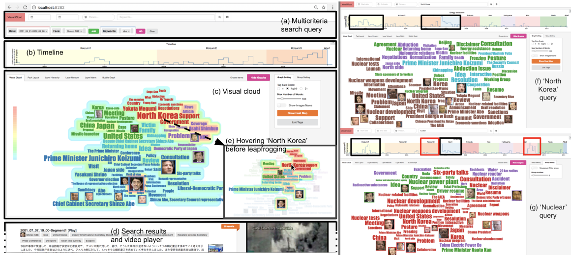
Fig. 3.14 Left. Interface overview, search query over Abe during Koizumi terms (a) - very active during the end of Koizumi3 (b), mention of ‘North Korea’ stands out (c). Hovering over ‘North Korea’ shows that it strongly relates to ‘abduction’ (e). Right. Comparison of the queries on North Korea (f), and Nuclear (g): two periods coincide (in black) Koizumi1 and Abe1 but we can notice two major differences (in red). Koizumi3 period did not associate much North Korea and Nuclear , and Kan period associate Nuclear with Accident . Demonstration video available at https://youtu.be/VfGwa6T94t8 .
