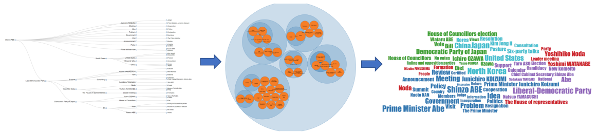
Fig. 3.10 Dendrogram is used to build pack layout, the location of the tag in the tag cloud depends on the location of the tags in the pack layout.
