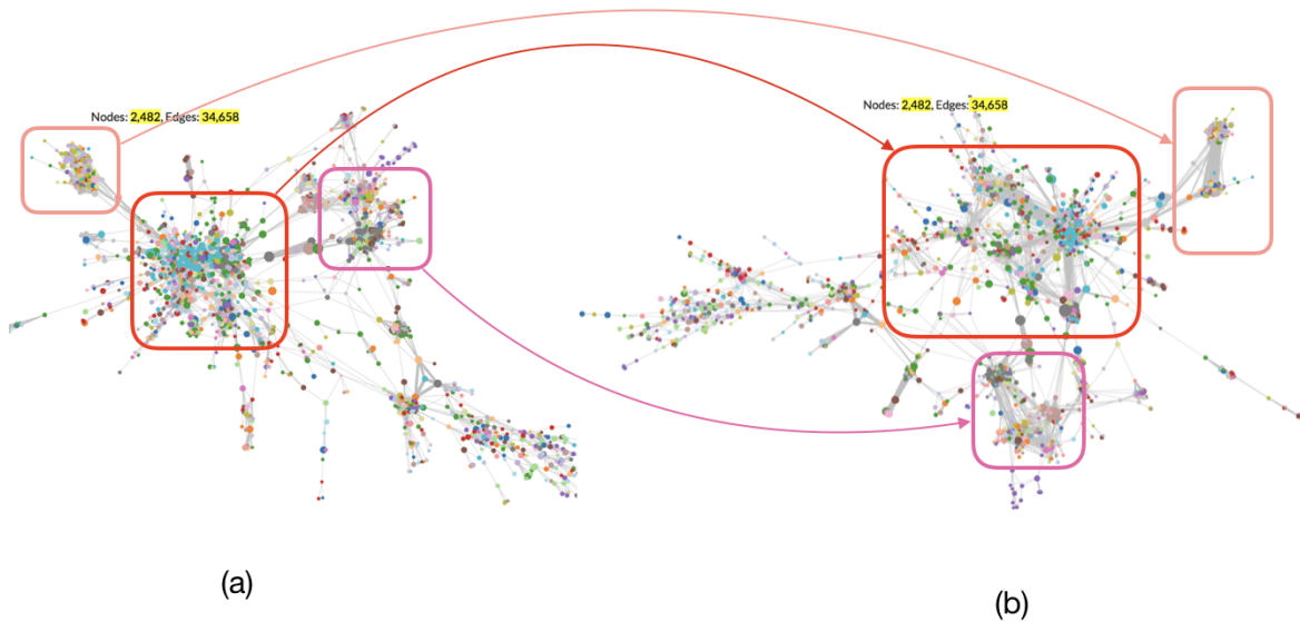
Fig. 4.14 The comparison between (a) and (b) shows the difference between before and after the layout algorithm is modified. (a) is the force layout not be modified, The middle part is very dense. It can be clearly seen in the (b) that the dense portion of the pattern is dispersed.
