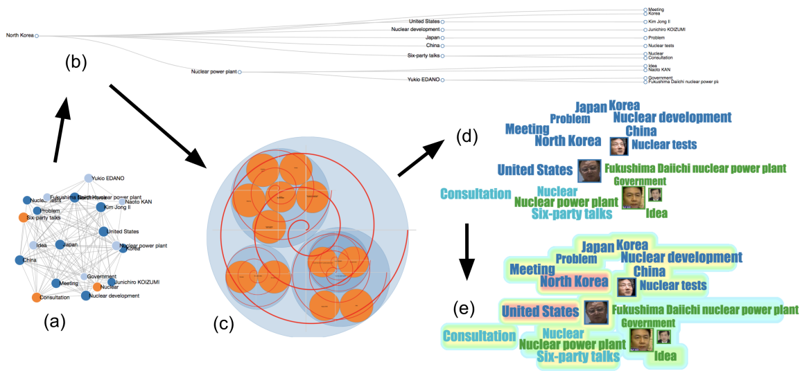
Fig. 3.9 Visual cloud layout: (a) LIN (b) extracted hierarchy (c) Pack Layout embedding (with spirals) (d) visual cloud (e) with heatmap.
