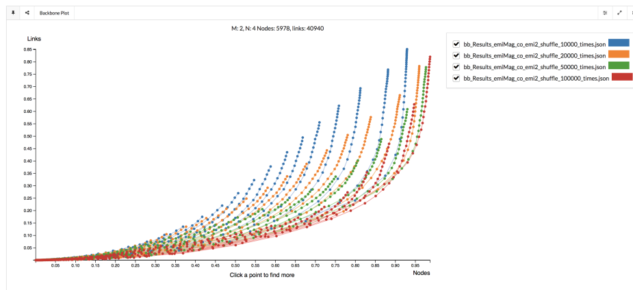
Fig. 5.12 Connect all the dots with same M value
