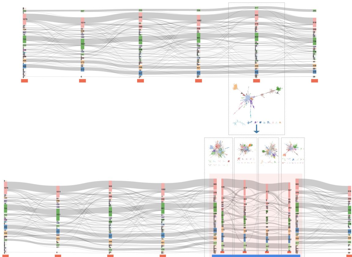
Fig. 4.29 Zoomable sankey, The user can select a time period and then continue to subdivide the graph during this time period.
