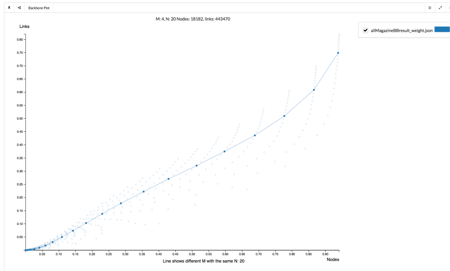
Fig. 5.4 Dots with same n = 20 are connected in turn
