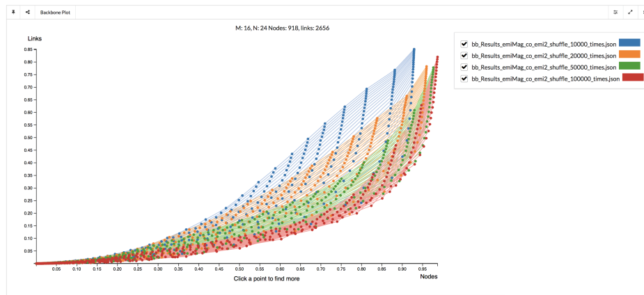
Fig. 5.11 Connect all the dots with same N value
