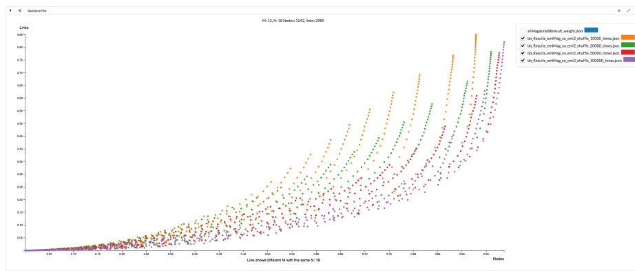
Fig. 5.8 Compare the results of the network in Simmelian after different random processes
