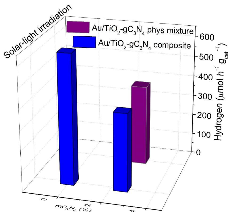
Figure 4.23. Mean hydrogen formation rate per hour and per mass with 1 vol% TEOA of Au/TiO 2 -gC 3 N 4 (97.5-2.5) zoom composite and one reference. Additionally, the physical mixture equivalent to the zoom proportion composition was added for comparison.
