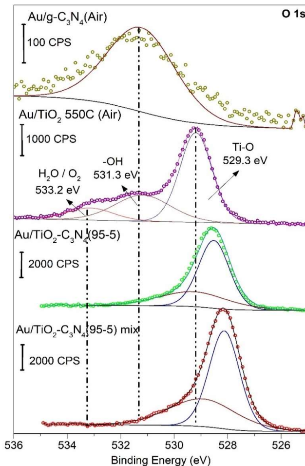
Figure 3.44. XPS O 1s spectra of the \text{Au/TiO}_2\text{-gC}_3\text{N}_4\text{-(95-5)-Air} and three references \text{Au/TiO}_2\text{-gC}_3\text{N}_4\text{-(95-5)} physical mixture, \text{Au/TiO}_2 550 °C, and \text{Au/g-C}_3\text{N}_4 (Air).
