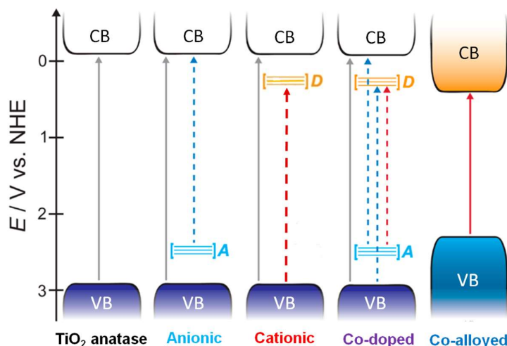
Figure 1.21. Density of states scheme of \text{TiO}_2 energy bands for the different doping types. Orange represents several energy states on the CB, blue represents several energy states on the VB, A stands for orbital p of the anion, and D stands for the metal [158].
