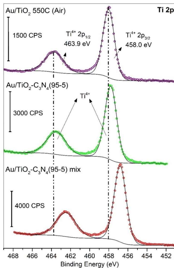
Figure 3.40. XPS Ti 2p spectra of the \text{Au/TiO}_2\text{-gC}_3\text{N}_4 -(95-5) composite \text{Au/TiO}_2\text{-gC}_3\text{N}_4 -(95-5) physical mixture and \text{Au/TiO}_2 550 °C (Air) reference.
