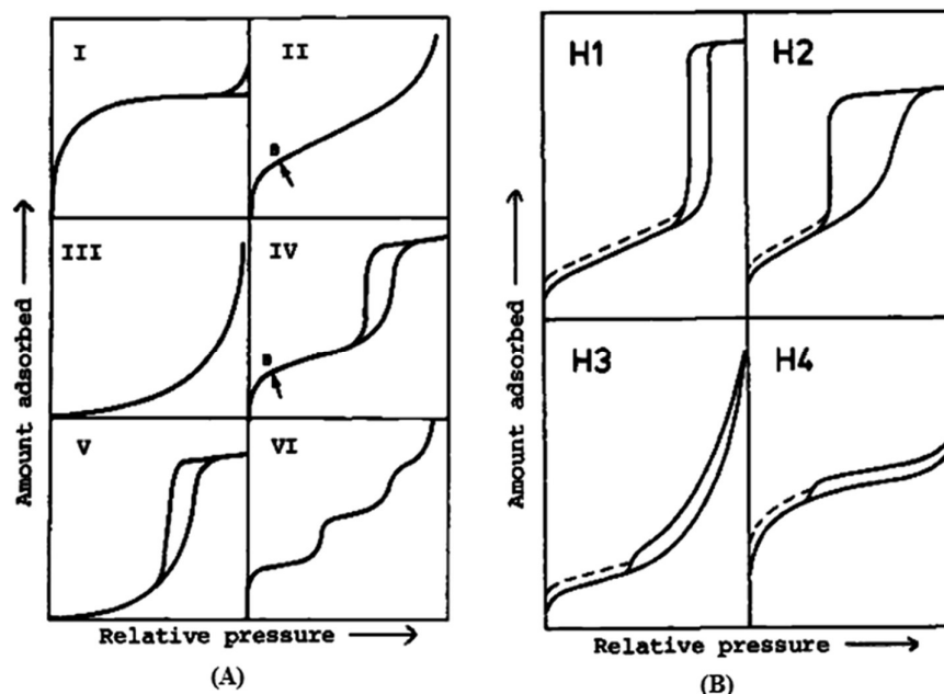
Figure A.7. A) 6 types of isotherms of adsorption-desorption B) 4 types of histeres loops.
