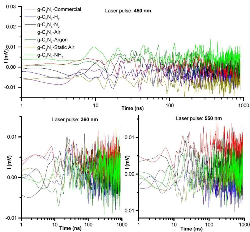
Figure 2.12. TRMC measurements of the references and of the as-prepared g\text{-C}_3\text{N}_4 -atm samples at 360, 450, and 550 nm.
