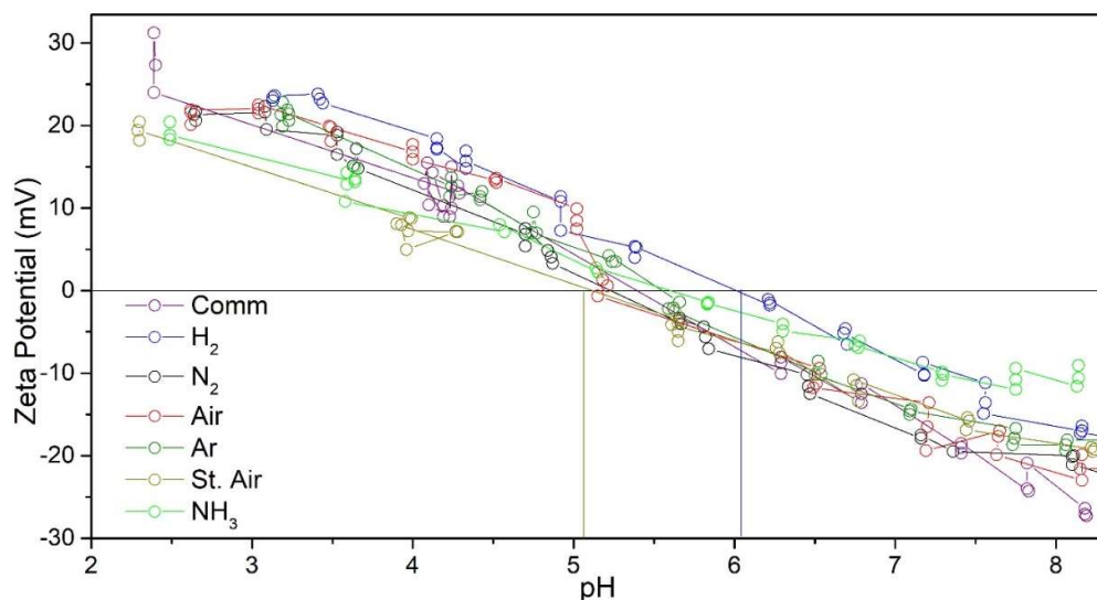
Figure 2.11. Auto-titration of the references and of the as-prepared g\text{-C}_3\text{N}_4 -atm samples to obtain the IEP.
