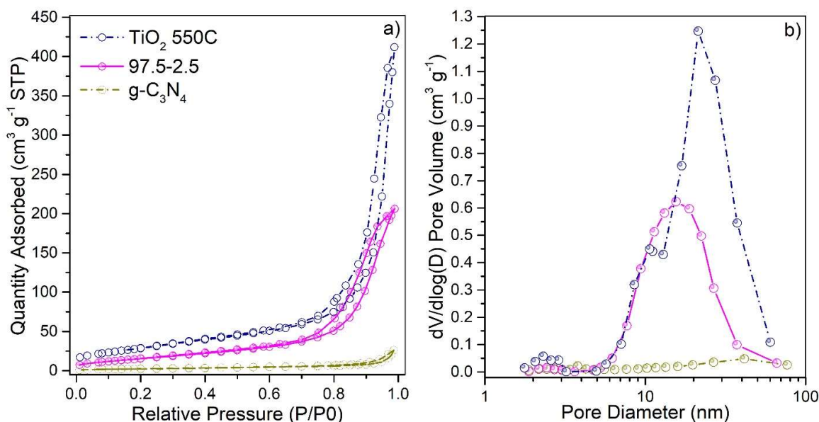
Figure 4.13. a) Nitrogen adsorption-desorption isotherms b) BJH pore-size distribution of the TiO 2 -gC 3 N 4 (97.5-2.5) zoom composite and references.
