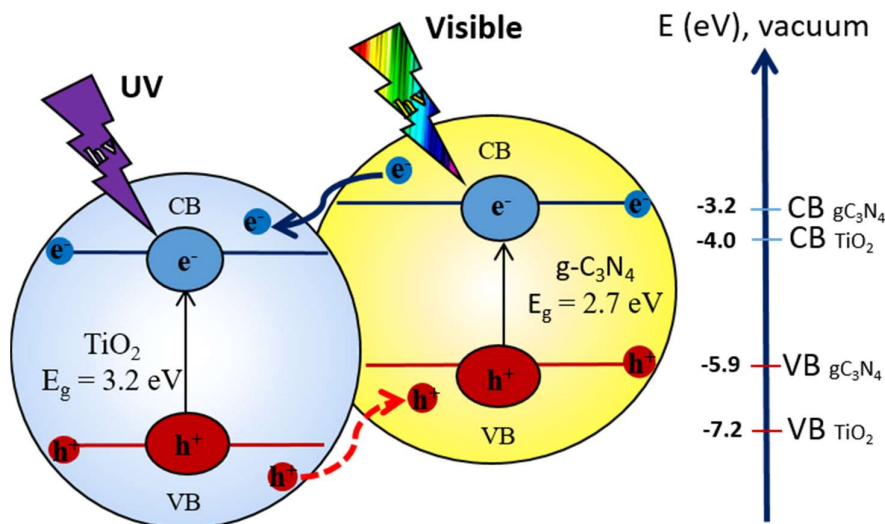
Figure 1.20. TiO 2 coupled with g-C 3 N 4 in a heterojunction type II (staggered type). The photo-sensitization mechanism, under visible-light irradiation is shown. Also, the possibility of transferring h^+ from TiO 2 (VB) to g-C 3 N 4 (VB).
