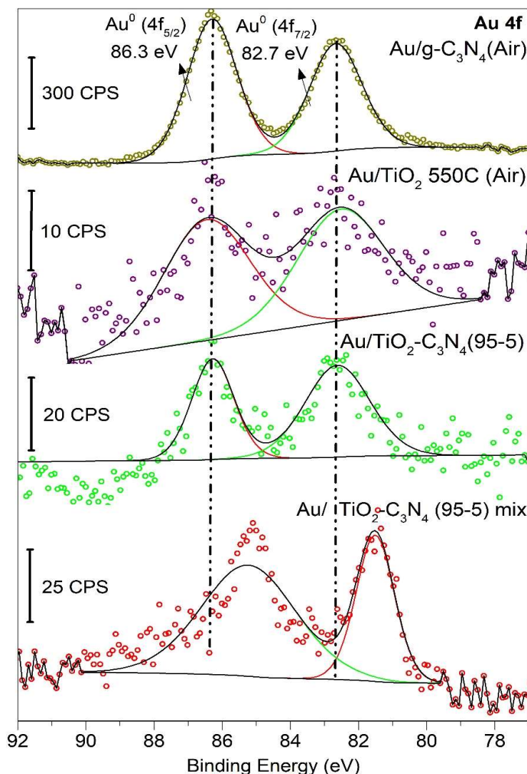
Figure 3.43. XPS Au 4f spectra of the \text{Au/TiO}_2\text{-gC}_3\text{N}_4\text{-(95-5)-Air} composite, \text{Au/TiO}_2\text{-gC}_3\text{N}_4\text{-(95-5)} physical mixture, \text{Au/TiO}_2 550 °C (Air), and \text{Au/g-C}_3\text{N}_4 (Air) three references.
