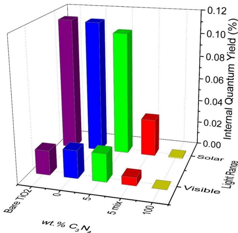
Figure 3.36. Internal quantum yield (IQY, %) of the \text{Au/TiO}_2\text{-gC}_3\text{N}_4 (95/5) composite, three references, and physical mixture with the same massic ratio under solar and visible-light irradiation.
