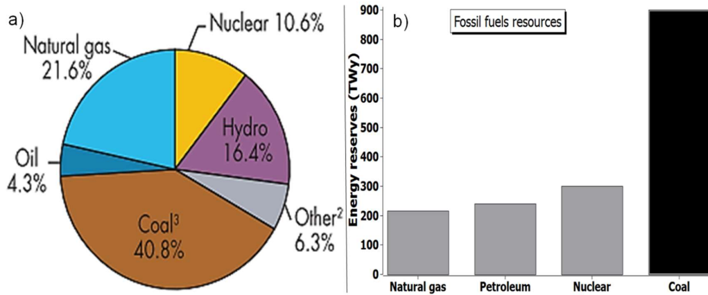
Figure 1.2. a) Distribution of world energy sources for the energy supply. b) World energy reserves amount of the fossil fuels [1,13].
