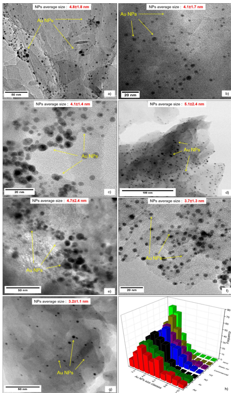
Figure 2.16. TEM images for the Au/g-C 3 N 4 -atm composites, including the mean particles size with their standard deviation, a) Au/g-C 3 N 4 -Commercial b) Au/g-C 3 N 4 -H 2 c) Au/g-C 3 N 4 -N 2 d) Au/g-C 3 N 4 -Air e) Au/g-C 3 N 4 -Ar f) Au/g-C 3 N 4 -Static Air g) Au/g-C 3 N 4 -NH 3 h) Au NPs size distribution determined from TEM characterization of Au/g-C 3 N 4 -atm samples (obtained from a selection of 200 Au NPs for each sample).
