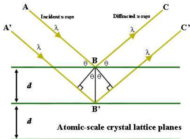
Figure A. 5. X-ray Diffraction principle (mode 2\theta ).
