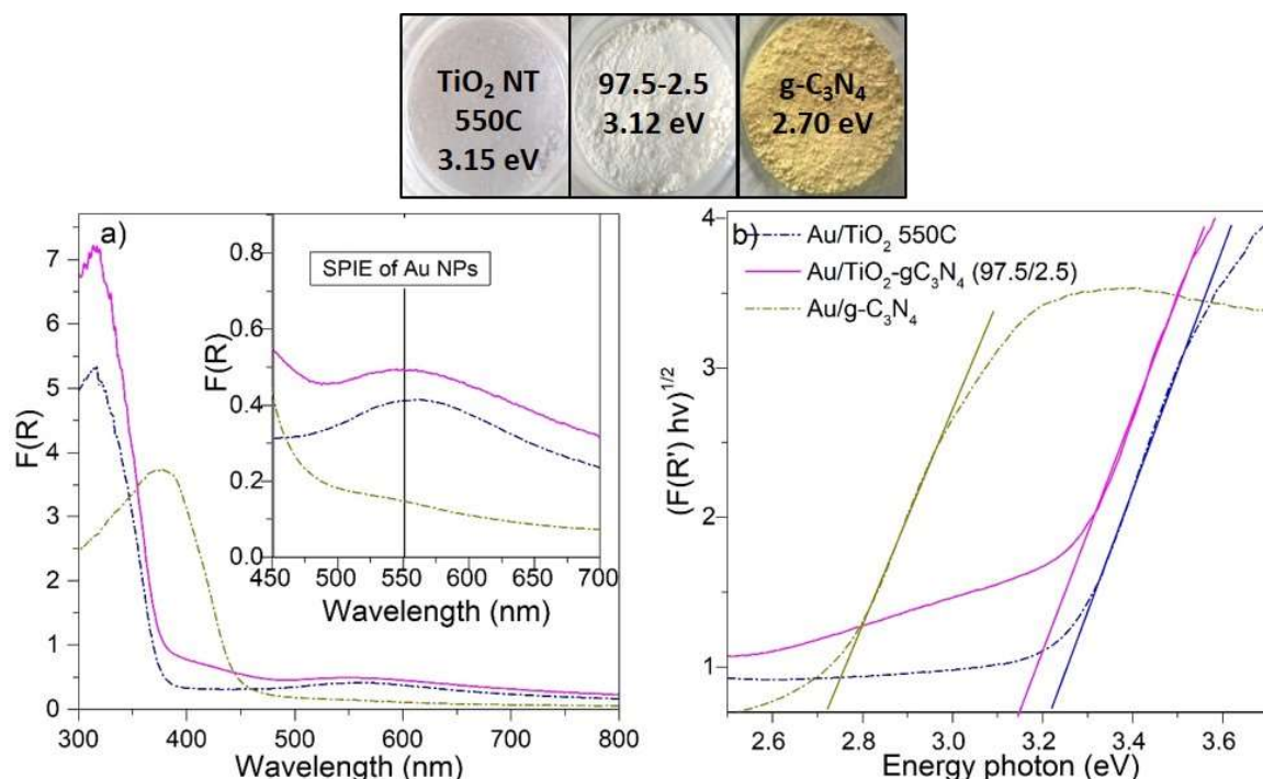
Figure 4.18. a) UV-Vis spectra of Au/TiO 2 -gC 3 N 4 (97.5-2.5) zoom composites and references Inset) zoom of the spectral domain corresponding to SPIE signal of Au NPS at approximately 550 nm b) Tauc plot to determine the apparent band gap of Au/TiO 2 -g-C 3 N 4 zoom composites.
