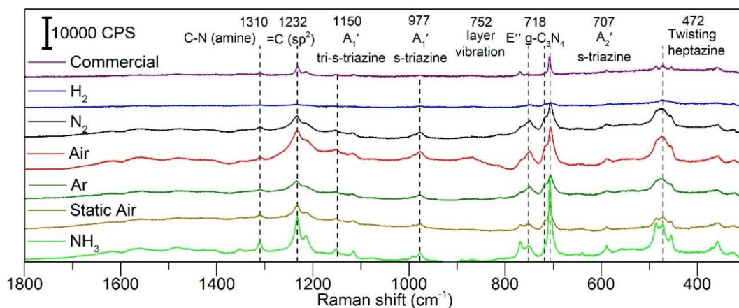
Figure 2.4. Background corrected Raman spectra of the as-prepared g-C 3 N 4 -atm samples.
