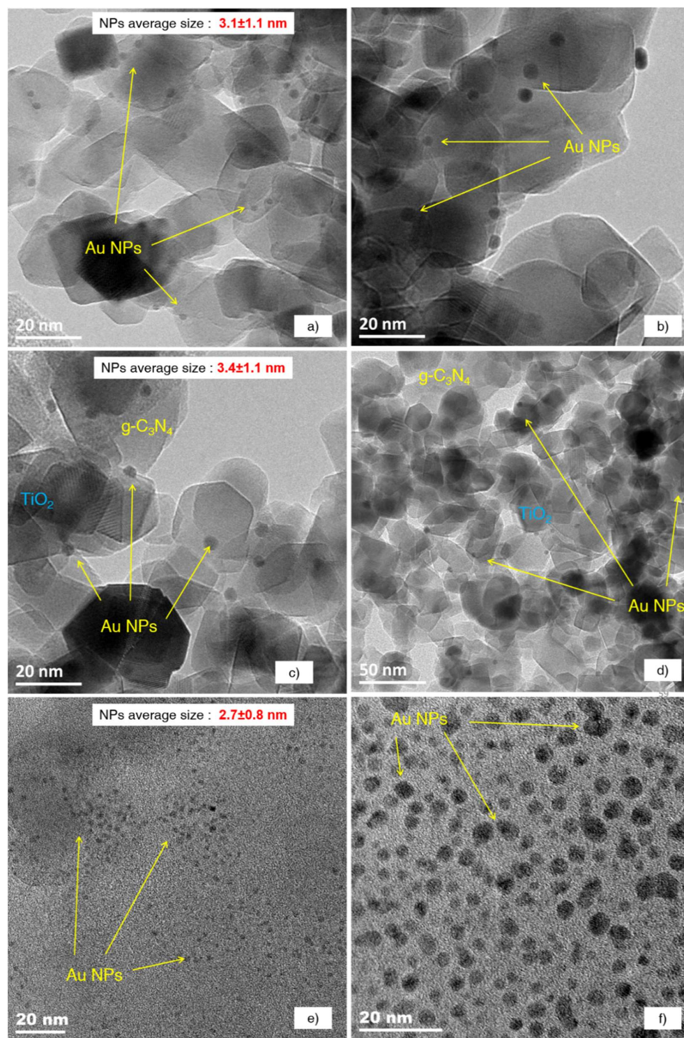
Figure 3.19. TEM images for Au/ TiO 2 -gC 3 N 4 -Air screening composite and references, including the mean particle size with their corresponding standard deviation, a, b) 0.3 wt. % Au/Bare TiO 2 (P25), c, d) 0.3 wt. % Au/TiO 2 550 °C Air, e, f) 0.3 wt. % Au/ TiO 2 -gC 3 N 4 (30-70).
