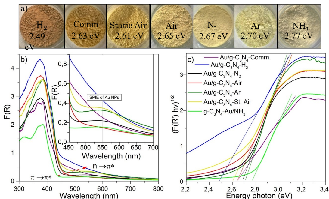
Figure 2.18. a) Color of the powders of the bare g-C 3 N 4 samples b) UV-Vis spectra of the Au/g-C 3 N 4 -atm composites. Inset) zoom of the spectral domain corresponding to SPIE signal of Au NPS at ca. 550 nm. c) Tauc plot to determine the apparent band gap of Au g-C 3 N 4 -atm composites.
