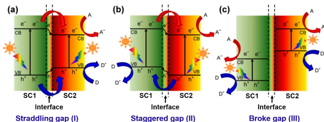
Figure 1.15. General three types of heterojunctions between two semiconductors with different band gaps and band edges positions [94,95].
