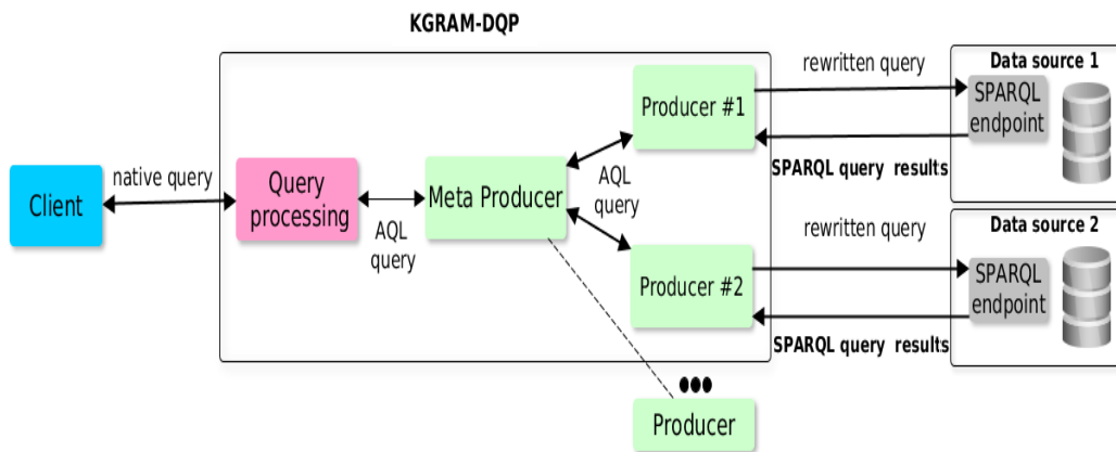
Figure. 6.1: KGRAM-DQP architecture
