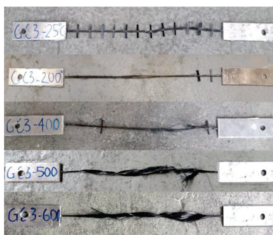
(c) Textile de carbone GC3
