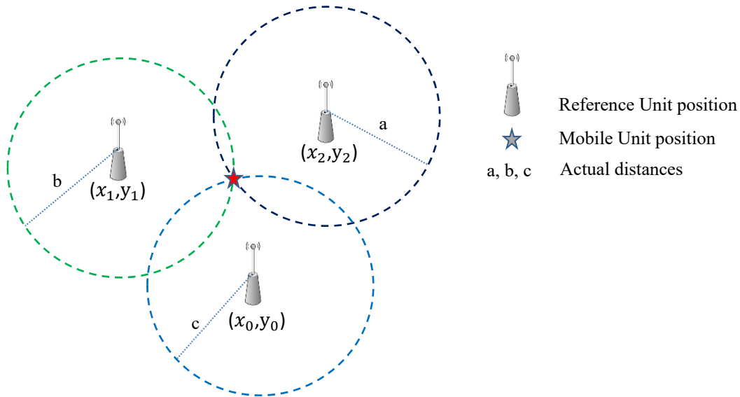
Figure 1-5: Time of arrival (ToA)-based approach.
