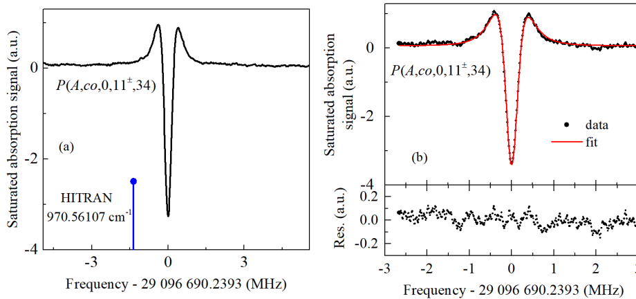
Figure F.2 – (a) Saturated absorption spectrum of the P(A, co, 0, 11^\pm, 34) K -doublet around 970.516 \text{ cm}^{-1} recorded using frequency modulation and second-harmonic detection. Experimental conditions: pressure, \sim 1.7 \text{ Pa} ; intra-cell average laser power, \sim 0.78 \text{ mW} ; modulation frequency, 20 kHz; frequency modulation excursion, 150 kHz; frequency step, \sim 15 \text{ kHz} ; average of five pairs of up and down scans; total integration time per point, 1 s; whole spectrum measurement time, 701 s. The P(A, co, 0, 11^\pm, 34) degenerate (indicated by \times 2 ) doublet position reported in the HITRAN database [54] is also shown as a blue stick. (b) One averaged pair of up and down scans contributing to the data of panel (a), the resulting fit to the data, and its residuals. The total integration time per point is 200 ms, whole spectrum measurement time: 77 s.
