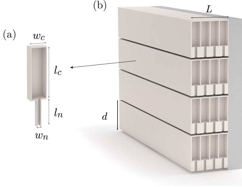
FIGURE 2.1: (a) Square cross-section Helmholtz resonator (HRs). (b) Conceptual view of the metamaterial panel placed on a rigid wall with N = 4 layers of HRs.
