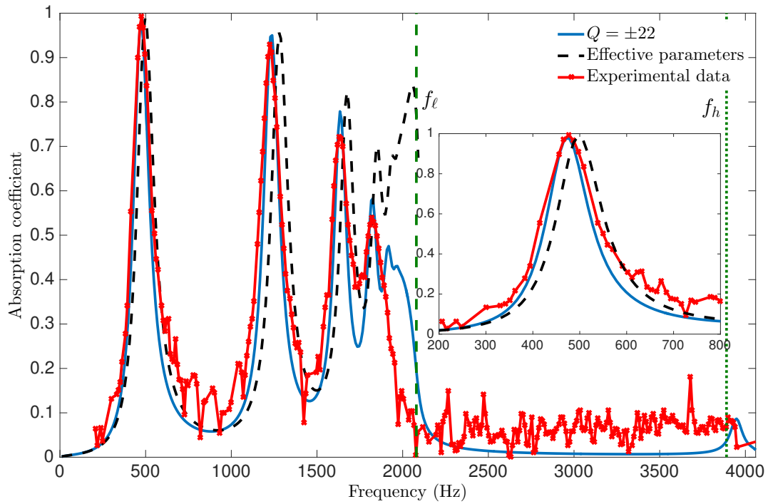
FIGURE 1.11: Absorption coefficients: Sample 2 measured and simulated with the full model and with the effective parameters ( f_l and f_h in green).
