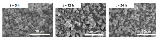
Fig. 3. PXRD crystallinity patterns and SEM morphology images of \gamma -CD-MOF crystals obtained after different reaction times of 6 h (F1), 12 h (F6) and 24 h (F7). The longer reaction time of 24 h showed the destruction of the crystalline structure of \gamma -CD-MOFs and resulted in a smaller size.
