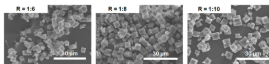
Fig. 4. PXRD crystallinity patterns and SEM morphology images of \gamma -CD-MOF crystals obtained with different ratios of \gamma -CD to KOH as 1:6 (F8), 1:8 (F1) and 1:10 (F9). Higher ratios of \gamma -CD to KOH showed no influence on the crystalline structure of \gamma -CD-MOFs and resulted in a smaller size.
