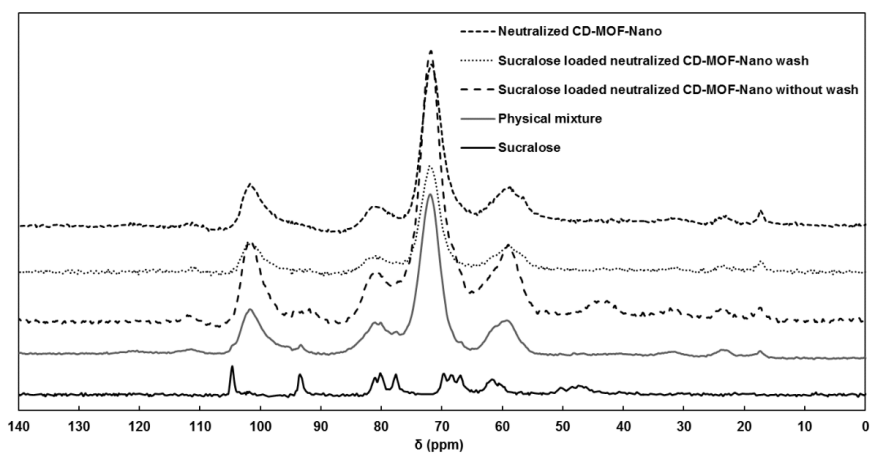
Figure S4. 13 C MAS NMR spectra of sucralose, neutralized CD-MOF-Nano, sucralose loaded CD-MOF-Nano with wash, sucralose loaded neutralized CD-MOF-Nano without wash and physical mixture of sucralose with neutralized CD-MOF-Nano.
