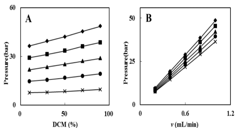
56 57 Fig. S1 Dependence of \gamma -CD-MOF packed column pressure on the flow rate and mobile phase 58 composition. (A) The different flow rate. (x: 0.2 mL/min, ●: 0.4 mL/min, ▲: 0.6 mL/min, ■: 0.8 59 mL/min, ◆: 1.0 mL/min), (B) The contents of DCM in the mobile phase. (x: 10%, ●: 30%, ▲: 60 50%, ■: 70%, ◆: 90%).
