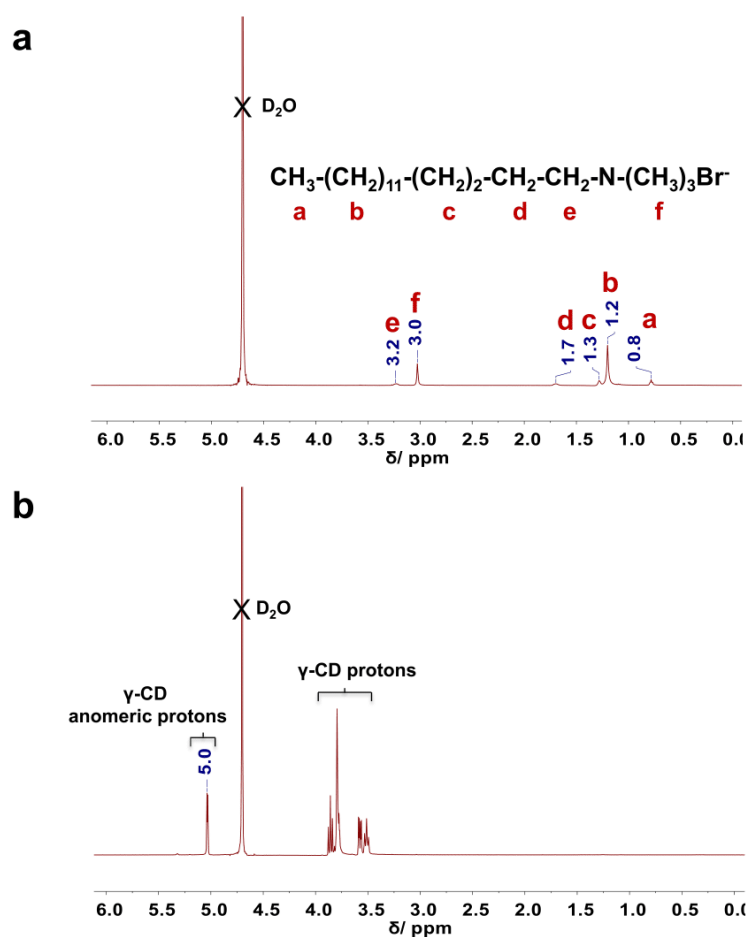
9 10 Fig. S1 1 H NMR spectrum (500 MHz) in D 2 O of a) CTAB (5 mg·mL -1 ) and b) redissolved 11 CD-MOF nanocrystals prepared from potassium hydroxide and γ-CD (10 mg·mL -1 ), 12 referenced to the H 2 O peak (δ = 4.79 ppm).
