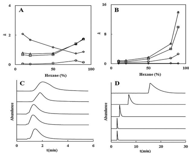
Fig. 3. The retention factors of the m -xylene, ketoprofen, fenbufen and diazepam at different mobile phase compositions in (A) \gamma -CD-MOF column and (B) the \gamma -CD column. (□: ketoprofen, △: fenbufen, ○: diazepam, ◇: m -xylene, error bars in these plots represented a range of \pm SD for duplicate injection); effect of the mobile phase on the ketoprofen HPLC chromatograms in the (C) \gamma -CD-MOF column and (D) \gamma -CD column, from top to bottom, the ratio of hexane were 90%, 80%, 50%, 20% and 10%.
