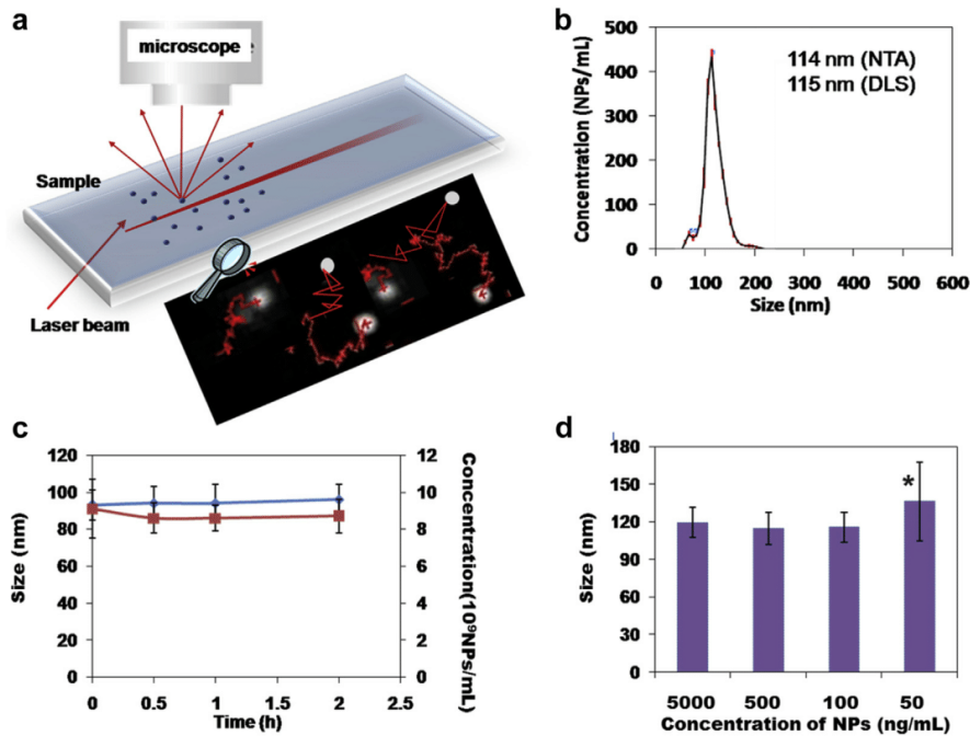
Figure 5. Poly-CD/Dex-Bz NP stability upon dilution determined by NTA analysis. (a) Schematic representation of the NTA measurements of NP diameters. (b) Typical size distribution results obtained by NTA in the case of poly-CD/Dex-Bz NPs obtained by mixing equal volumes of polymer solutions at concentration of 1.0 mg/mL. (c) Mean hydrodynamic diameters (blue) and concentration (red) of poly-CD/Dex-Bz NPs (5 \mu\text{g/mL} ) after their formation and during storage at room temperature. (d) Mean hydrodynamic diameters of poly-CD/Dex-Bz NPs prepared at a polymer concentration of 1 mg/mL and further diluted to reach the final concentration of 5-0.05 \mu\text{g/mL} . The asterisk in (d) is referred to the presence of polydisperse NPs at the highest dilutions (final concentrations of 50 ng/mL). The error bars in (c) and (d) are from the standard deviation values.
