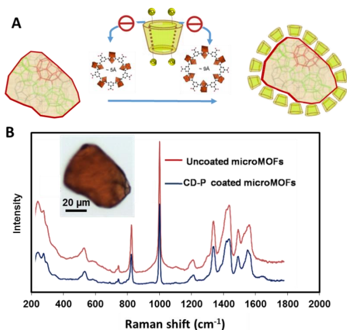
Fig.7 Raman spectra of individual MIL-100(Fe) MOF particles, coated or not with P-CD. Schematic representation of the coating procedure (A) and experimental results (B) for MOF particles before and after CD-P coating.
