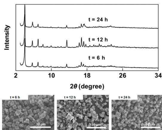
Fig. 3. PXRD crystallinity patterns and SEM morphology images of \gamma -CD-MOF crystals obtained after different reaction times of 6 h (F1), 12 h (F6) and 24 h (F7). The longer reaction time of 24 h showed the destruction of the crystalline structure of \gamma -CD-MOFs and resulted in a smaller size.
