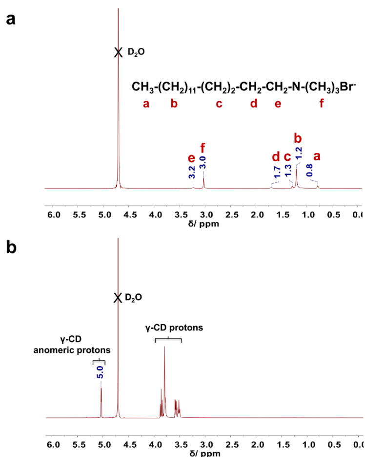
9 10 Fig. S1 1 H NMR spectrum (500 MHz) in D 2 O of a) CTAB (5 mg·mL -1 ) and b) redissolved 11 CD-MOF nanocrystals prepared from potassium hydroxide and γ-CD (10 mg·mL -1 ), 12 referenced to the H 2 O peak (δ = 4.79 ppm).
