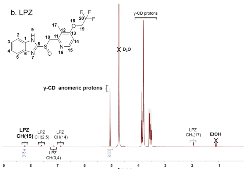
1 2 Fig. S4 ^1\text{H} NMR spectrum (500 MHz) in \text{D}_2\text{O} of drug-loaded CD-MOF nanocrystals 3 prepared by co-crystallisation ( 10 \text{ mg}\cdot\text{mL}^{-1} ). a) IBU and b) LPZ.
