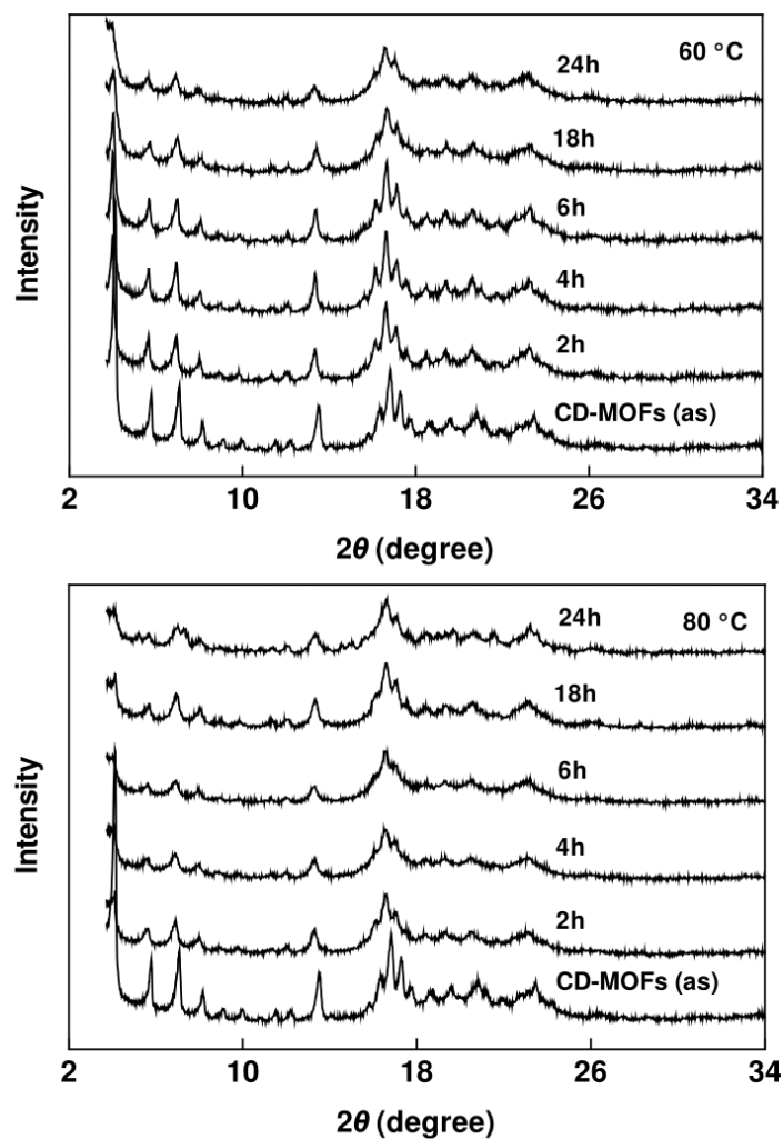
Figure S5. PXRD patterns of \gamma -CD-MOFs (as: as-synthesized) at 60, 80 °C after different time
