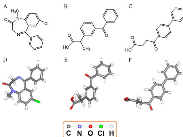
Fig. 1. The 2D and 3D images of the drug analytes. (A) 2D structure of diazepam, (B) 2D structure of ketoprofen, (C) 2D structure of fenbufen, (D) 3D structure of diazepam, (E) 3D structure of ketoprofen, (F) 3D structure of fenbufen.
