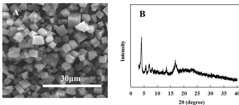
94 95 Fig. S3 The characterization of \gamma -CD-MOF during the column preparation, (A) the SEM image. 96 and (B) the powder-XRD image.
