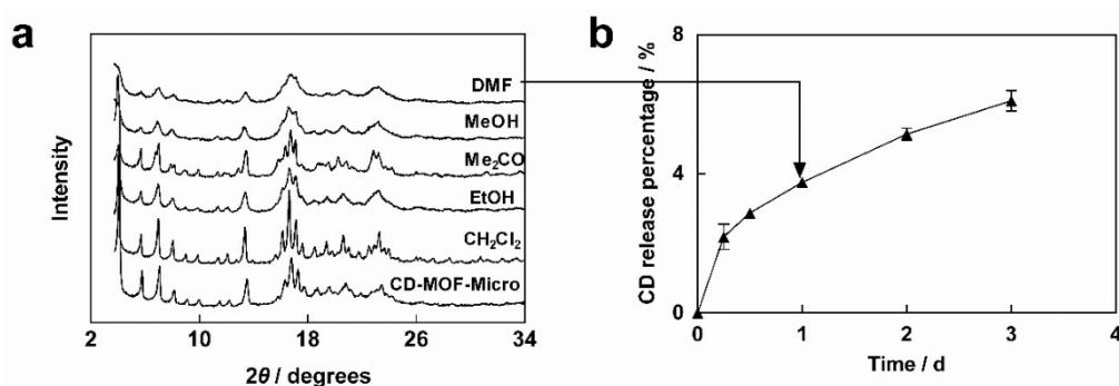
10 11 Fig. S2 a) PXRD Pattern of CD-MOF microcrystals incubated in different solvents at 70 12 °C for one day. b) The CD release profile for the incubation in DMF at 70 °C for three 13 days. Error bars are based on repeating experiments on three batches of crystals.
