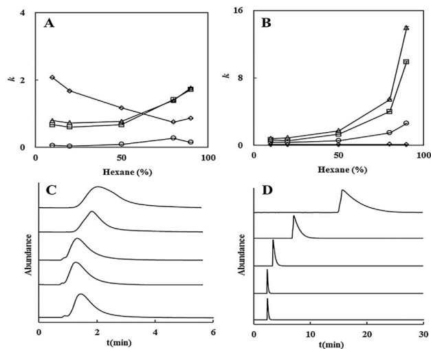
Fig. 3. The retention factors of the m -xylene, ketoprofen, fenbufen and diazepam at different mobile phase compositions in (A) \gamma -CD-MOF column and (B) the \gamma -CD column. (□: ketoprofen, Δ: fenbufen, ○: diazepam, ◇: m -xylene, error bars in these plots represented a range of \pm SD for duplicate injection); effect of the mobile phase on the ketoprofen HPLC chromatograms in the (C) \gamma -CD-MOF column and (D) \gamma -CD column, from top to bottom, the ratio of hexane were 90%, 80%, 50%, 20% and 10%.
