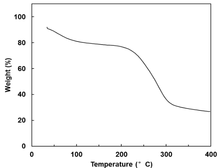
Figure S4. Thermogravimetric analysis of \gamma -CD-MOFs
