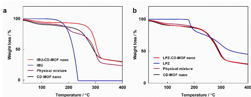
5 6 Fig. S7 TGA traces of drug-loaded CD-MOF nanocrystals prepared by the co- 7 crystallisation. a) IBU. b) LPZ.
