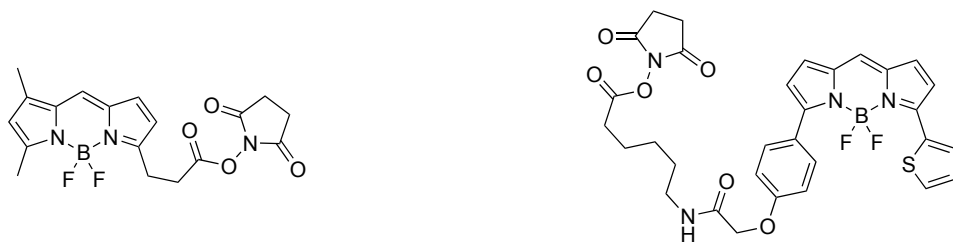
BODIPY ® FL – ester succinimidyle
