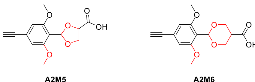
Figure 20. New cyclic acetal linker models A2M5 and A2M6 .
